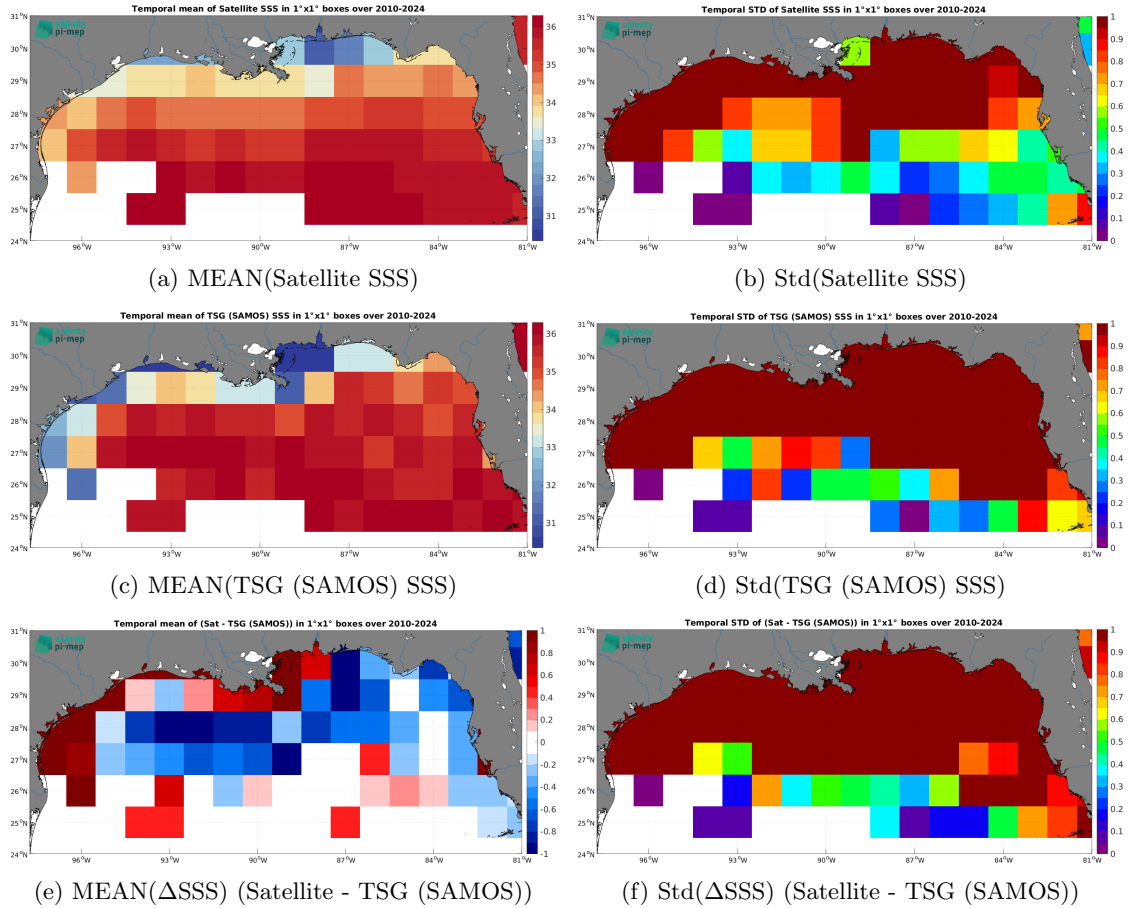
Figure 7: Temporal mean (left) and Std (right) of SSS from SMOS SSS L4 v1 - Monthly (CMEMS-CNR) (top), TSG (SAMOS) (middle), and of \Delta\text{SSS} (Satellite - TSG (SAMOS)). Only match-up pairs are used to generate these maps.
