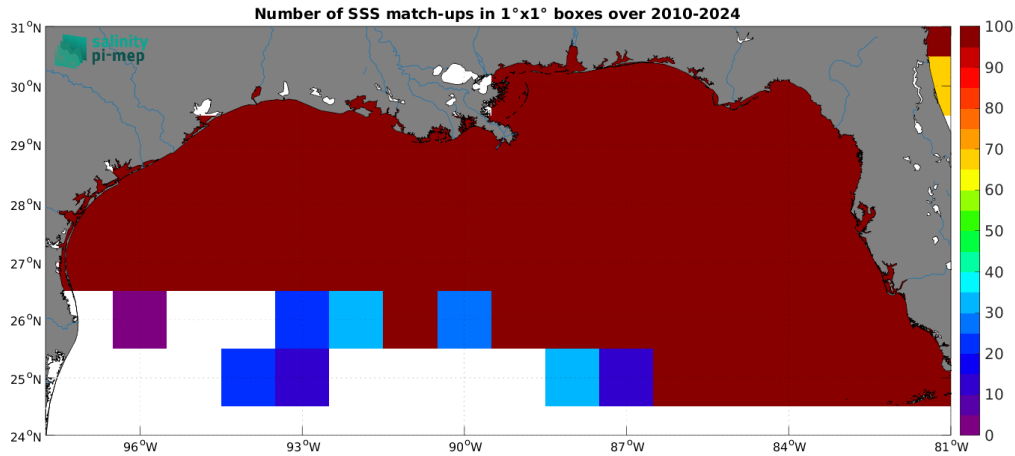
Figure 5: Number of SSS match-ups between TSG (SAMOS) SSS and the SMOS SSS L4 v1 - Monthly (CMEMS-CNR) SSS product for the Mississippi river plume Pi-MEP region over 1^\circ \times 1^\circ boxes and for the full satellite product period.
