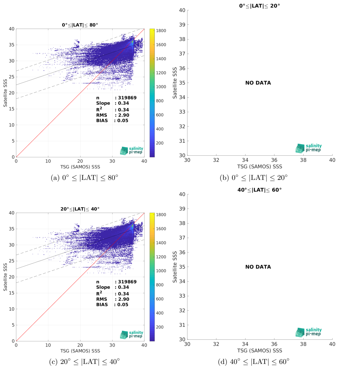
Figure 10: Contour maps of the concentration of SMOS SSS L4 v1 - Monthly (CMEMS-CNR) SSS (y-axis) versus TSG (SAMOS) SSS (x-axis) at match-up pairs for different latitude bands. For each plot, the red line shows x=y . The black thin and dashed lines indicate a linear fit through the data cloud and the \pm 95\% confidence levels, respectively. The number match-up pairs n , the slope and R^2 coefficient of the linear fit, the root mean square (RMS) and the mean bias between satellite and in situ data are indicated for each latitude band in each plots.
