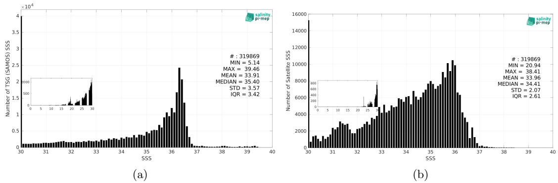
Figure 3: Histograms of SSS from TSG (SAMOS) (a) and SMOS SSS L4 v1 - Monthly (CMEMS-CNR) (b) considering all match-up pairs per bins of 0.1 over the Mississippi river plume Pi-MEP region and for the full satellite product period.
