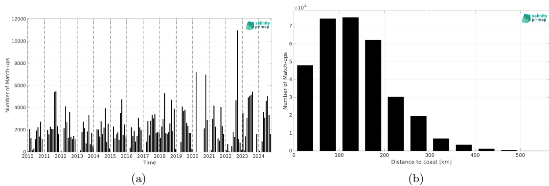
Figure 2: Number of match-ups between TSG (SAMOS) and SMOS SSS L4 v1 - Monthly (CMEMS-CNR) SSS as a function of time (a) and as function of the distance to coast (b) over the Mississippi river plume Pi-MEP region and for the full satellite product period.
