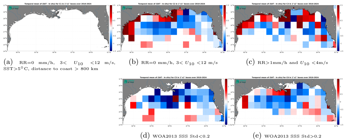
Figure 14: Temporal mean gridded over spatial boxes of size 1^\circ \times 1^\circ of \Delta SSS (SMOS SSS L4 v1 - Monthly (CMEMS-CNR) - TSG (SAMOS)) for 5 different subdatasets corresponding to: RR=0 mm/h, 3 < U_{10} < 12 m/s, SST > 5°C, distance to coast > 800 km (a), RR=0 mm/h, 3 < U_{10} < 12 m/s (b), RR > 1 mm/h and U_{10} < 4 m/s (c), WOA2013 SSS Std < 0.2 (d), WOA2013 SSS Std > 0.2 (e).
