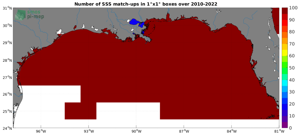
Figure 4: Number of SSS match-ups between TSG (SAMOS) SSS and the SMOS SSS L4 v1 - Monthly (CMEMS-CNR) SSS product for the Mississippi river plume Pi-MEP region over 1^\circ \times 1^\circ boxes and for the full satellite product period.
