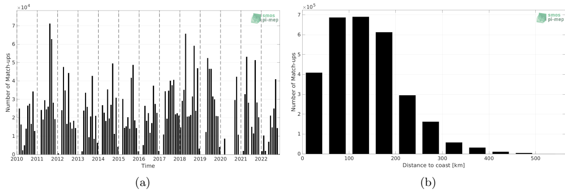
Figure 1: Number of match-ups between TSG (SAMOS) and SMOS SSS L4 v1 - Monthly (CMEMS-CNR) SSS as a function of time (a) and as function of the distance to coast (b) over the Mississippi river plume Pi-MEP region and for the full satellite product period.
