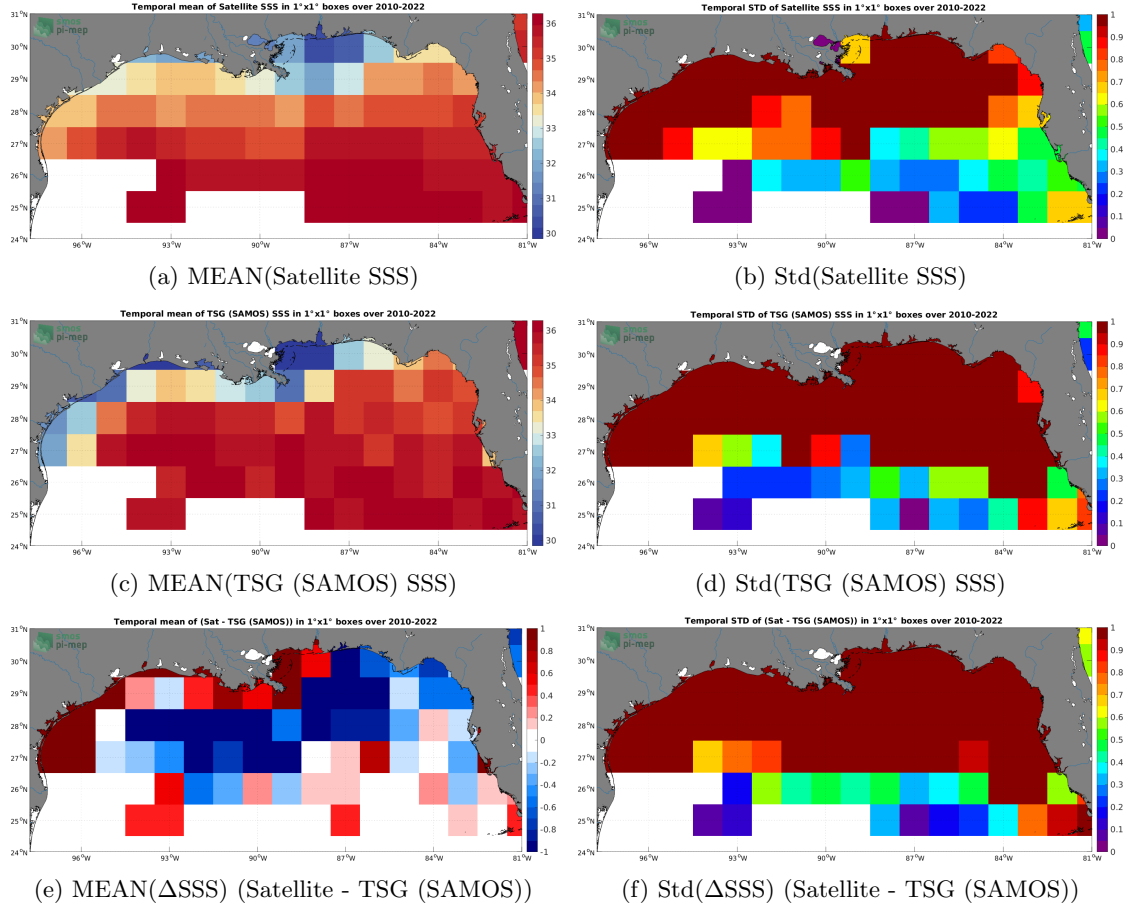
Figure 6: Temporal mean (left) and Std (right) of SSS from SMOS SSS L4 v1 - Monthly (CMEMS-CNR) (top), TSG (SAMOS) (middle), and of \Delta\text{SSS} (Satellite - TSG (SAMOS)). Only match-up pairs are used to generate these maps.
