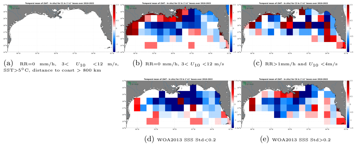
Figure 12: Temporal mean gridded over spatial boxes of size 1^{\circ}\times 1^{\circ} of \Delta\text{SSS} (SMOS SSS L4 v1 - Monthly (CMEMS-CNR) - TSG (SAMOS)) for 5 different subdatasets corresponding to:RR=0 mm/h, 3 < U_{10} < 12 m/s, SST >5^{\circ}\text{C} , distance to coast > 800 km (a), RR=0 mm/h, 3 < U_{10} < 12 m/s (b), RR >1 mm/h and U_{10} < 4 m/s (c), WOA2013 SSS Std <0.2 (d), WOA2013 SSS Std >0.2 (e).
