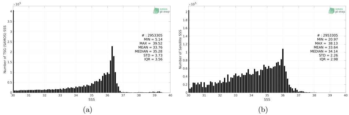
Figure 2: Histograms of SSS from TSG (SAMOS) (a) and SMOS SSS L4 v1 - Monthly (CMEMS-CNR) (b) considering all match-up pairs per bins of 0.1 over the Mississippi river plume Pi-MEP region and for the full satellite product period.
