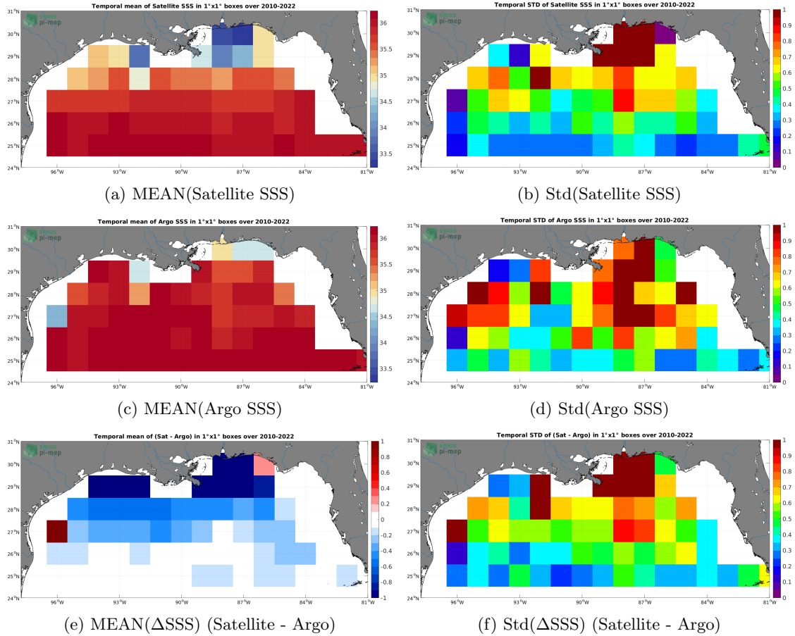
Figure 6: Temporal mean (left) and Std (right) of SSS from SMOS SSS L4 v1 - Monthly (CMEMS-CNR) (top), Argo (middle), and of \Delta\text{SSS} (Satellite - Argo). Only match-up pairs are used to generate these maps.
