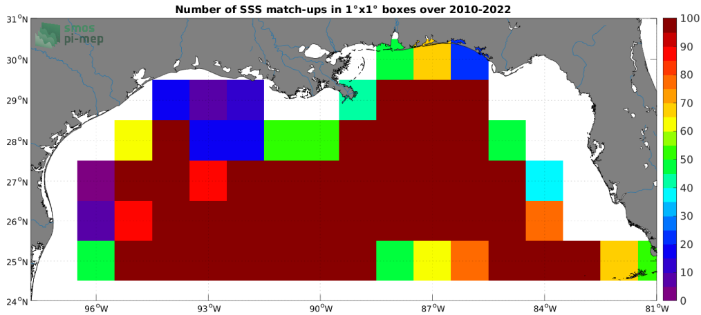
Figure 4: Number of SSS match-ups between Argo SSS and the SMOS SSS L4 v1 - Monthly (CMEMS-CNR) SSS product for the Mississippi river plume Pi-MEP region over 1^\circ \times 1^\circ boxes and for the full satellite product period.
