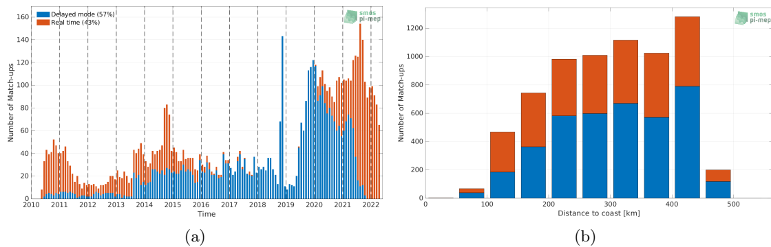
Figure 1: Number of match-ups between Argo and SMOS SSS L4 v1 - Monthly (CMEMS-CNR) SSS as a function of time (a) and as function of the distance to coast (b) over the Mississippi river plume Pi-MEP region and for the full satellite product period.
