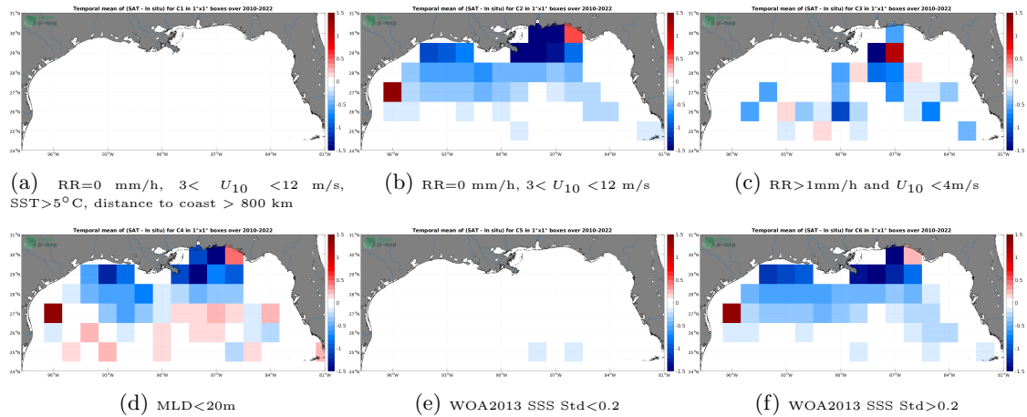
Figure 12: Temporal mean gridded over spatial boxes of size 1^{\circ}\times 1^{\circ} of \Delta\text{SSS} (SMOS SSS L4 v1 - Monthly (CMEMS-CNR) - Argo) for 6 different subdatasets corresponding to: RR=0 mm/h, 3 < U_{10} < 12 m/s, SST > 5^{\circ}\text{C} , distance to coast > 800 km (a), RR=0 mm/h, 3 < U_{10} < 12 m/s (b), RR > 1 mm/h and U_{10} < 4 m/s (c), MLD < 20\text{m} (d), WOA2013 SSS Std < 0.2 (e), WOA2013 SSS Std > 0.2 (f).
