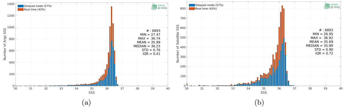
Figure 2: Histograms of SSS from Argo (a) and SMOS SSS L4 v1 - Monthly (CMEMS-CNR) (b) considering all match-up pairs per bins of 0.1 over the Mississippi river plume Pi-MEP region and for the full satellite product period.
