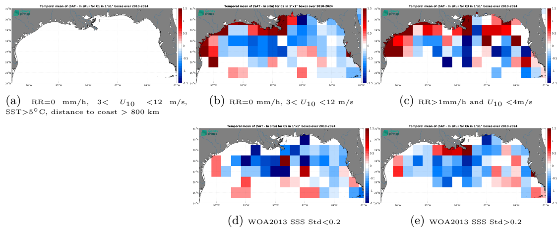
Figure 14: Temporal mean gridded over spatial boxes of size 1^\circ \times 1^\circ of \Delta SSS (SMOS SSS L4 v1 - Daily (CMEMS-CNR) - TSG (SAMOS)) for 5 different subdatasets corresponding to:RR=0 mm/h, 3 < U_{10} < 12 m/s, SST>5°C, distance to coast > 800 km (a), RR=0 mm/h, 3 < U_{10} < 12 m/s (b), RR>1mm/h and U_{10} < 4 m/s (c), WOA2013 SSS Std<0.2 (d), WOA2013 SSS Std>0.2 (e).
