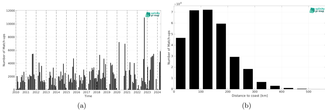
Figure 2: Number of match-ups between TSG (SAMOS) and SMOS SSS L4 v1 - Daily (CMEMS-CNR) SSS as a function of time (a) and as function of the distance to coast (b) over the Mississippi river plume Pi-MEP region and for the full satellite product period.
