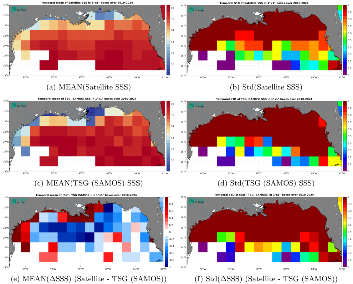
Figure 7: Temporal mean (left) and Std (right) of SSS from SMOS SSS L4 v1 - Daily (CMEMS-CNR) (top), TSG (SAMOS) (middle), and of \Delta\text{SSS} (Satellite - TSG (SAMOS)). Only match-up pairs are used to generate these maps.
