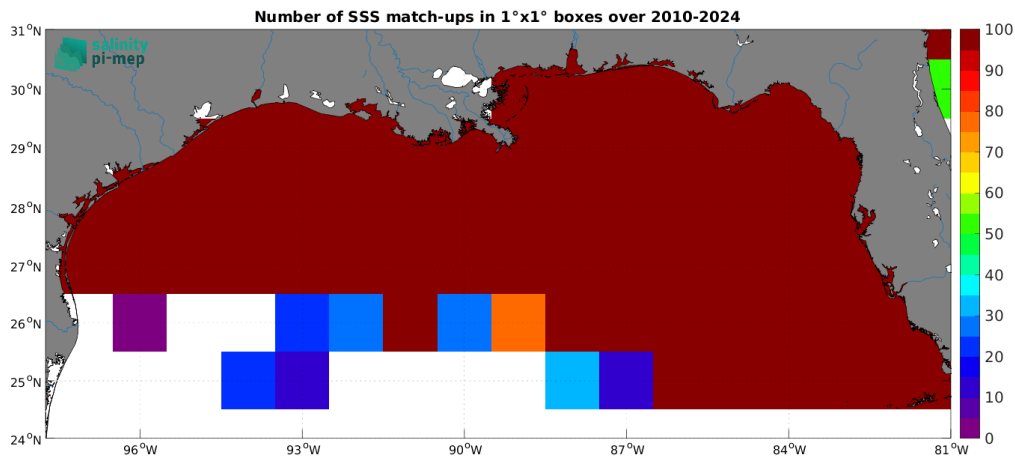
Figure 5: Number of SSS match-ups between TSG (SAMOS) SSS and the SMOS SSS L4 v1 - Daily (CMEMS-CNR) SSS product for the Mississippi river plume Pi-MEP region over 1^\circ \times 1^\circ boxes and for the full satellite product period.
