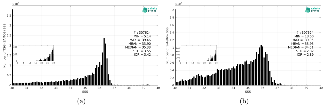
Figure 3: Histograms of SSS from TSG (SAMOS) (a) and SMOS SSS L4 v1 - Daily (CMEMS-CNR) (b) considering all match-up pairs per bins of 0.1 over the Mississippi river plume Pi-MEP region and for the full satellite product period.
