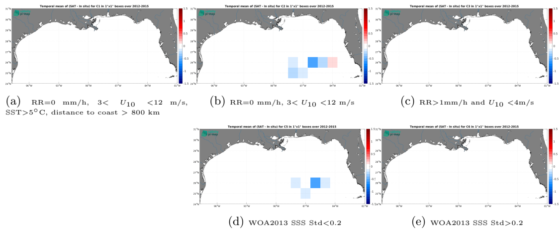
Figure 14: Temporal mean gridded over spatial boxes of size 1^\circ \times 1^\circ of \Delta\text{SSS} (SMOS SSS L4 v1 - Daily (CMEMS-CNR) - TSG (GOSUD-Sailing-ship)) for 5 different subdatasets corresponding to: RR=0 mm/h, 3 < U_{10} < 12 m/s, SST > 5°C, distance to coast > 800 km (a), RR=0 mm/h, 3 < U_{10} < 12 m/s (b), RR > 1mm/h and U_{10} < 4 m/s (c), WOA2013 SSS Std < 0.2 (d), WOA2013 SSS Std > 0.2 (e).
