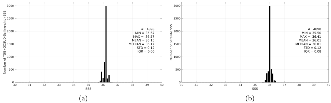
Figure 3: Histograms of SSS from TSG (GOSUD-Sailing-ship) (a) and SMOS SSS L4 v1 - Daily (CMEMS-CNR) (b) considering all match-up pairs per bins of 0.1 over the Mississippi river plume Pi-MEP region and for the full satellite product period.
