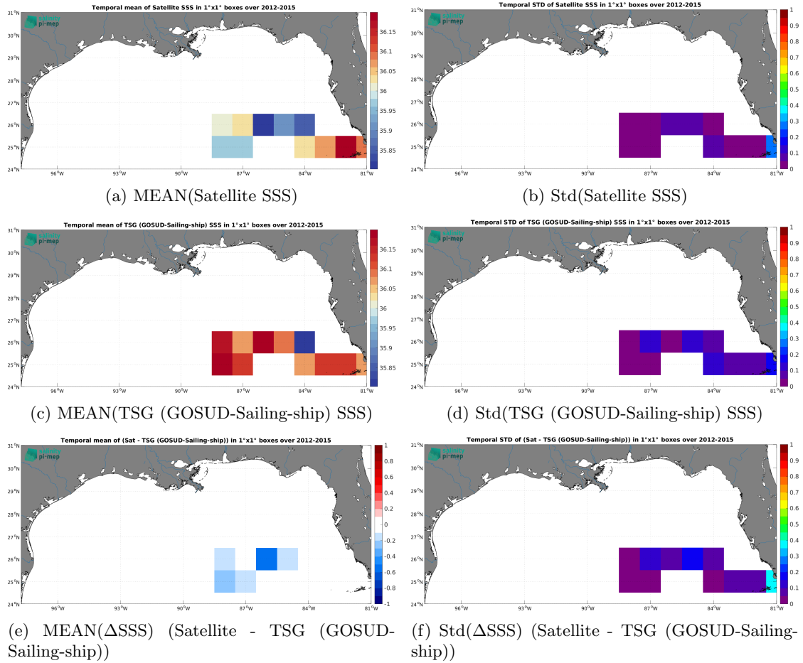
Figure 7: Temporal mean (left) and Std (right) of SSS from SMOS SSS L4 v1 - Daily (CMEMS-CNR) (top), TSG (GOSUD-Sailing-ship) (middle), and of \Delta\text{SSS} (Satellite - TSG (GOSUD-Sailing-ship)). Only match-up pairs are used to generate these maps.
