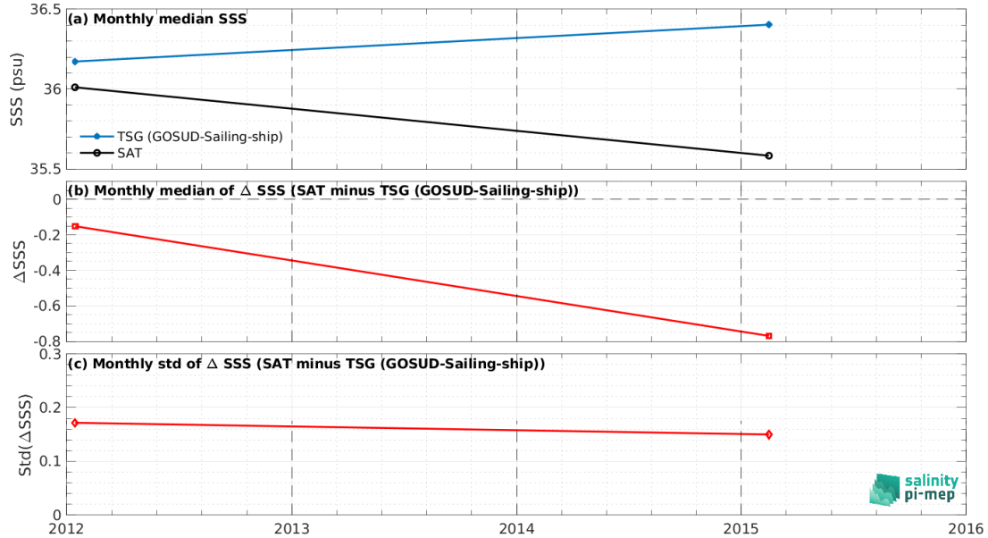
Figure 8: Time series of the monthly median SSS (top), median of \Delta\text{SSS} (Satellite - TSG (GOSUD-Sailing-ship)) and Std of \Delta\text{SSS} (Satellite - TSG (GOSUD-Sailing-ship)) over the Mississippi river plume Pi-MEP region considering all match-ups collected by the Pi-MEP.
