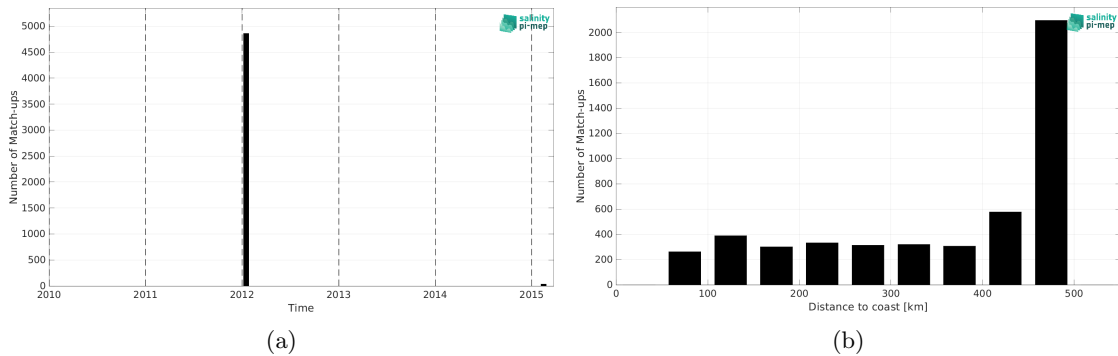
Figure 2: Number of match-ups between TSG (GOSUD-Sailing-ship) and SMOS SSS L4 v1 - Daily (CMEMS-CNR) SSS as a function of time (a) and as function of the distance to coast (b) over the Mississippi river plume Pi-MEP region and for the full satellite product period.
