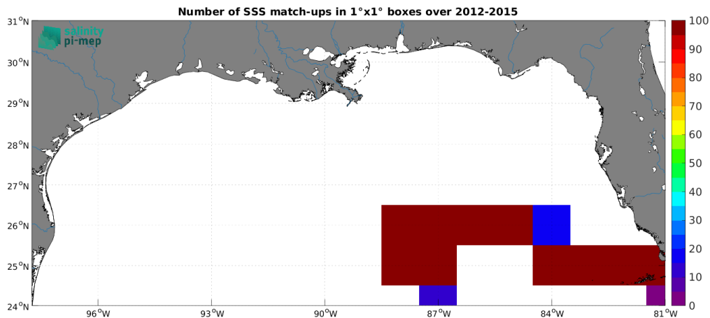
Figure 5: Number of SSS match-ups between TSG (GOSUD-Sailing-ship) SSS and the SMOS SSS L4 OI v346 - Weekly (CMEMS-CATDS-LOPS) SSS product for the Mississippi river plume Pi-MEP region over 1^\circ \times 1^\circ boxes and for the full satellite product period.
