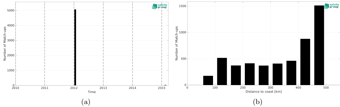
Figure 2: Number of match-ups between TSG (GOSUD-Sailing-ship) and SMOS SSS L4 OI v346 - Weekly (CMEMS-CATDS-LOPS) SSS as a function of time (a) and as function of the distance to coast (b) over the Mississippi river plume Pi-MEP region and for the full satellite product period.
