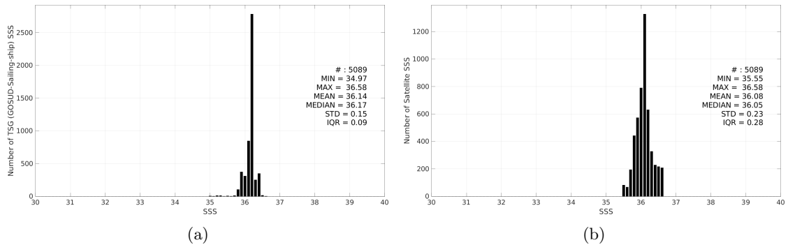
Figure 3: Histograms of SSS from TSG (GOSUD-Sailing-ship) (a) and SMOS SSS L4 OI v346 - Weekly (CMEMS-CATDS-LOPS) (b) considering all match-up pairs per bins of 0.1 over the Mississippi river plume Pi-MEP region and for the full satellite product period.
