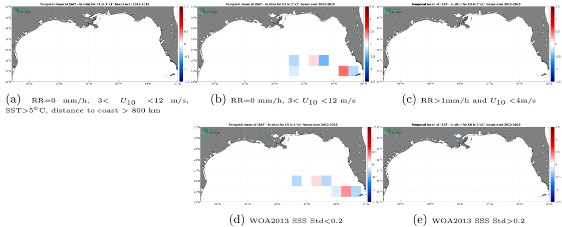
Figure 12: Temporal mean gridded over spatial boxes of size 1^{\circ}\times 1^{\circ} of \Delta SSS (SMOS SSS L4 OI v342 - Weekly (CMEMS-CATDS-LOPS) - TSG (GOSUD-Sailing-ship)) for 5 different sub-datasets corresponding to:RR=0 mm/h, 3 < U_{10} < 12 m/s, SST >5^{\circ}\text{C} , distance to coast > 800 km (a), RR=0 mm/h, 3 < U_{10} < 12 m/s (b), RR >1 mm/h and U_{10} < 4 m/s (c), WOA2013 SSS Std <0.2 (d), WOA2013 SSS Std >0.2 (e).
