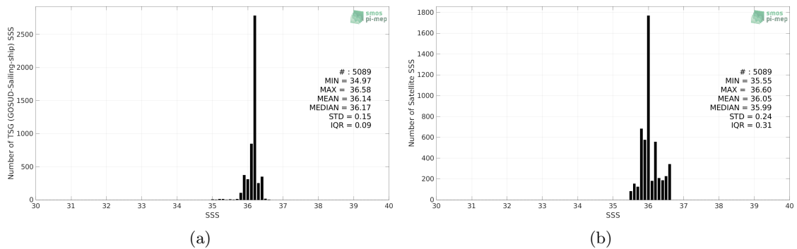
Figure 2: Histograms of SSS from TSG (GOSUD-Sailing-ship) (a) and SMOS SSS L4 OI v342 - Weekly (CMEMS-CATDS-LOPS) (b) considering all match-up pairs per bins of 0.1 over the Mississippi river plume Pi-MEP region and for the full satellite product period.
