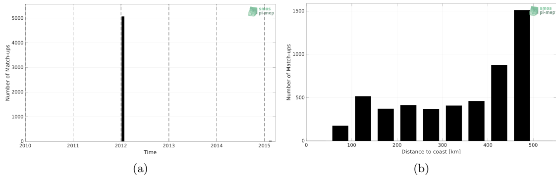
Figure 1: Number of match-ups between TSG (GOSUD-Sailing-ship) and SMOS SSS L4 OI v342 - Weekly (CMEMS-CATDS-LOPS) SSS as a function of time (a) and as function of the distance to coast (b) over the Mississippi river plume Pi-MEP region and for the full satellite product period.
