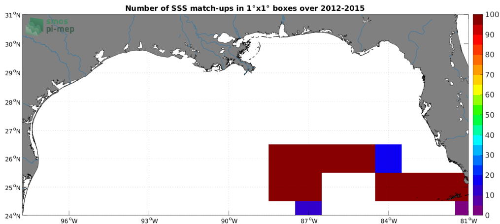
Figure 4: Number of SSS match-ups between TSG (GOSUD-Sailing-ship) SSS and the SMOS SSS L4 OI v342 - Weekly (CMEMS-CATDS-LOPS) SSS product for the Mississippi river plume Pi-MEP region over 1^\circ \times 1^\circ boxes and for the full satellite product period.
