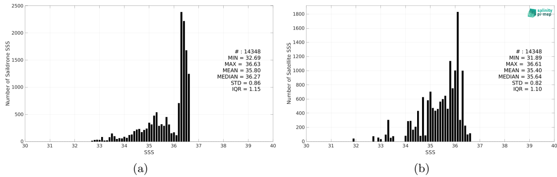
Figure 2: Histograms of SSS from Saildrone (a) and SMOS SSS L4 OI v342 - Weekly (CMEMS-CATDS-LOPS) (b) considering all match-up pairs per bins of 0.1 over the Mississippi river plume Pi-MEP region and for the full satellite product period.
