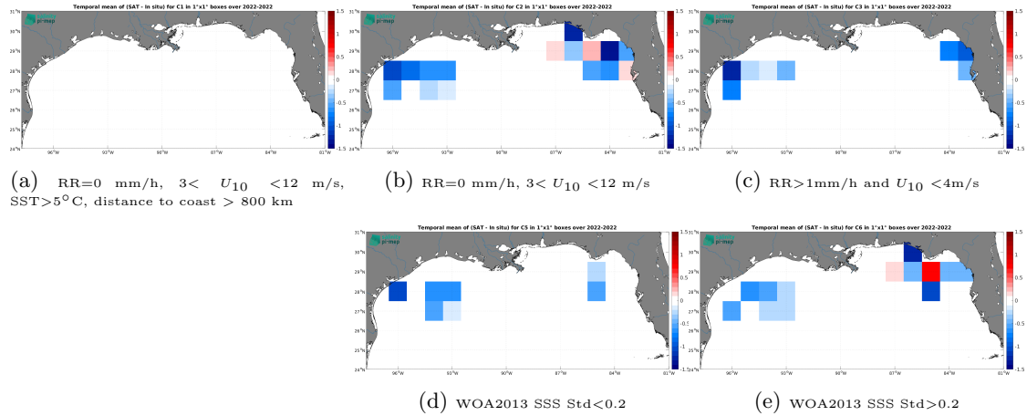
Figure 12: Temporal mean gridded over spatial boxes of size 1^{\circ}\times 1^{\circ} of \Delta\text{SSS} (SMOS SSS L4 OI v342 - Weekly (CMEMS-CATDS-LOPS) - Saildrone) for 5 different subdatasets corresponding to:RR=0 mm/h, 3 < U_{10} < 12 m/s, SST >5^{\circ}\text{C} , distance to coast > 800 km (a), RR=0 mm/h, 3 < U_{10} < 12 m/s (b), RR >1 mm/h and U_{10} < 4 m/s (c), WOA2013 SSS Std <0.2 (d), WOA2013 SSS Std >0.2 (e).
