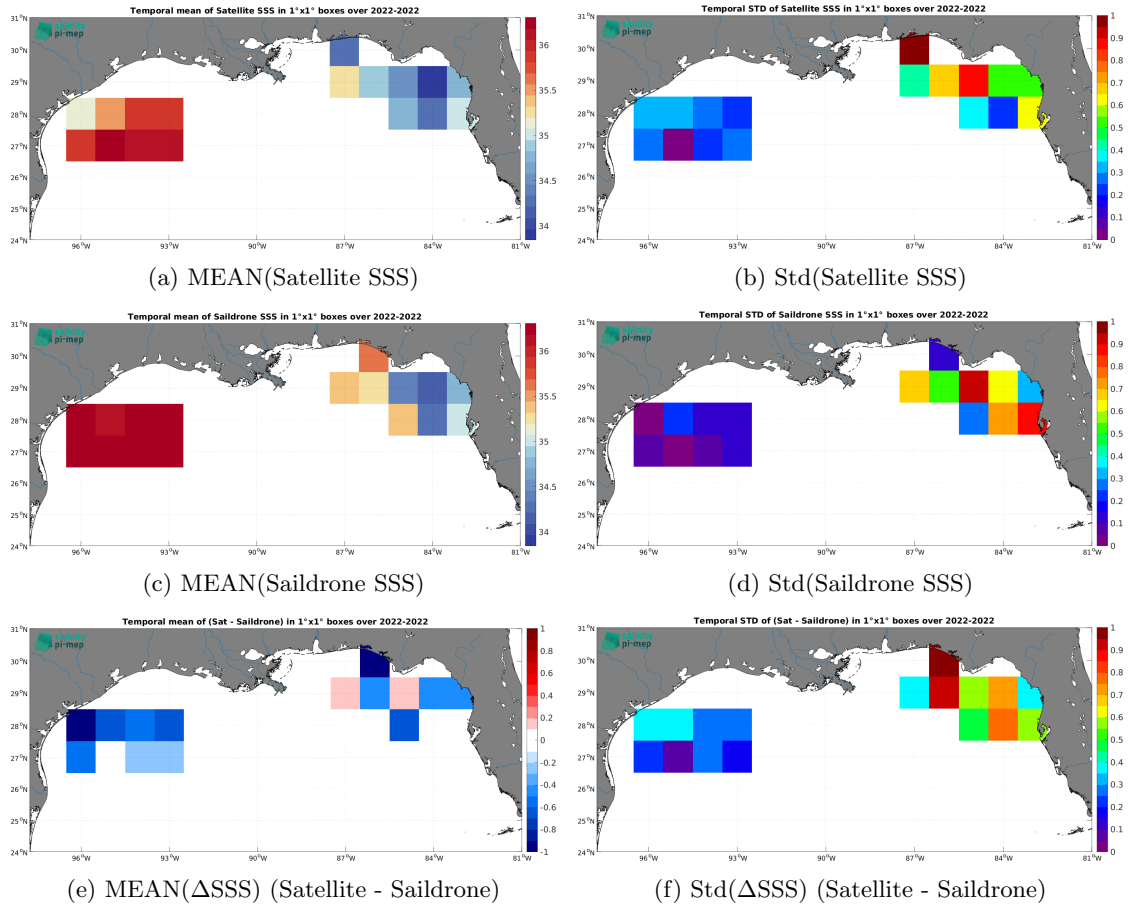
Figure 6: Temporal mean (left) and Std (right) of SSS from SMOS SSS L4 OI v342 - Weekly (CMEMS-CATDS-LOPS) (top), Saildrone (middle), and of \Delta SSS (Satellite - Saildrone). Only match-up pairs are used to generate these maps.
