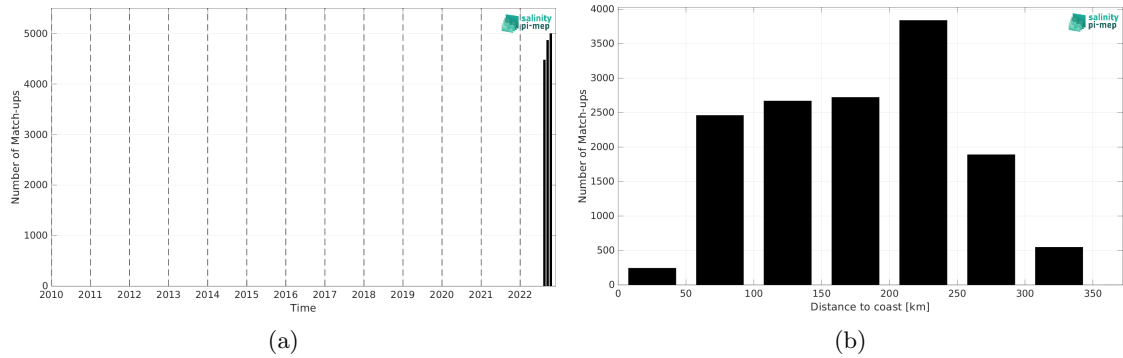
Figure 1: Number of match-ups between Saildrone and SMOS SSS L4 OI v342 - Weekly (CMEMS-CATDS-LOPS) SSS as a function of time (a) and as function of the distance to coast (b) over the Mississippi river plume Pi-MEP region and for the full satellite product period.
