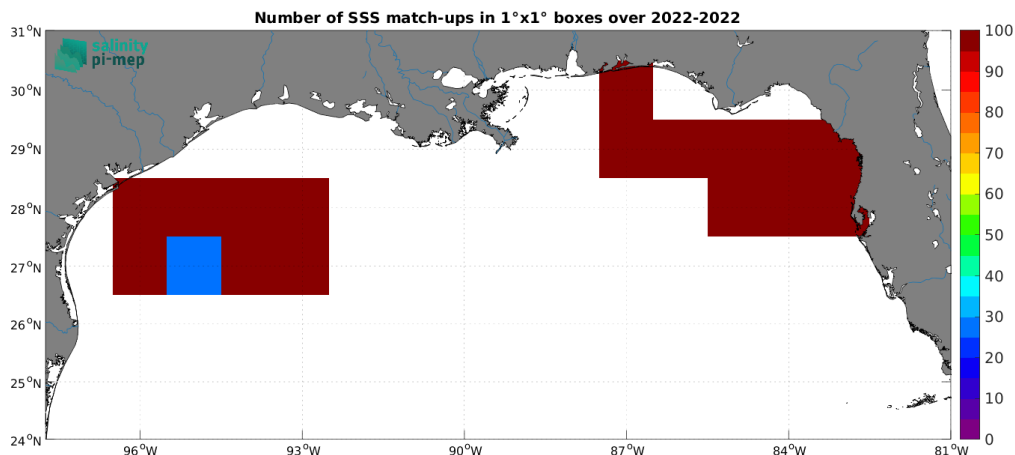
Figure 4: Number of SSS match-ups between Saildrone SSS and the SMOS SSS L4 OI v342 - Weekly (CMEMS-CATDS-LOPS) SSS product for the Mississippi river plume Pi-MEP region over 1^\circ \times 1^\circ boxes and for the full satellite product period.
