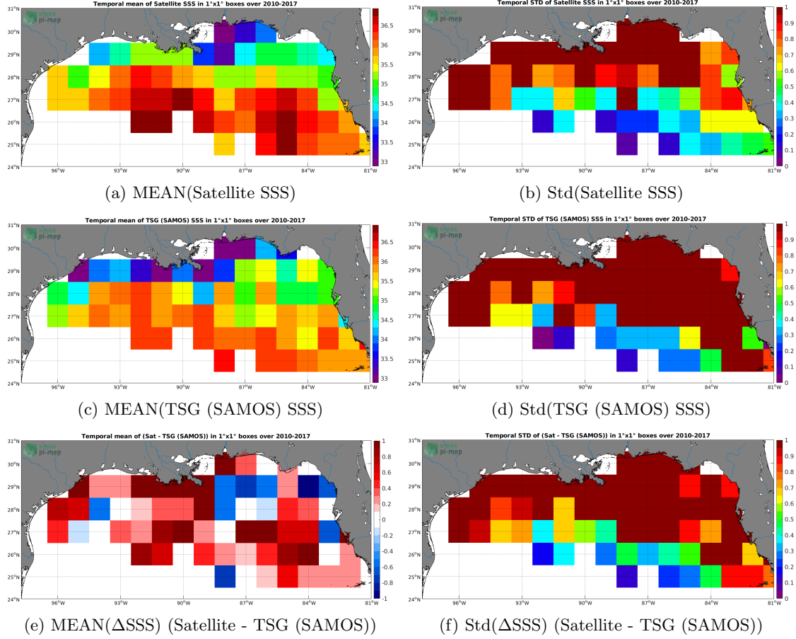
Figure 6: Temporal mean (left) and Std (right) of SSS from SMOS L4 v2 Weekly (CATDS-CECOS-IFREMER) (top), TSG (SAMOS) (middle), and of \Delta\text{SSS} (Satellite - TSG (SAMOS)). Only match-up pairs are used to generate these maps.
