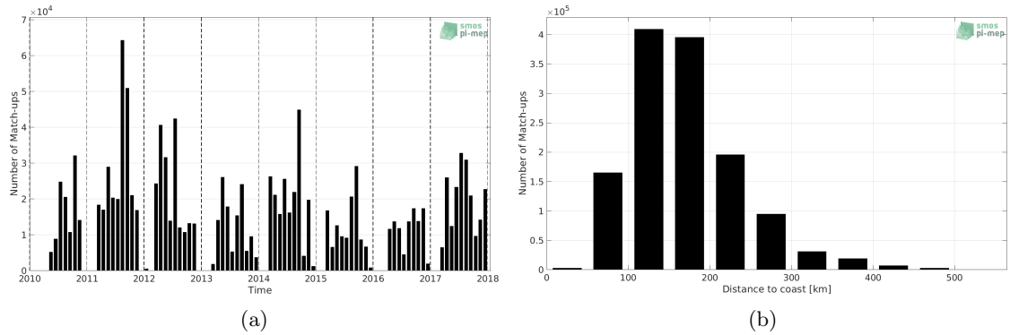
Figure 1: Number of match-ups between TSG (SAMOS) and SMOS L4 v2 Weekly (CATDS-CECOS-IFREMER) SSS as a function of time (a) and as function of the distance to coast (b) over the Mississippi river plume Pi-MEP region and for the full satellite product period.
