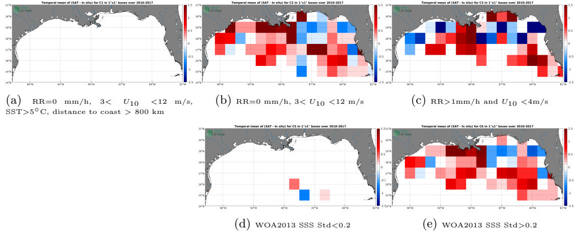
Figure 12: Temporal mean gridded over spatial boxes of size 1^{\circ}\times 1^{\circ} of \Delta\text{SSS} (SMOS L4 v2 Weekly (CATDS-CECOS-IFREMER) - TSG (SAMOS)) for 5 different subdatasets corresponding to: RR=0 mm/h, 3 < U_{10} < 12 m/s, SST > 5^{\circ}\text{C} , distance to coast > 800 km (a), RR=0 mm/h, 3 < U_{10} < 12 m/s (b), RR > 1\text{mm/h} and U_{10} < 4\text{m/s} (c), WOA2013 SSS Std < 0.2 (d), WOA2013 SSS Std > 0.2 (e).
