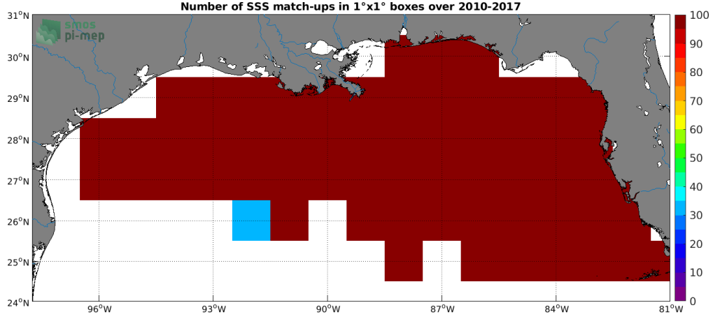
Figure 4: Number of SSS match-ups between TSG (SAMOS) SSS and the SMOS L4 v2 Weekly (CATDS-CECOS-IFREMER) SSS product for the Mississippi river plume Pi-MEP region over 1^\circ \times 1^\circ boxes and for the full satellite product period.
