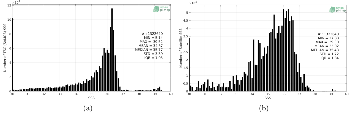
Figure 2: Histograms of SSS from TSG (SAMOS) (a) and SMOS L4 v2 Weekly (CATDS-CECOS-IFREMER) (b) considering all match-up pairs per bins of 0.1 over the Mississippi river plume Pi-MEP region and for the full satellite product period.
