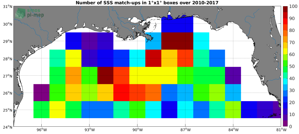
Figure 4: Number of SSS match-ups between Argo SSS and the SMOS L4 v2 Weekly (CATDS-CECOS-IFREMER) SSS product for the Mississippi river plume Pi-MEP region over 1^\circ \times 1^\circ boxes and for the full satellite product period.
