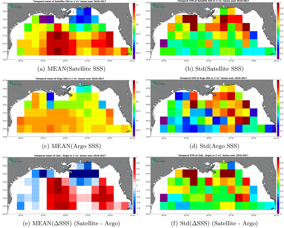
Figure 6: Temporal mean (left) and Std (right) of SSS from SMOS L4 v2 Weekly (CATDS-CECOS-IFREMER) (top), Argo (middle), and of \Delta\text{SSS} (Satellite - Argo). Only match-up pairs are used to generate these maps.
