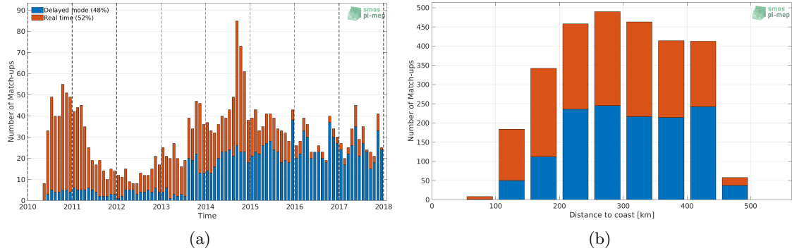
Figure 1: Number of match-ups between Argo and SMOS L4 v2 Weekly (CATDS-CECOS-IFREMER) SSS as a function of time (a) and as function of the distance to coast (b) over the Mississippi river plume Pi-MEP region and for the full satellite product period.
