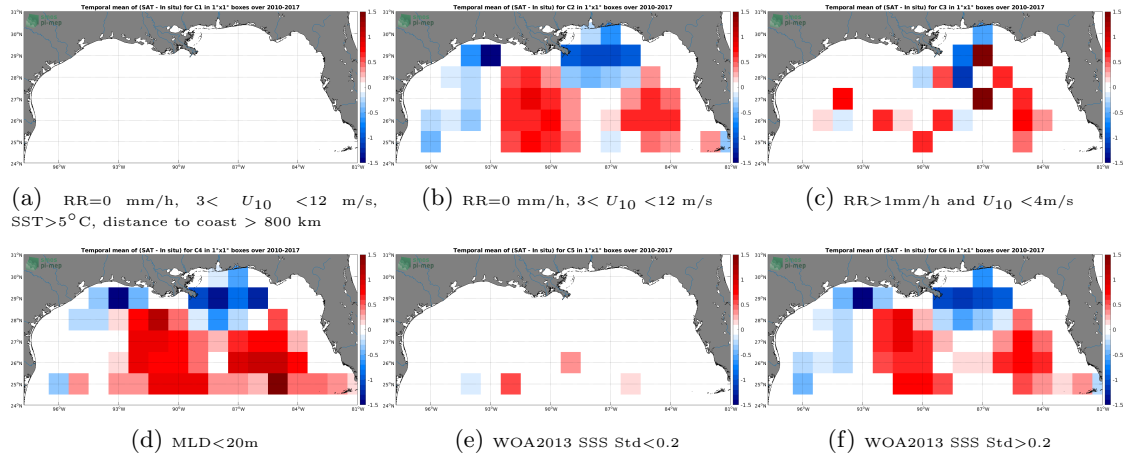
Figure 12: Temporal mean gridded over spatial boxes of size 1^{\circ}\times 1^{\circ} of \Delta\text{SSS} (SMOS L4 v2 Weekly (CATDS-CECOS-IFREMER) - Argo) for 6 different subdatasets corresponding to:RR=0 mm/h, 3 < U_{10} < 12 m/s, SST >5^{\circ}\text{C} , distance to coast > 800 km (a), RR=0 mm/h, 3 < U_{10} < 12 m/s (b), RR >1\text{mm/h} and U_{10} < 4\text{m/s} (c),MLD <20\text{m} (d),WOA2013 SSS Std <0.2 (e),WOA2013 SSS Std >0.2 (f).
