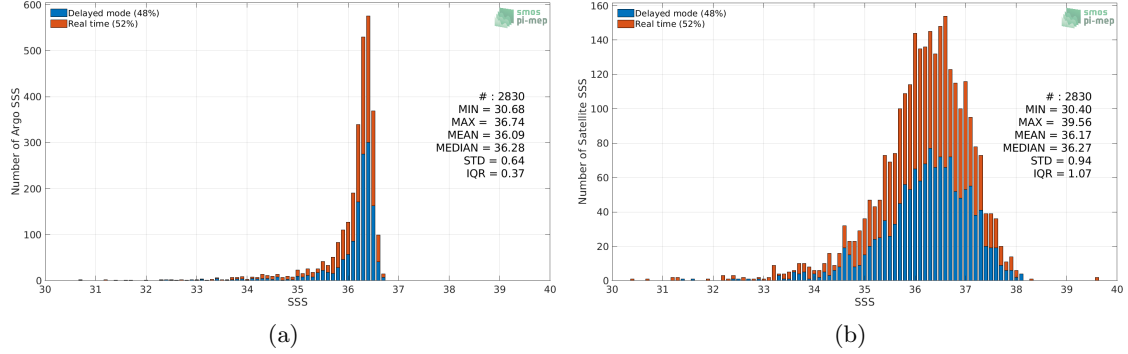
Figure 2: Histograms of SSS from Argo (a) and SMOS L4 v2 Weekly (CATDS-CECOS-IFREMER) (b) considering all match-up pairs per bins of 0.1 over the Mississippi river plume Pi-MEP region and for the full satellite product period.
