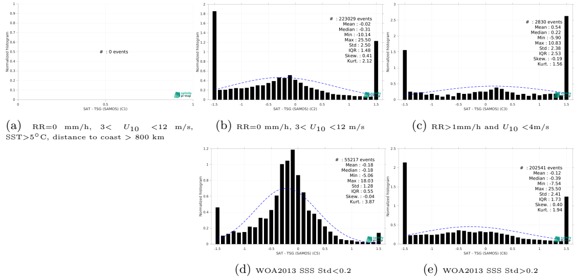
Figure 15: Normalized histogram of \Delta\text{SSS} (SMOS SSS L4 v2 - Daily (BEC) - TSG (SAMOS)) for 5 different subdatasets corresponding to: RR=0 mm/h, 3 < U_{10} < 12 m/s, SST>5°C, distance to coast > 800 km (a), RR=0 mm/h, 3 < U_{10} < 12 m/s (b), RR>1mm/h and U_{10} < 4 m/s (c), WOA2013 SSS Std<0.2 (d), WOA2013 SSS Std>0.2 (e).
