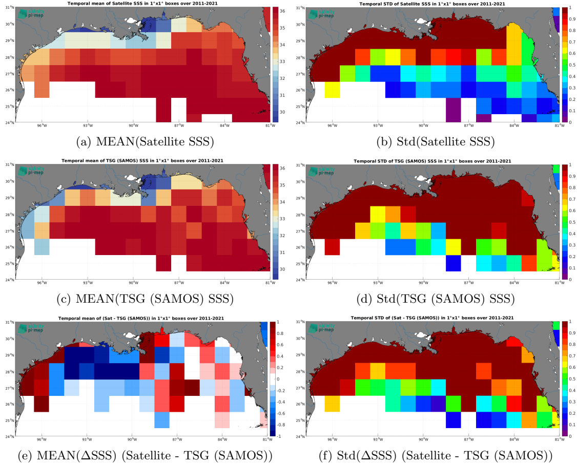
Figure 7: Temporal mean (left) and Std (right) of SSS from SMOS SSS L4 v2 - Daily (BEC) (top), TSG (SAMOS) (middle), and of \Delta\text{SSS} (Satellite - TSG (SAMOS)). Only match-up pairs are used to generate these maps.
