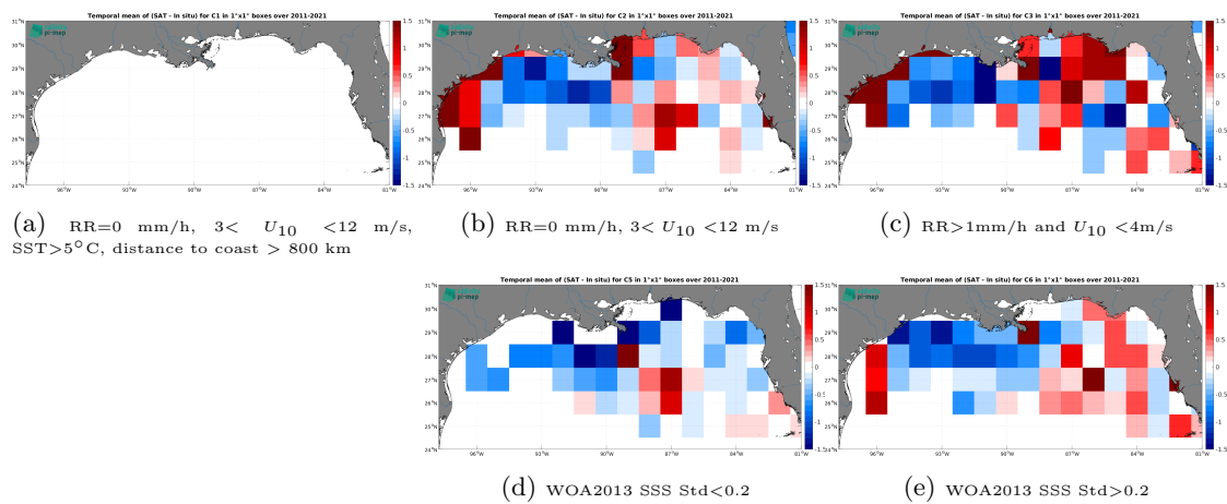
Figure 14: Temporal mean gridded over spatial boxes of size 1^\circ \times 1^\circ of \Delta SSS (SMOS SSS L4 v2 - Daily (BEC) - TSG (SAMOS)) for 5 different subdatasets corresponding to:RR=0 mm/h, 3 < U_{10} < 12 m/s, SST>5°C, distance to coast > 800 km (a), RR=0 mm/h, 3 < U_{10} < 12 m/s (b), RR>1mm/h and U_{10} < 4 m/s (c), WOA2013 SSS Std<0.2 (d), WOA2013 SSS Std>0.2 (e).
