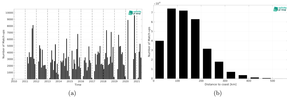
Figure 2: Number of match-ups between TSG (SAMOS) and SMOS SSS L4 v2 - Daily (BEC) SSS as a function of time (a) and as function of the distance to coast (b) over the Mississippi river plume Pi-MEP region and for the full satellite product period.
