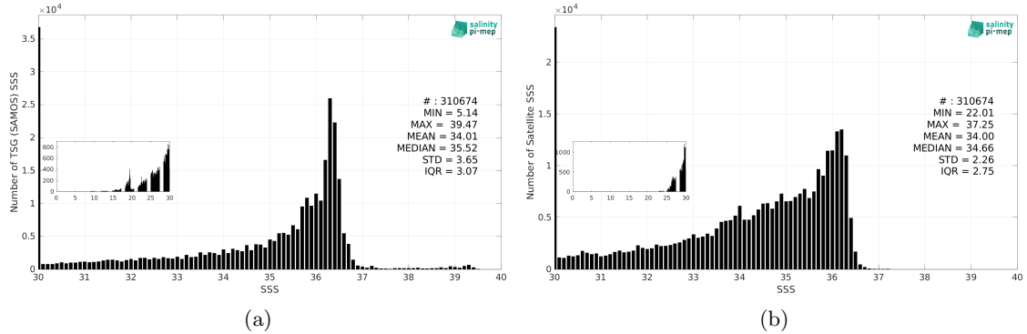
Figure 3: Histograms of SSS from TSG (SAMOS) (a) and SMOS SSS L4 v2 - Daily (BEC) (b) considering all match-up pairs per bins of 0.1 over the Mississippi river plume Pi-MEP region and for the full satellite product period.
