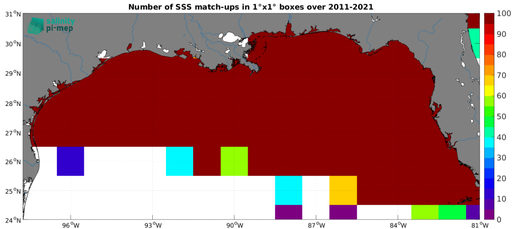
Figure 5: Number of SSS match-ups between TSG (SAMOS) SSS and the SMOS SSS L4 v2 - Daily (BEC) SSS product for the Mississippi river plume Pi-MEP region over 1^\circ \times 1^\circ boxes and for the full satellite product period.
