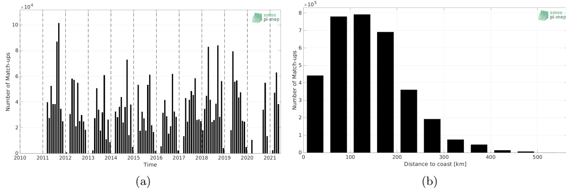
Figure 1: Number of match-ups between TSG (SAMOS) and SMOS SSS L4 v2 - Daily (BEC) SSS as a function of time (a) and as function of the distance to coast (b) over the Mississippi river plume Pi-MEP region and for the full satellite product period.
