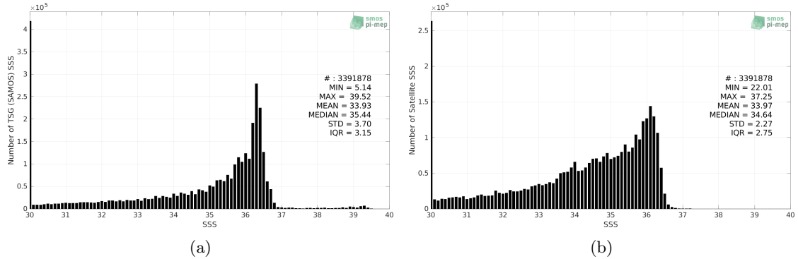
Figure 2: Histograms of SSS from TSG (SAMOS) (a) and SMOS SSS L4 v2 - Daily (BEC) (b) considering all match-up pairs per bins of 0.1 over the Mississippi river plume Pi-MEP region and for the full satellite product period.
