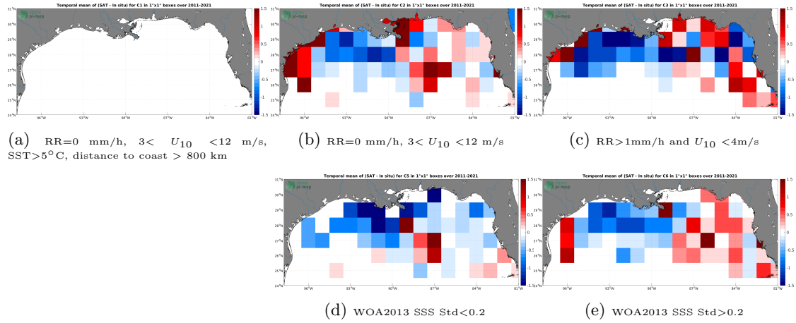
Figure 12: Temporal mean gridded over spatial boxes of size 1^{\circ}\times 1^{\circ} of \Delta\text{SSS} (SMOS SSS L4 v2 - Daily (BEC) - TSG (SAMOS)) for 5 different subdatasets corresponding to:RR=0 mm/h, 3 < U_{10} < 12 m/s, SST > 5^{\circ}\text{C} , distance to coast > 800 km (a), RR=0 mm/h, 3 < U_{10} < 12 m/s (b), RR > 1 mm/h and U_{10} < 4 m/s (c), WOA2013 SSS Std < 0.2 (d), WOA2013 SSS Std > 0.2 (e).
