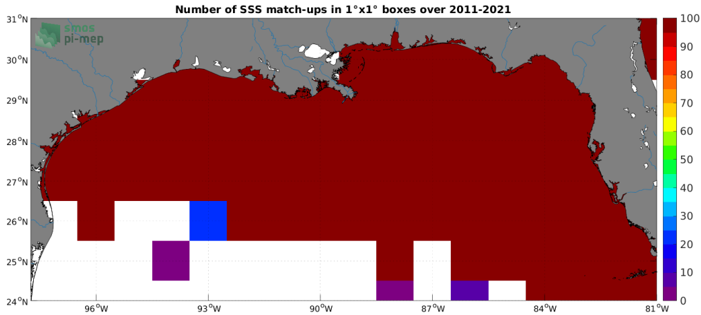
Figure 4: Number of SSS match-ups between TSG (SAMOS) SSS and the SMOS SSS L4 v2 - Daily (BEC) SSS product for the Mississippi river plume Pi-MEP region over 1^\circ \times 1^\circ boxes and for the full satellite product period.
