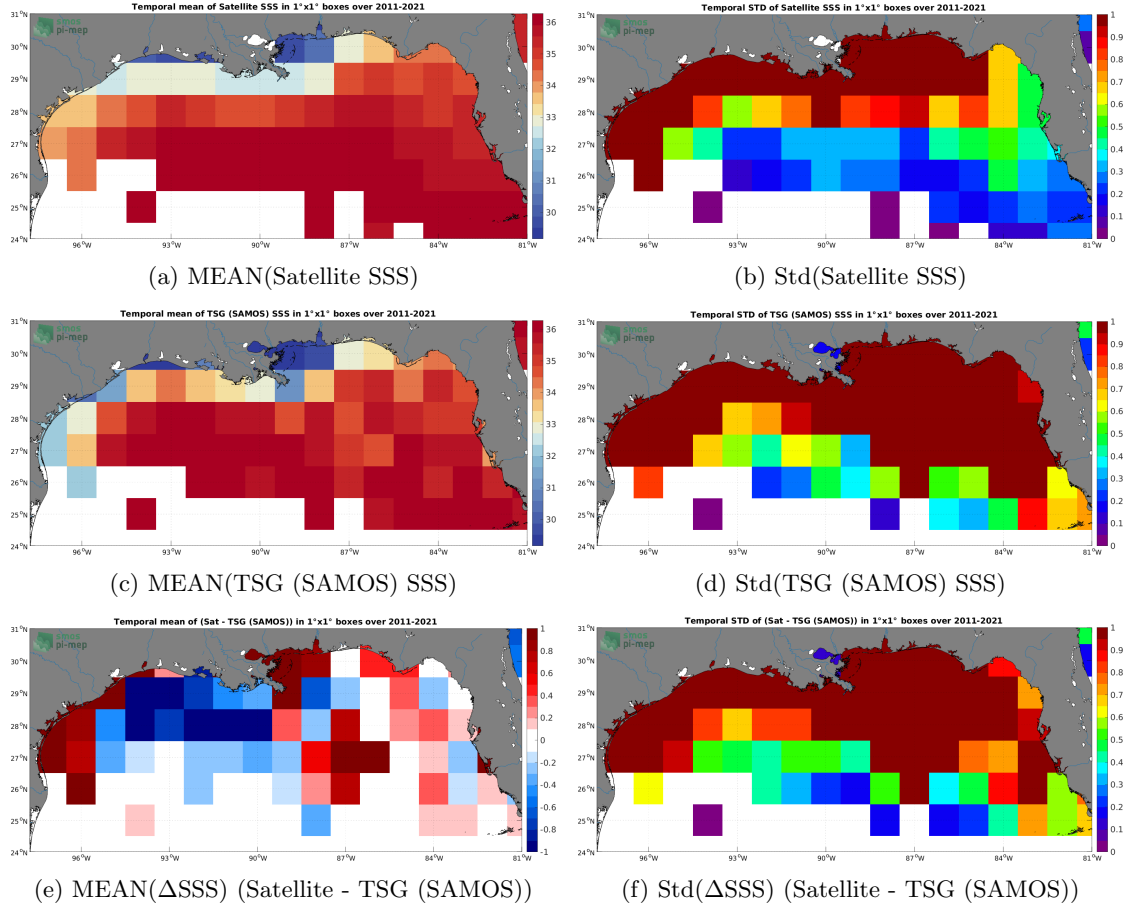
Figure 6: Temporal mean (left) and Std (right) of SSS from SMOS SSS L4 v2 - Daily (BEC) (top), TSG (SAMOS) (middle), and of \Delta\text{SSS} (Satellite - TSG (SAMOS)). Only match-up pairs are used to generate these maps.
