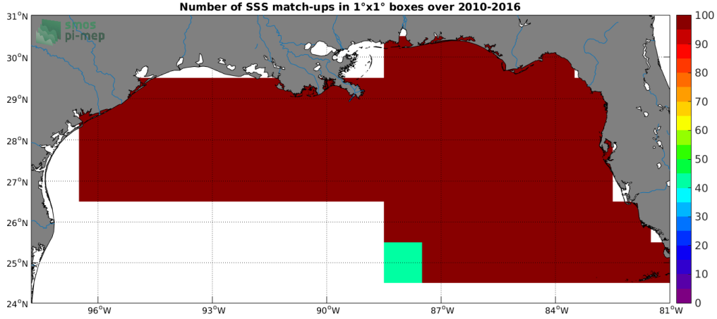
Figure 4: Number of SSS match-ups between TSG (SAMOS) SSS and the SMOS SSS L3 v3 Monthly (ICDC) SSS product for the Mississippi river plume Pi-MEP region over 1^\circ \times 1^\circ boxes and for the full satellite product period.
