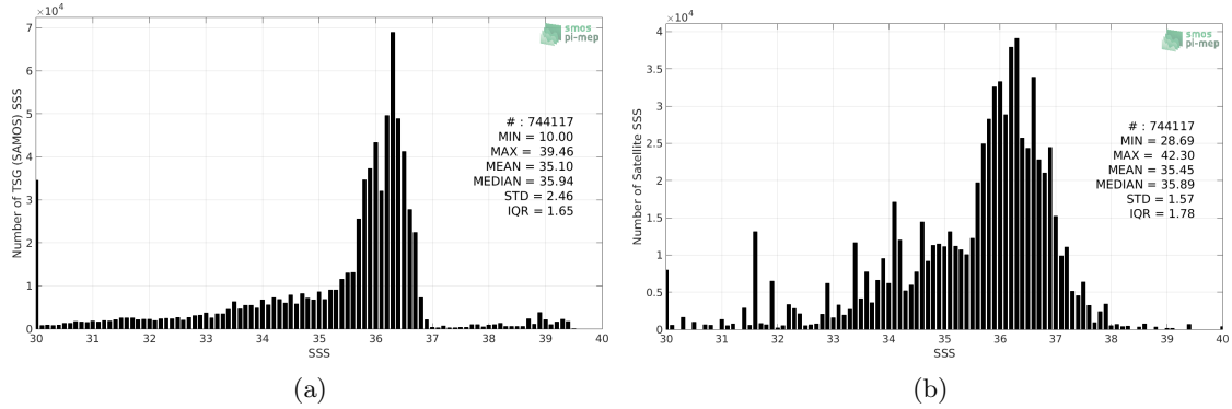
Figure 2: Histograms of SSS from TSG (SAMOS) (a) and SMOS SSS L3 v3 Monthly (ICDC) (b) considering all match-up pairs per bins of 0.1 over the Mississippi river plume Pi-MEP region and for the full satellite product period.
