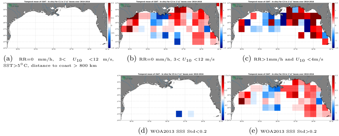
Figure 12: Temporal mean gridded over spatial boxes of size 1^{\circ}\times 1^{\circ} of \Delta\text{SSS} (SMOS SSS L3 v3 Monthly (ICDC) - TSG (SAMOS)) for 5 different subdatasets corresponding to:RR=0 mm/h, 3 < U_{10} < 12 m/s, SST >5^{\circ}\text{C} , distance to coast > 800 km (a), RR=0 mm/h, 3 < U_{10} < 12 m/s (b), RR >1\text{mm/h} and U_{10} < 4\text{m/s} (c), WOA2013 SSS Std <0.2 (d), WOA2013 SSS Std >0.2 (e).
