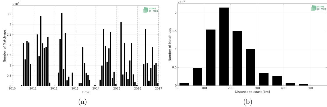
Figure 1: Number of match-ups between TSG (SAMOS) and SMOS SSS L3 v3 Monthly (ICDC) SSS as a function of time (a) and as function of the distance to coast (b) over the Mississippi river plume Pi-MEP region and for the full satellite product period.
