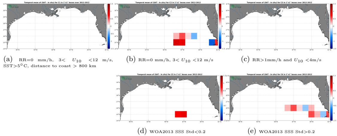
Figure 12: Temporal mean gridded over spatial boxes of size 1^\circ \times 1^\circ of \Delta SSS (SMOS SSS L3 v3 Monthly (ICDC) - TSG (GOSUD-Sailing-ship)) for 5 different subdatasets corresponding to: RR=0 mm/h, 3 < U_{10} < 12 m/s, SST >5^\circ\text{C} , distance to coast > 800 km (a), RR=0 mm/h, 3 < U_{10} < 12 m/s (b), RR >1 mm/h and U_{10} < 4 m/s (c), WOA2013 SSS Std <0.2 (d), WOA2013 SSS Std >0.2 (e).
