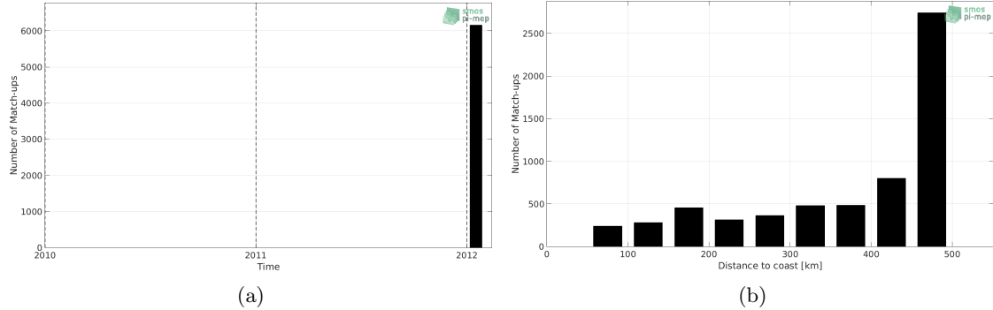
Figure 1: Number of match-ups between TSG (GOSUD-Sailing-ship) and SMOS SSS L3 v3 Monthly (ICDC) SSS as a function of time (a) and as function of the distance to coast (b) over the Mississippi river plume Pi-MEP region and for the full satellite product period.
