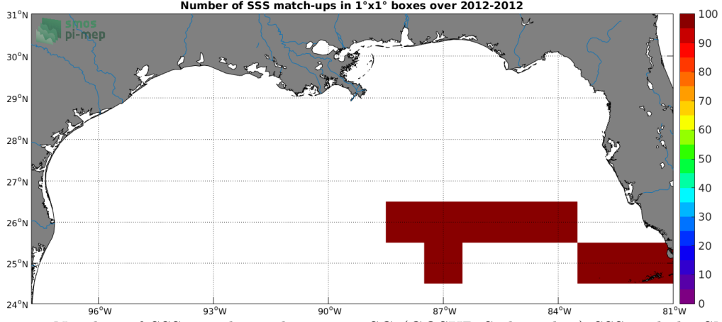
Figure 4: Number of SSS match-ups between TSG (GOSUD-Sailing-ship) SSS and the SMOS SSS L3 v3 Monthly (ICDC) SSS product for the Mississippi river plume Pi-MEP region over 1^\circ \times 1^\circ boxes and for the full satellite product period.
