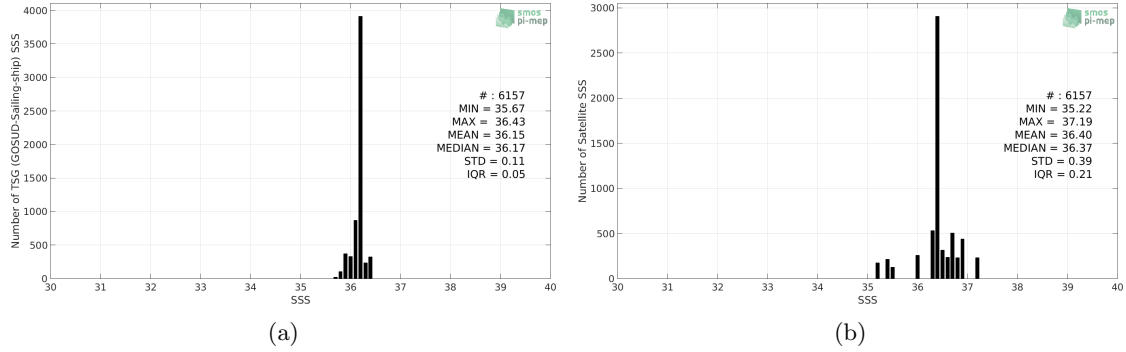
Figure 2: Histograms of SSS from TSG (GOSUD-Sailing-ship) (a) and SMOS SSS L3 v3 Monthly (ICDC) (b) considering all match-up pairs per bins of 0.1 over the Mississippi river plume Pi-MEP region and for the full satellite product period.
