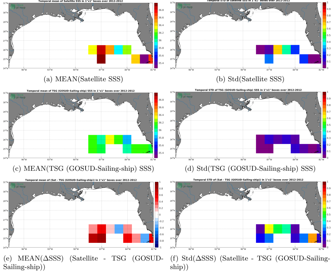
Figure 6: Temporal mean (left) and Std (right) of SSS from SMOS SSS L3 v3 Monthly (ICDC) (top), TSG (GOSUD-Sailing-ship) (middle), and of \Delta\text{SSS} (Satellite - TSG (GOSUD-Sailing-ship)). Only match-up pairs are used to generate these maps.
