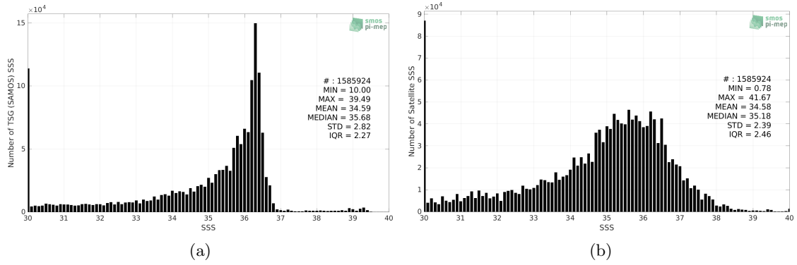
Figure 2: Histograms of SSS from TSG (SAMOS) (a) and SMOS SSS L2Q v331 - With FLAG (CMEMS-CATDS-CPDC) (b) considering all match-up pairs per bins of 0.1 over the Mississippi river plume Pi-MEP region and for the full satellite product period.
