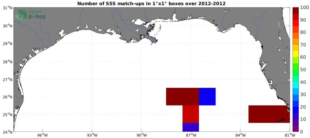
Figure 4: Number of SSS match-ups between TSG (GOSUD-Sailing-ship) SSS and the SMOS SSS L2Q v331 - With FLAG (CMEMS-CATDS-CPDC) SSS product for the Mississippi river plume Pi-MEP region over 1^\circ \times 1^\circ boxes and for the full satellite product period.
