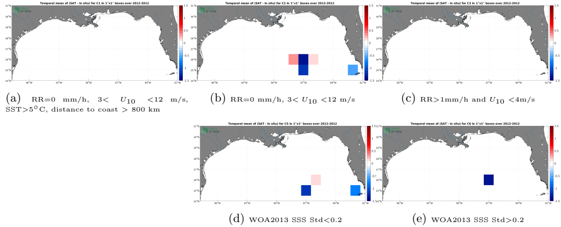
Figure 12: Temporal mean gridded over spatial boxes of size 1^{\circ}\times 1^{\circ} of \Delta SSS (SMOS SSS L2Q v331 - With FLAG (CMEMS-CATDS-CPDC) - TSG (GOSUD-Sailing-ship)) for 5 different subdatasets corresponding to:RR=0 mm/h, 3 < U_{10} < 12 m/s, SST >5^{\circ}\text{C} , distance to coast > 800 km (a), RR=0 mm/h, 3 < U_{10} < 12 m/s (b), RR >1 mm/h and U_{10} < 4 m/s (c), WOA2013 SSS Std <0.2 (d), WOA2013 SSS Std >0.2 (e).
