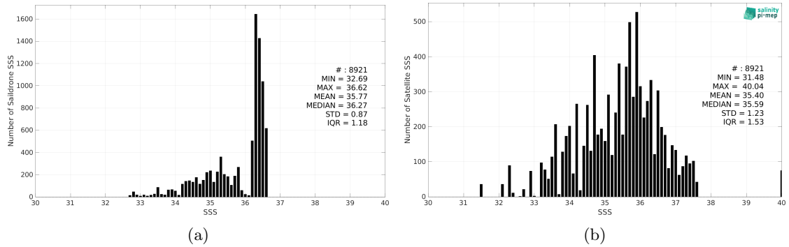
Figure 2: Histograms of SSS from Saildrone (a) and SMOS SSS L2Q v331 - With FLAG (CMEMS-CATDS-CPDC) (b) considering all match-up pairs per bins of 0.1 over the Mississippi river plume Pi-MEP region and for the full satellite product period.
