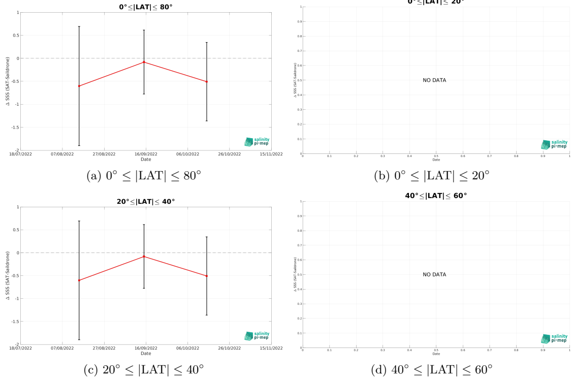
Figure 10: Monthly median (red curves) of \Delta SSS (Satellite - Sairdronne) and \pm 1 Std (black vertical thick bars) as function of time for all the collected Pi-MEP match-up pairs estimated over the Mississippi river plume Pi-MEP region and for the full satellite product period are shown for different latitude bands: (a) 80^{\circ}\text{S}-80^{\circ}\text{N} , (b) 20^{\circ}\text{S}-20^{\circ}\text{N} , (c) 40^{\circ}\text{S}-20^{\circ}\text{S} and 20^{\circ}\text{N}-40^{\circ}\text{N} and (d) 60^{\circ}\text{S}-40^{\circ}\text{S} and 40^{\circ}\text{N}-60^{\circ}\text{N} .
