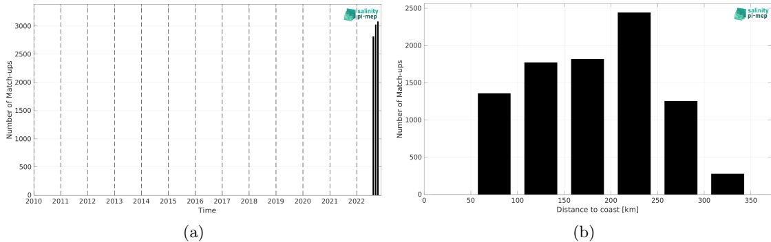
Figure 1: Number of match-ups between Saildrone and SMOS SSS L2Q v331 - With FLAG (CMEMS-CATDS-CPDC) SSS as a function of time (a) and as function of the distance to coast (b) over the Mississippi river plume Pi-MEP region and for the full satellite product period.
