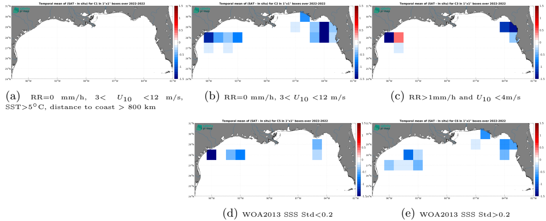
Figure 12: Temporal mean gridded over spatial boxes of size 1^{\circ}\times 1^{\circ} of \Delta\text{SSS} (SMOS SSS L2Q v331 - With FLAG (CMEMS-CATDS-CPDC) - Saildrone) for 5 different subdatasets corresponding to:RR=0 mm/h, 3 < U_{10} < 12 m/s, SST > 5^{\circ}\text{C} , distance to coast > 800 km (a), RR=0 mm/h, 3 < U_{10} < 12 m/s (b), RR > 1 mm/h and U_{10} < 4 m/s (c), WOA2013 SSS Std < 0.2 (d), WOA2013 SSS Std > 0.2 (e).
