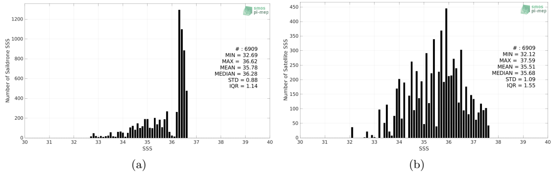
Figure 2: Histograms of SSS from Sairdrone (a) and SMOS SSS L2Q v331 - With FLAG (CMEMS-CATDS-CPDC) (b) considering all match-up pairs per bins of 0.1 over the Mississippi river plume Pi-MEP region and for the full satellite product period.
