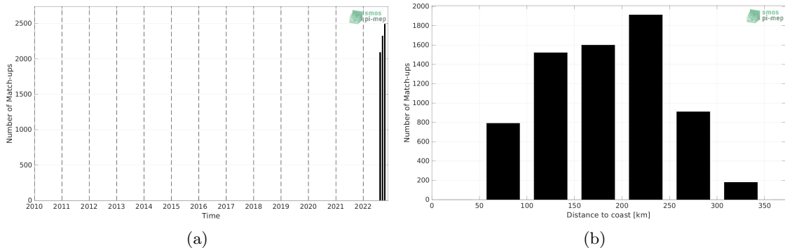
Figure 1: Number of match-ups between Sairdrone and SMOS SSS L2Q v331 - With FLAG (CMEMS-CATDS-CPDC) SSS as a function of time (a) and as function of the distance to coast (b) over the Mississippi river plume Pi-MEP region and for the full satellite product period.
