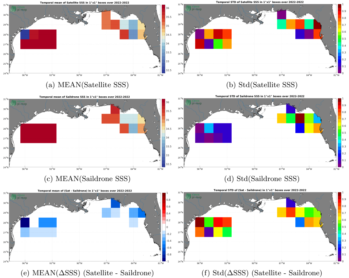
Figure 6: Temporal mean (left) and Std (right) of SSS from SMOS SSS L2Q v331 - With FLAG (CMEMS-CATDS-CPDC) (top), Saildrone (middle), and of \Delta\text{SSS} (Satellite - Saildrone). Only match-up pairs are used to generate these maps.
