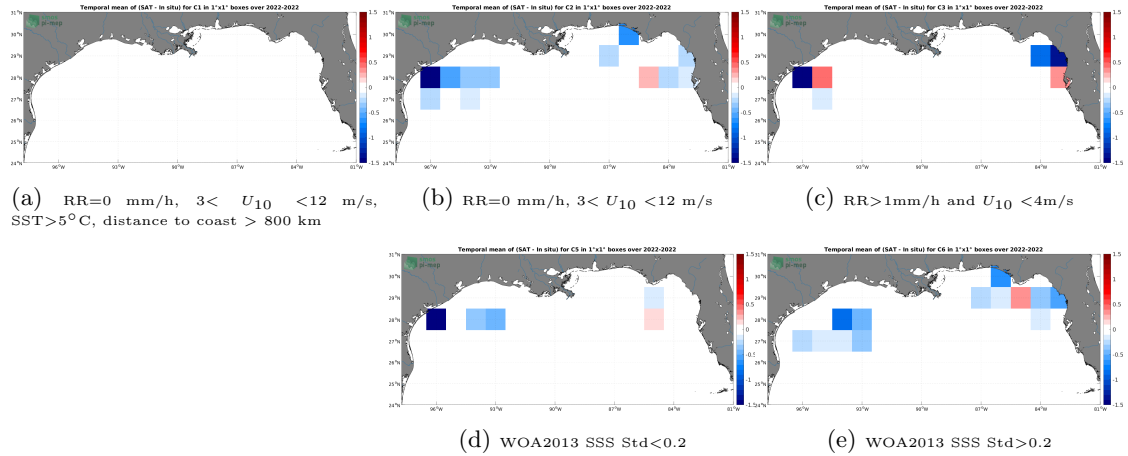
Figure 12: Temporal mean gridded over spatial boxes of size 1^{\circ}\times 1^{\circ} of \Delta\text{SSS} (SMOS SSS L2Q v331 - With FLAG (CMEMS-CATDS-CPDC) - Sairdrone) for 5 different subdatasets corresponding to:RR=0 mm/h, 3 < U_{10} < 12 m/s, SST > 5^{\circ}\text{C} , distance to coast > 800 km (a), RR=0 mm/h, 3 < U_{10} < 12 m/s (b), RR > 1 mm/h and U_{10} < 4 m/s (c), WOA2013 SSS Std < 0.2 (d), WOA2013 SSS Std > 0.2 (e).
