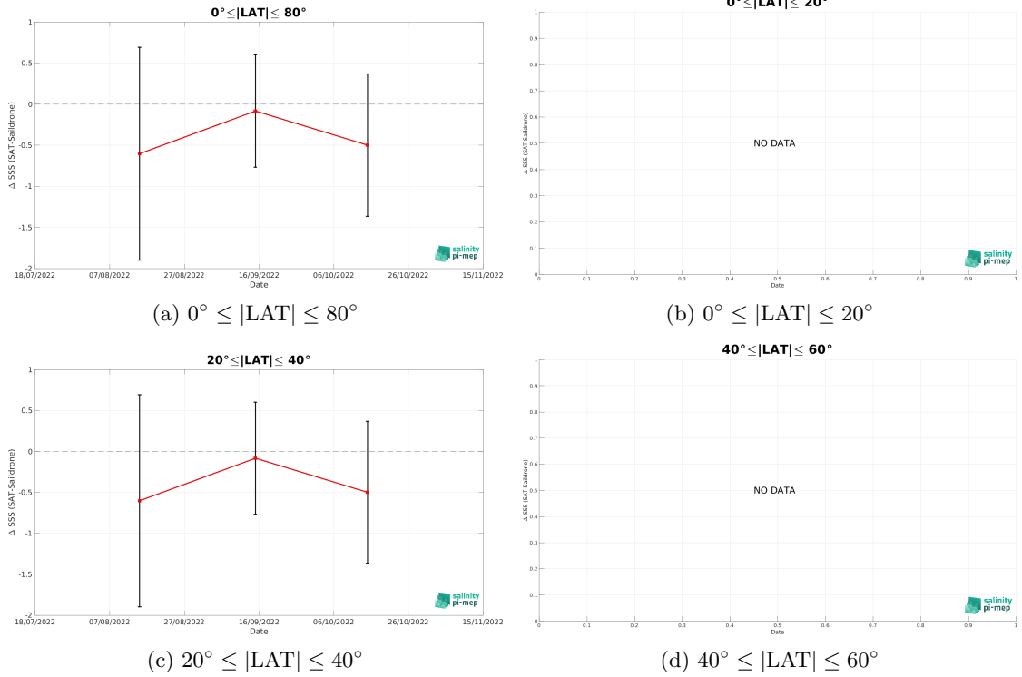
Figure 10: Monthly median (red curves) of \Delta SSS (Satellite - Sairdron ) and \pm 1 Std (black vertical thick bars) as function of time for all the collected Pi-MEP match-up pairs estimated over the Mississippi river plume Pi-MEP region and for the full satellite product period are shown for different latitude bands: (a) 80^{\circ}\text{S}-80^{\circ}\text{N} , (b) 20^{\circ}\text{S}-20^{\circ}\text{N} , (c) 40^{\circ}\text{S}-20^{\circ}\text{S} and 20^{\circ}\text{N}-40^{\circ}\text{N} and (d) 60^{\circ}\text{S}-40^{\circ}\text{S} and 40^{\circ}\text{N}-60^{\circ}\text{N} .
