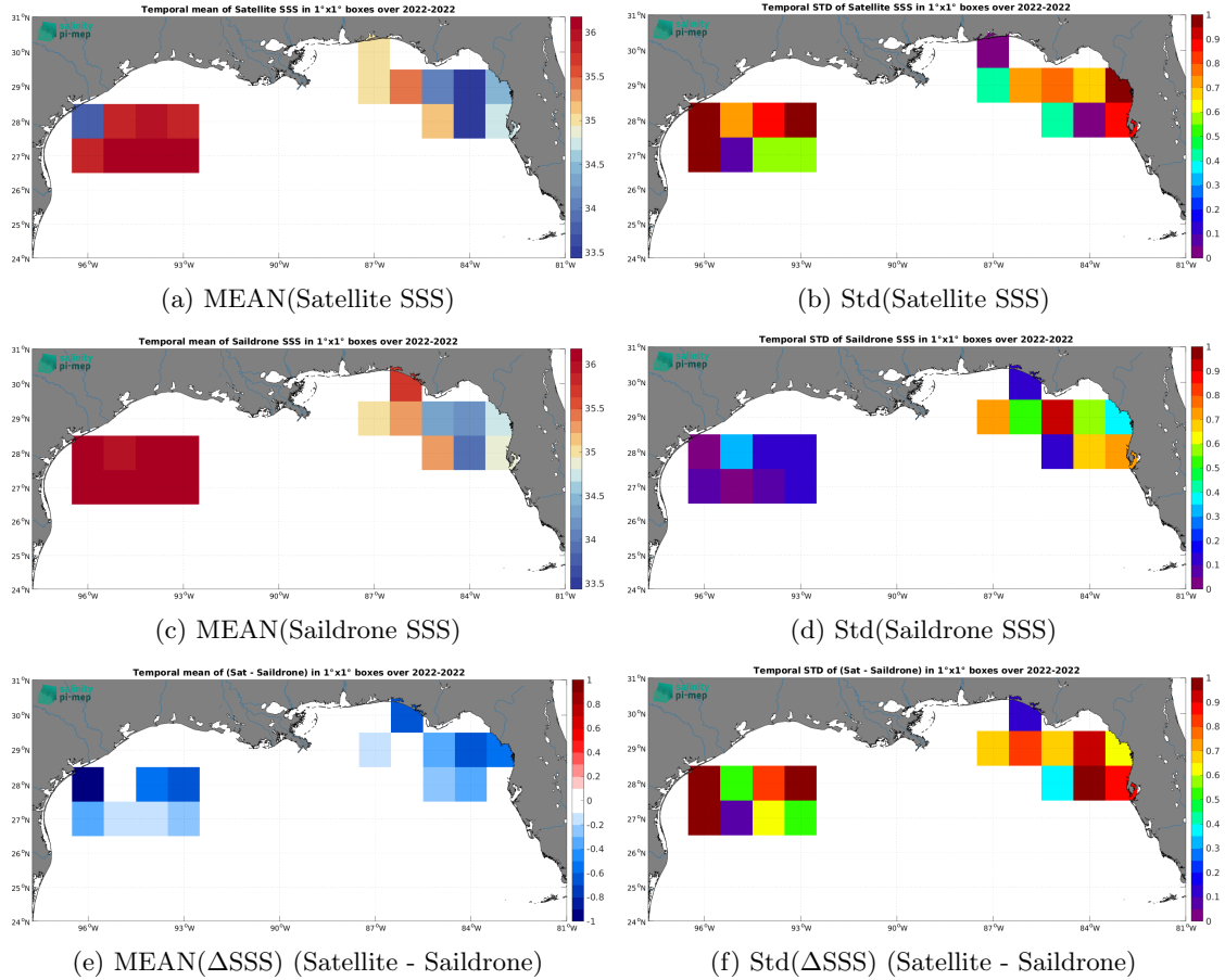
Figure 6: Temporal mean (left) and Std (right) of SSS from SMOS SSS L2Q v331 - No FLAG (CMEMS-CATDS-CPDC) (top), Sairdrone (middle), and of \Delta SSS (Satellite - Sairdrone). Only match-up pairs are used to generate these maps.
