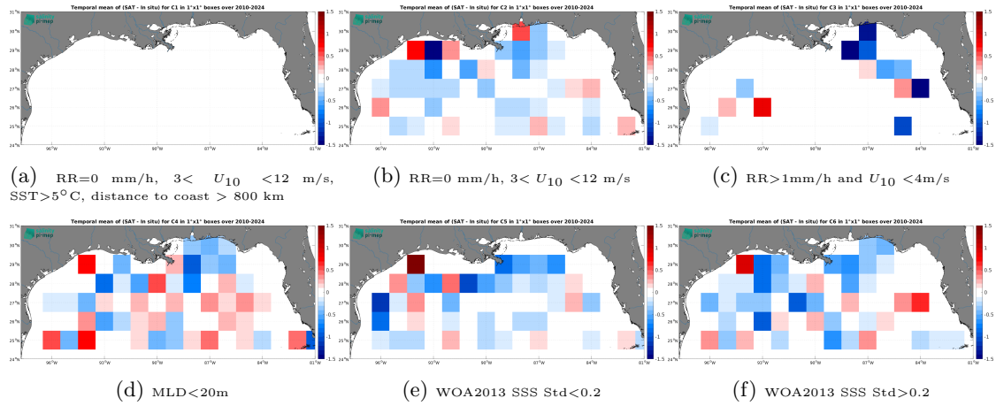
Figure 14: Temporal mean gridded over spatial boxes of size 1^\circ \times 1^\circ of \Delta SSS (SMOS SSS L2Q v331 - No FLAG (CMEMS-CATDS-CPDC) - Argo) for 6 different subdatasets corresponding to:RR=0 mm/h, 3 < U_{10} < 12 m/s, SST >5^\circ C, distance to coast > 800 km (a), RR=0 mm/h, 3 < U_{10} < 12 m/s (b), RR >1 mm/h and U_{10} < 4 m/s (c),MLD <20 m (d),WOA2013 SSS Std <0.2 (e),WOA2013 SSS Std >0.2 (f).
