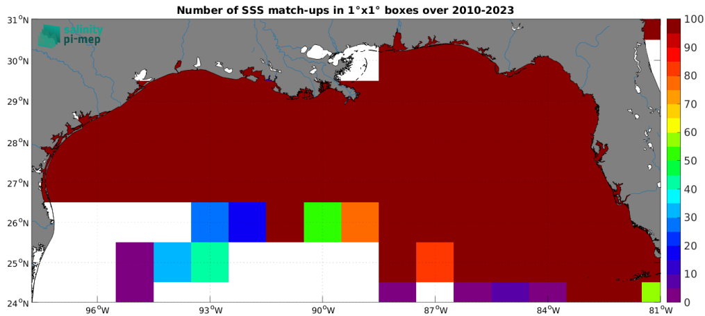
Figure 5: Number of SSS match-ups between TSG (SAMOS) SSS and the SMOS SSS L3 v9 - 9 Days (CATDS-CEC-LOCEAN) SSS product for the Mississippi river plume Pi-MEP region over 1^\circ \times 1^\circ boxes and for the full satellite product period.
