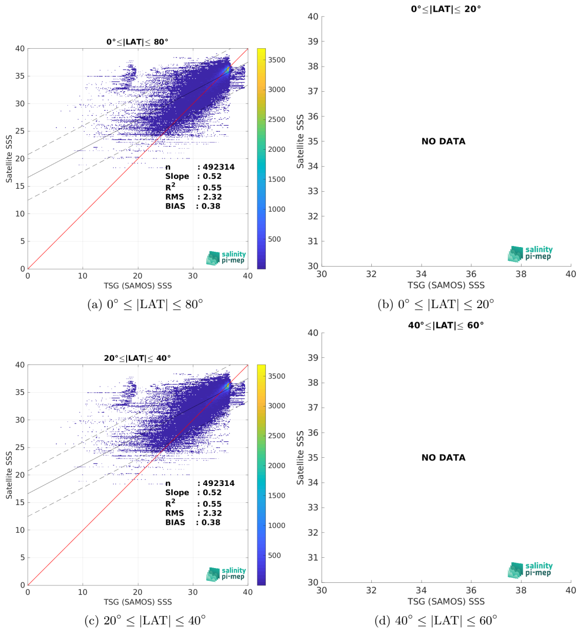
Figure 10: Contour maps of the concentration of SMOS SSS L3 v9 - 9 Days (CATDS-CEC-LOCEAN) SSS (y-axis) versus TSG (SAMOS) SSS (x-axis) at match-up pairs for different latitude bands. For each plot, the red line shows x=y . The black thin and dashed lines indicate a linear fit through the data cloud and the \pm 95\% confidence levels, respectively. The number match-up pairs n , the slope and R^2 coefficient of the linear fit, the root mean square (RMS) and the mean bias between satellite and in situ data are indicated for each latitude band in each plots.
