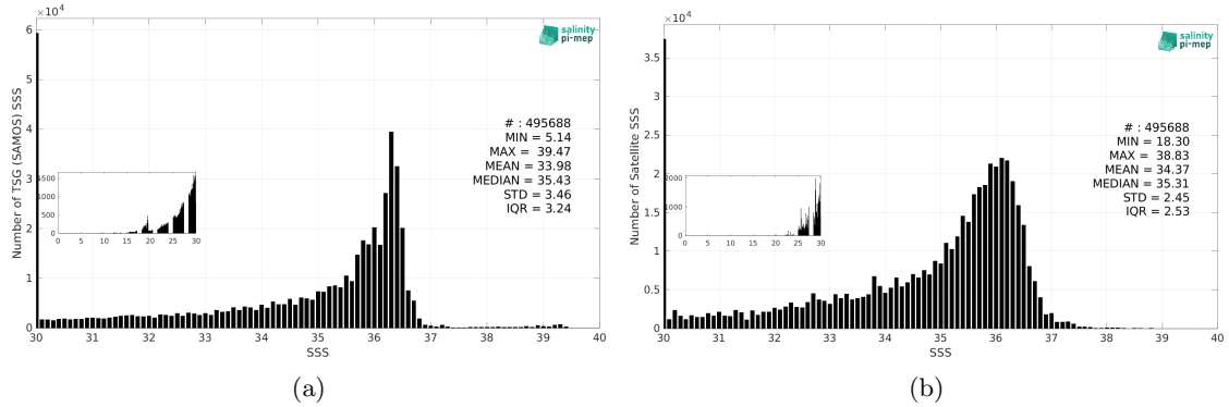
Figure 2: Histograms of SSS from TSG (SAMOS) (a) and SMOS SSS L3 v9 - 9 Days (CATDS-CEC-LOCEAN) (b) considering all match-up pairs per bins of 0.1 over the Mississippi river plume Pi-MEP region and for the full satellite product period.
