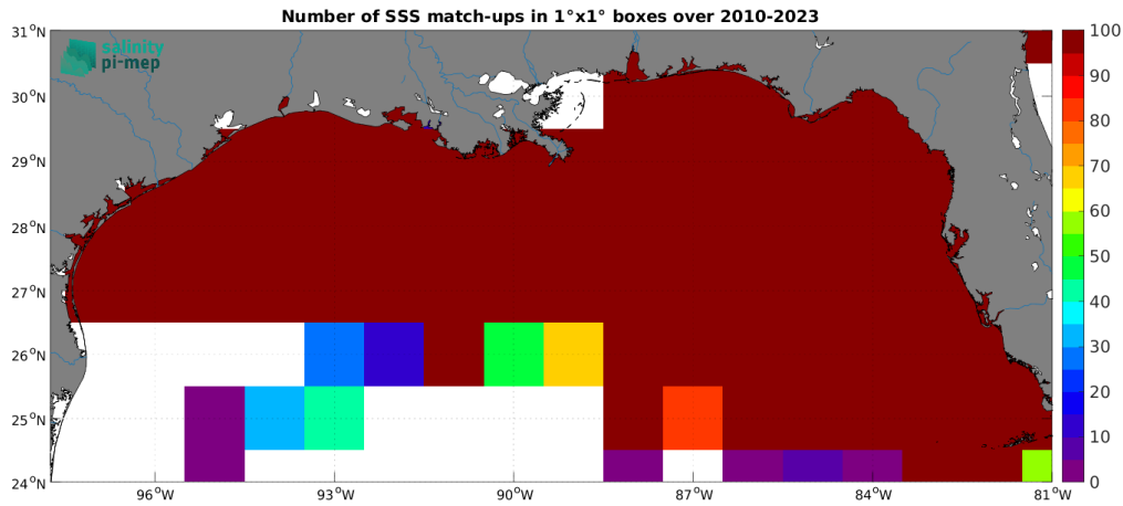
Figure 4: Number of SSS match-ups between TSG (SAMOS) SSS and the SMOS SSS L3 v9 - 9 Days (CATDS-CEC-LOCEAN) SSS product for the Mississippi river plume Pi-MEP region over 1^\circ \times 1^\circ boxes and for the full satellite product period.
