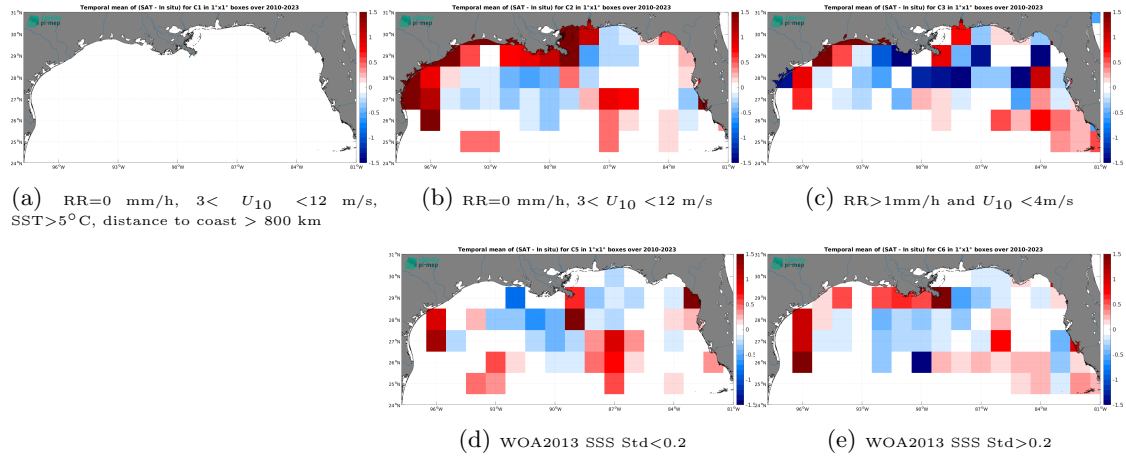
Figure 12: Temporal mean gridded over spatial boxes of size 1^{\circ}\times 1^{\circ} of \Delta\text{SSS} (SMOS SSS L3 v9 - 9 Days (CATDS-CEC-LOCEAN) - TSG (SAMOS)) for 5 different subdatasets corresponding to:RR=0 mm/h, 3 < U_{10} < 12 m/s, SST >5^{\circ}\text{C} , distance to coast > 800 km (a), RR=0 mm/h, 3 < U_{10} < 12 m/s (b), RR >1 mm/h and U_{10} < 4 m/s (c), WOA2013 SSS Std <0.2 (d), WOA2013 SSS Std >0.2 (e).
