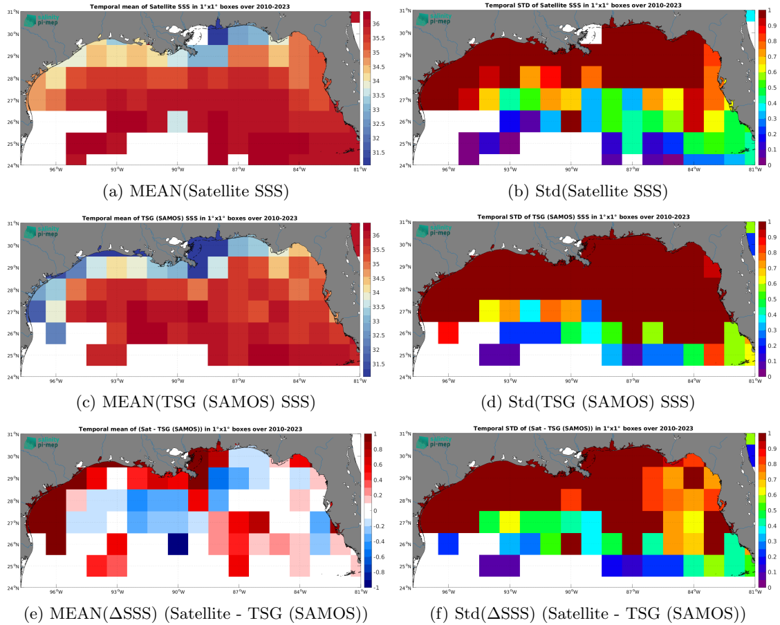
Figure 6: Temporal mean (left) and Std (right) of SSS from SMOS SSS L3 v9 - 9 Days (CATDS-CEC-LOCEAN) (top), TSG (SAMOS) (middle), and of \Delta\text{SSS} (Satellite - TSG (SAMOS)). Only match-up pairs are used to generate these maps.
