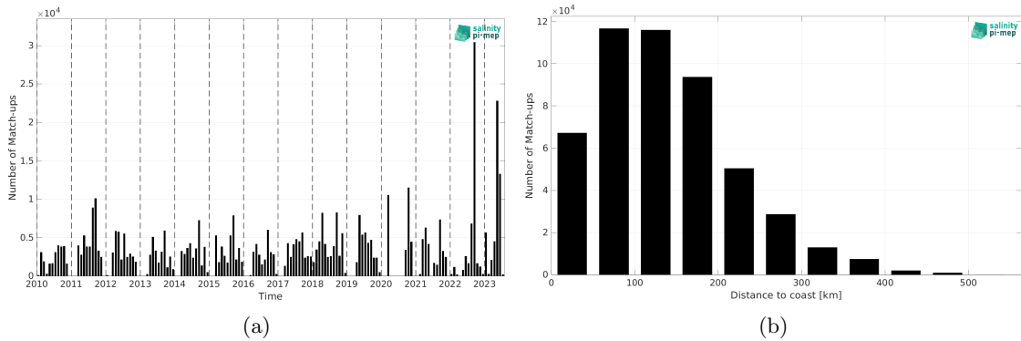
Figure 1: Number of match-ups between TSG (SAMOS) and SMOS SSS L3 v9 - 9 Days (CATDS-CEC-LOCEAN) SSS as a function of time (a) and as function of the distance to coast (b) over the Mississippi river plume Pi-MEP region and for the full satellite product period.
