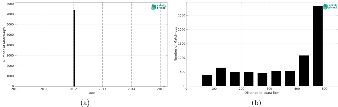
Figure 2: Number of match-ups between TSG (GOSUD-Sailing-ship) and SMOS SSS L3 v9 - 9 Days (CATDS-CEC-LOCEAN) SSS as a function of time (a) and as function of the distance to coast (b) over the Mississippi river plume Pi-MEP region and for the full satellite product period.
