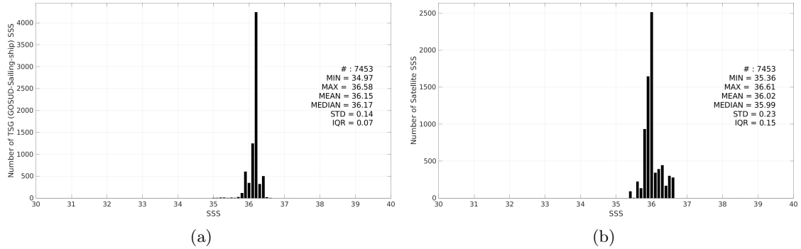
Figure 3: Histograms of SSS from TSG (GOSUD-Sailing-ship) (a) and SMOS SSS L3 v9 - 9 Days (CATDS-CEC-LOCEAN) (b) considering all match-up pairs per bins of 0.1 over the Mississippi river plume Pi-MEP region and for the full satellite product period.
