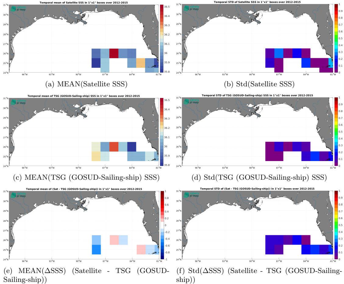
Figure 7: Temporal mean (left) and Std (right) of SSS from SMOS SSS L3 v9 - 9 Days (CATDS-CEC-LOCEAN) (top), TSG (GOSUD-Sailing-ship) (middle), and of \Delta\text{SSS} (Satellite - TSG (GOSUD-Sailing-ship)). Only match-up pairs are used to generate these maps.
