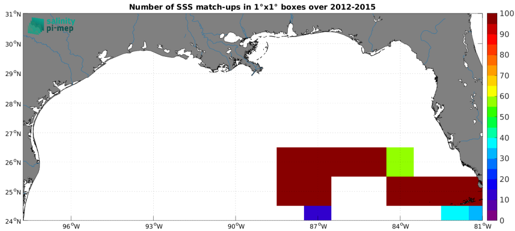
Figure 4: Number of SSS match-ups between TSG (GOSUD-Sailing-ship) SSS and the SMOS SSS L3 v9 - 9 Days (CATDS-CEC-LOCEAN) SSS product for the Mississippi river plume Pi-MEP region over 1^\circ \times 1^\circ boxes and for the full satellite product period.
