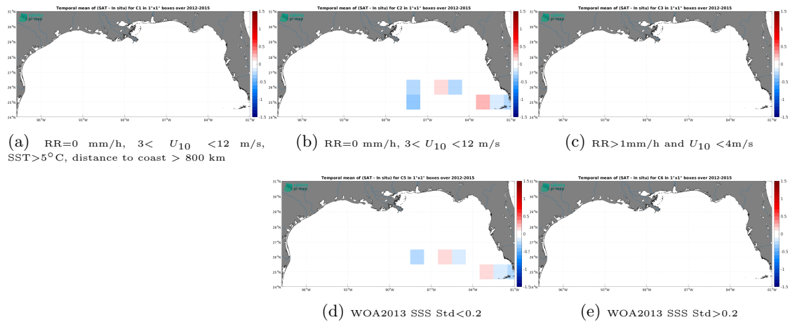
Figure 12: Temporal mean gridded over spatial boxes of size 1^{\circ}\times 1^{\circ} of \Delta SSS (SMOS SSS L3 v9 - 9 Days (CATDS-CEC-LOCEAN) - TSG (GOSUD-Sailing-ship)) for 5 different subdatasets corresponding to:RR=0 mm/h, 3 < U_{10} < 12 m/s, SST >5^{\circ}\text{C} , distance to coast > 800 km (a), RR=0 mm/h, 3 < U_{10} < 12 m/s (b), RR >1 mm/h and U_{10} < 4 m/s (c), WOA2013 SSS Std <0.2 (d), WOA2013 SSS Std >0.2 (e).
