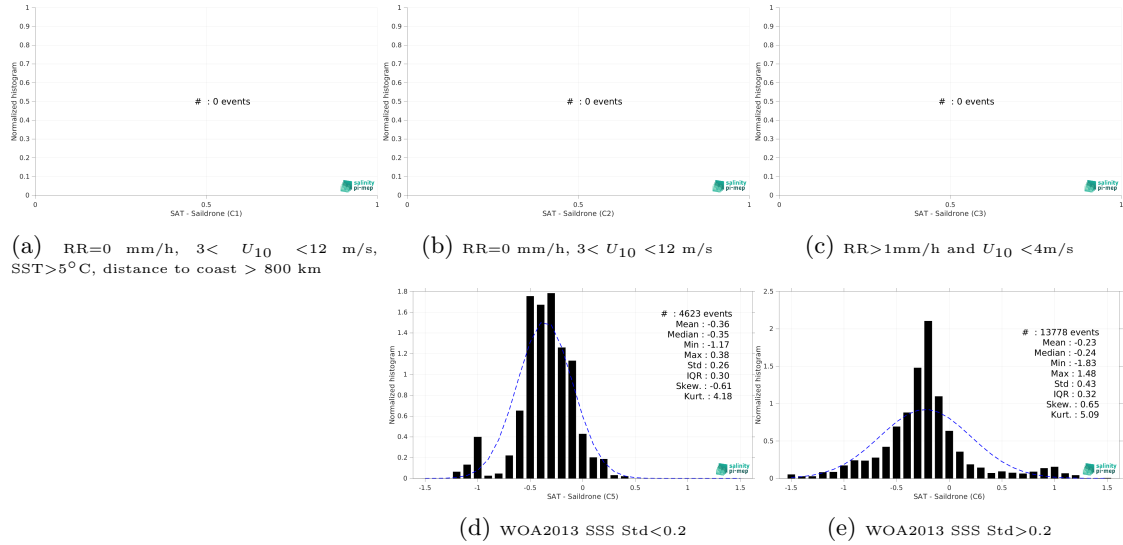
Figure 15: Normalized histogram of \Delta SSS (SMOS SSS L3 v9 - 9 Days (CATDS-CEC-LOCEAN) - Saildrone) for 5 different subdatasets corresponding to: RR=0 mm/h, 3 < U_{10} < 12 m/s, SST >5^{\circ} C, distance to coast > 800 km (a), RR=0 mm/h, 3 < U_{10} < 12 m/s (b), RR >1 mm/h and U_{10} < 4 m/s (c), WOA2013 SSS Std <0.2 (d), WOA2013 SSS Std >0.2 (e).
