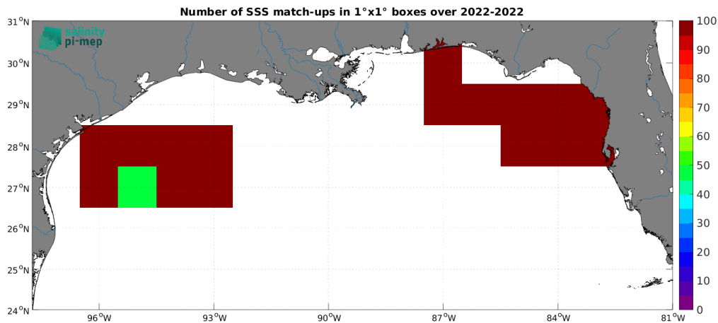
Figure 5: Number of SSS match-ups between Saildrone SSS and the SMOS SSS L3 v9 - 9 Days (CATDS-CEC-LOCEAN) SSS product for the Mississippi river plume Pi-MEP region over 1^\circ \times 1^\circ boxes and for the full satellite product period.
