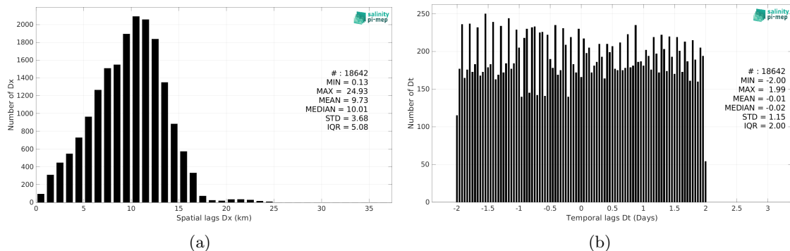
Figure 6: Histograms of the spatial (a) and temporal (b) lags between the location/time of the Saildrone measurement and the date of the corresponding SMOS SSS L3 v9 - 9 Days (CATDS-CEC-LOCEAN) SSS pixel.
