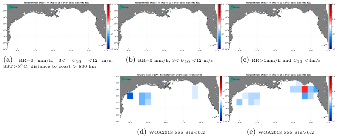
Figure 14: Temporal mean gridded over spatial boxes of size 1^\circ \times 1^\circ of \Delta SSS (SMOS SSS L3 v9 - 9 Days (CATDS-CEC-LOCEAN) - Saildrone) for 5 different subdatasets corresponding to: RR=0 mm/h, 3 < U_{10} < 12 m/s, SST > 5°C, distance to coast > 800 km (a), RR=0 mm/h, 3 < U_{10} < 12 m/s (b), RR > 1 mm/h and U_{10} < 4 m/s (c), WOA2013 SSS Std < 0.2 (d), WOA2013 SSS Std > 0.2 (e).
