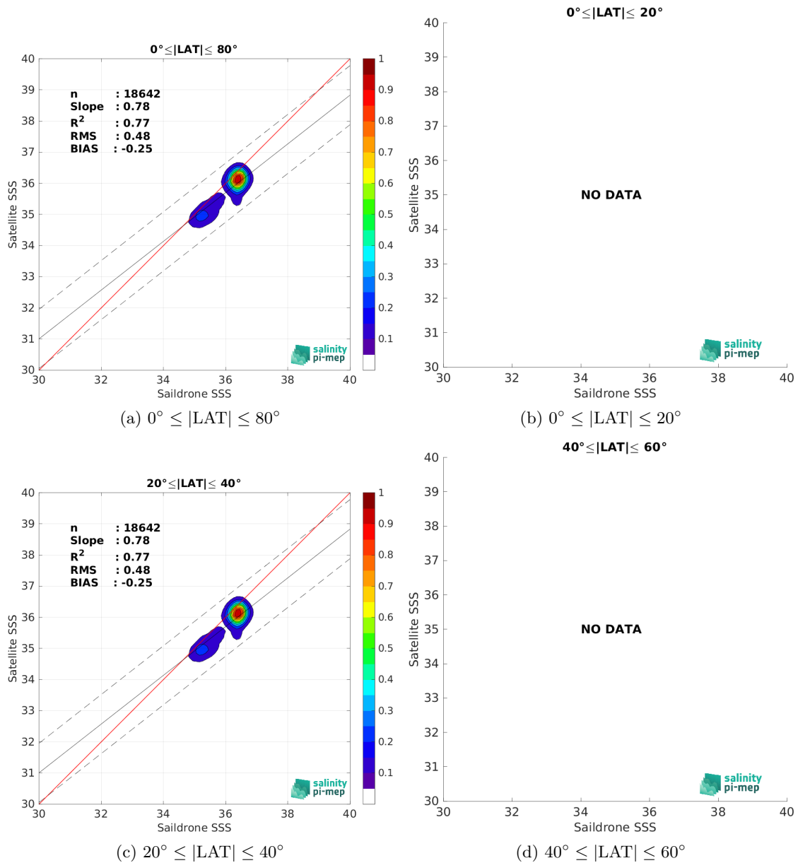
Figure 10: Contour maps of the concentration of SMOS SSS L3 v9 - 9 Days (CATDS-CEC-LOCEAN) SSS (y-axis) versus Saïdrone SSS (x-axis) at match-up pairs for different latitude bands. For each plot, the red line shows x=y . The black thin and dashed lines indicate a linear fit through the data cloud and the \pm 95\% confidence levels, respectively. The number match-up pairs n , the slope and R^2 coefficient of the linear fit, the root mean square (RMS) and the mean bias between satellite and in situ data are indicated for each latitude band in each plots.
