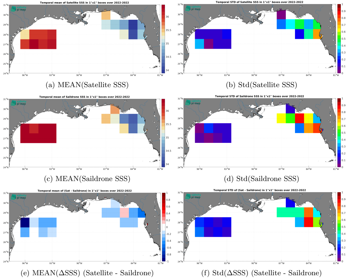
Figure 7: Temporal mean (left) and Std (right) of SSS from SMOS SSS L3 v9 - 9 Days (CATDS-CEC-LOCEAN) (top), Sairdrone (middle), and of \Delta SSS (Satellite - Sairdrone). Only match-up pairs are used to generate these maps.
