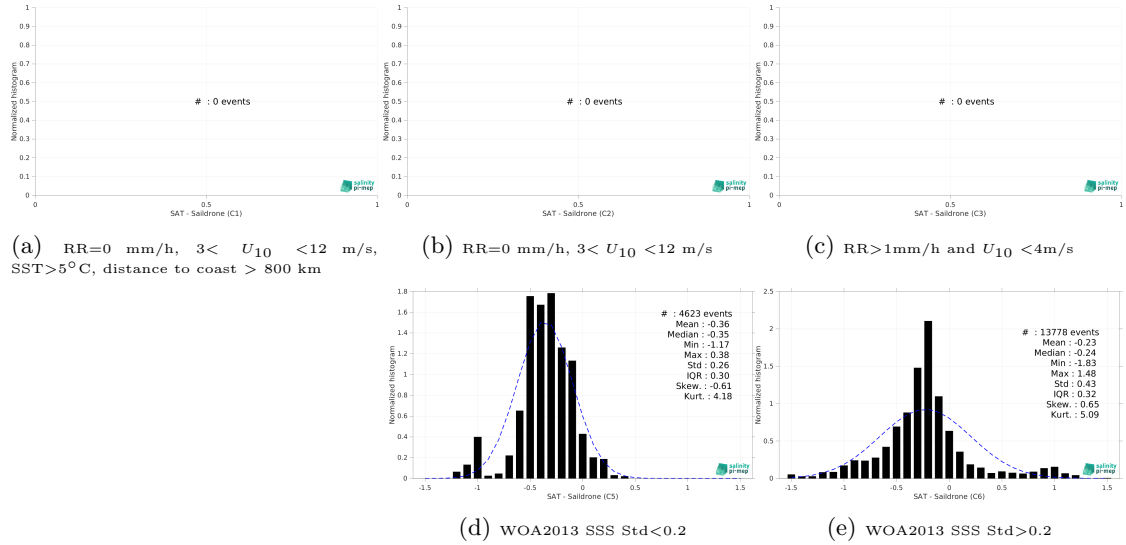
Figure 15: Normalized histogram of \Delta SSS (SMOS SSS L3 v9 - 9 Days (CATDS-CEC-LOCEAN) - Saildrone) for 5 different subdatasets corresponding to: RR=0 mm/h, 3 < U_{10} < 12 m/s, SST >5^{\circ}\text{C} , distance to coast > 800 km (a), RR=0 mm/h, 3 < U_{10} < 12 m/s (b), RR >1 mm/h and U_{10} < 4 m/s (c), WOA2013 SSS Std <0.2 (d), WOA2013 SSS Std >0.2 (e).
