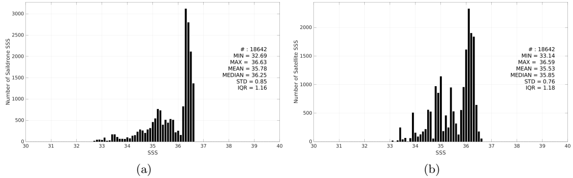
Figure 2: Histograms of SSS from Saildrone (a) and SMOS SSS L3 v9 - 9 Days (CATDS-CEC-LOCEAN) (b) considering all match-up pairs per bins of 0.1 over the Mississippi river plume Pi-MEP region and for the full satellite product period.
