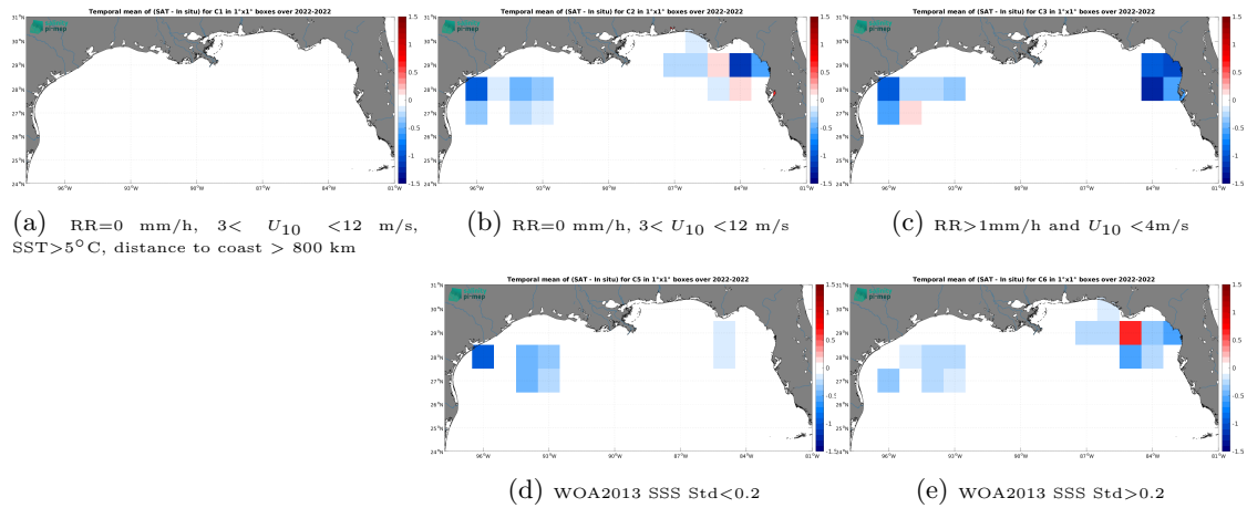
Figure 12: Temporal mean gridded over spatial boxes of size 1^{\circ}\times 1^{\circ} of \Delta\text{SSS} (SMOS SSS L3 v9 - 9 Days (CATDS-CEC-LOCEAN) - Saildrone) for 5 different subdatasets corresponding to:RR=0 mm/h, 3 < U_{10} < 12 m/s, SST >5^{\circ}\text{C} , distance to coast > 800 km (a), RR=0 mm/h, 3 < U_{10} < 12 m/s (b), RR >1 mm/h and U_{10} < 4 m/s (c), WOA2013 SSS Std <0.2 (d), WOA2013 SSS Std >0.2 (e).
