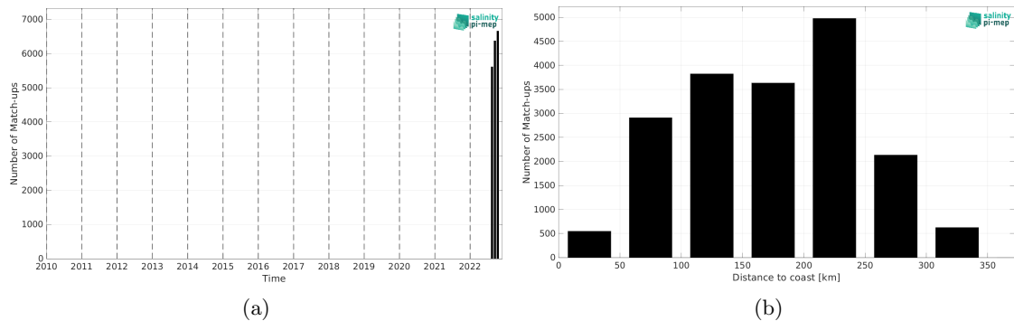
Figure 1: Number of match-ups between Saildrone and SMOS SSS L3 v9 - 9 Days (CATDS-CEC-LOCEAN) SSS as a function of time (a) and as function of the distance to coast (b) over the Mississippi river plume Pi-MEP region and for the full satellite product period.
