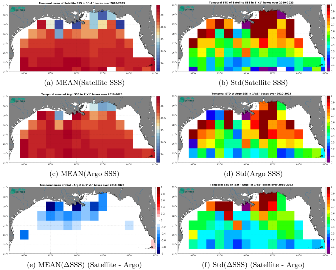
Figure 7: Temporal mean (left) and Std (right) of SSS from SMOS SSS L3 v9 - 9 Days (CATDS-CEC-LOCEAN) (top), Argo (middle), and of \Delta SSS (Satellite - Argo). Only match-up pairs are used to generate these maps.
