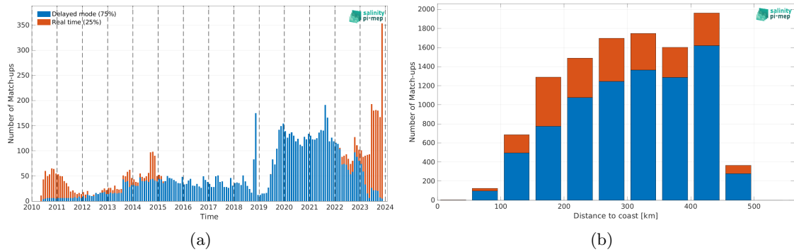
Figure 2: Number of match-ups between Argo and SMOS SSS L3 v9 - 9 Days (CATDS-CEC-LOCEAN) SSS as a function of time (a) and as function of the distance to coast (b) over the Mississippi river plume Pi-MEP region and for the full satellite product period.
