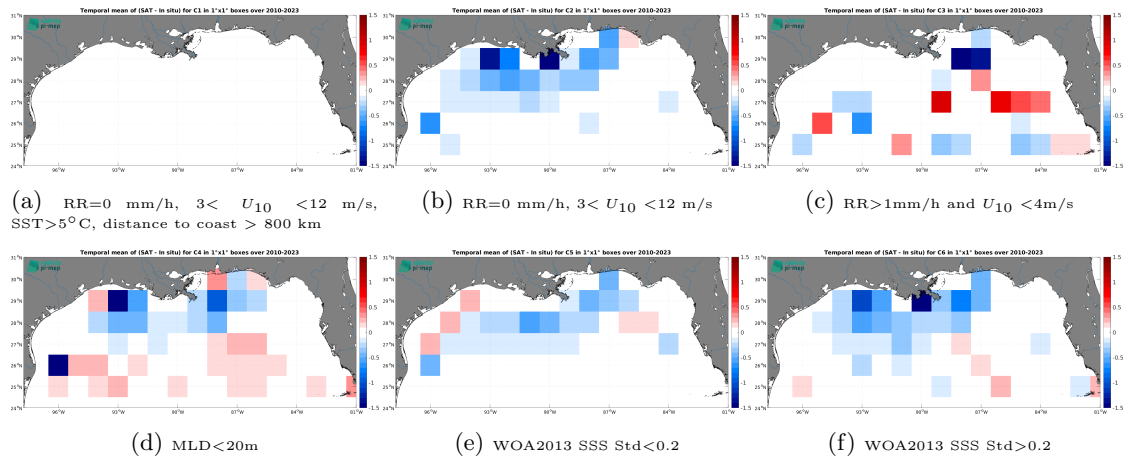
Figure 14: Temporal mean gridded over spatial boxes of size 1^\circ \times 1^\circ of \Delta SSS (SMOS SSS L3 v9 - 9 Days (CATDS-CEC-LOCEAN) - Argo) for 6 different subdatasets corresponding to: RR=0 mm/h, 3 < U_{10} < 12 m/s, SST > 5^\circ\text{C} , distance to coast > 800 km (a), RR=0 mm/h, 3 < U_{10} < 12 m/s (b), RR > 1 mm/h and U_{10} < 4 m/s (c), MLD < 20 m (d), WOA2013 SSS Std < 0.2 (e), WOA2013 SSS Std > 0.2 (f).
