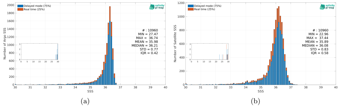
Figure 3: Histograms of SSS from Argo (a) and SMOS SSS L3 v9 - 9 Days (CATDS-CEC-LOCEAN) (b) considering all match-up pairs per bins of 0.1 over the Mississippi river plume Pi-MEP region and for the full satellite product period.
