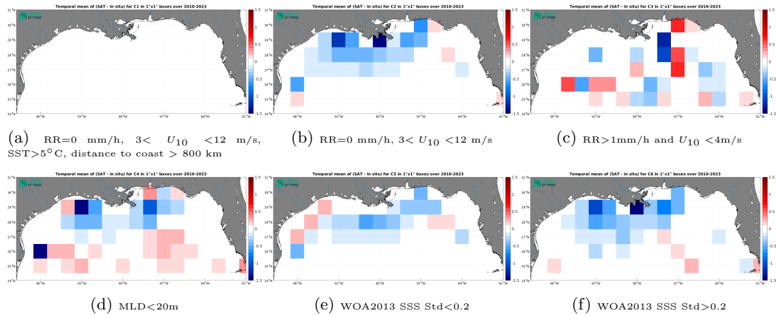
Figure 12: Temporal mean gridded over spatial boxes of size 1^{\circ}\times 1^{\circ} of \Delta\text{SSS} (SMOS SSS L3 v9 - 9 Days (CATDS-CEC-LOCEAN) - Argo) for 6 different subdatasets corresponding to:RR=0 mm/h, 3 < U_{10} < 12 m/s, SST > 5^{\circ}\text{C} , distance to coast > 800 km (a), RR=0 mm/h, 3 < U_{10} < 12 m/s (b), RR > 1\text{mm/h} and U_{10} < 4\text{m/s} (c),MLD < 20\text{m} (d),WOA2013 SSS Std < 0.2 (e),WOA2013 SSS Std > 0.2 (f).
