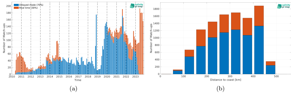
Figure 1: Number of match-ups between Argo and SMOS SSS L3 v9 - 9 Days (CATDS-CEC-LOCEAN) SSS as a function of time (a) and as function of the distance to coast (b) over the Mississippi river plume Pi-MEP region and for the full satellite product period.
