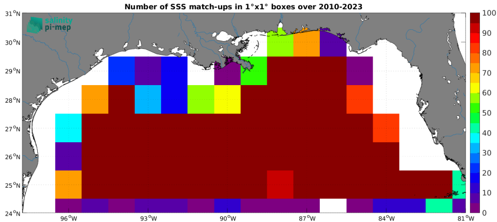
Figure 4: Number of SSS match-ups between Argo SSS and the SMOS SSS L3 v9 - 9 Days (CATDS-CEC-LOCEAN) SSS product for the Mississippi river plume Pi-MEP region over 1^\circ \times 1^\circ boxes and for the full satellite product period.
