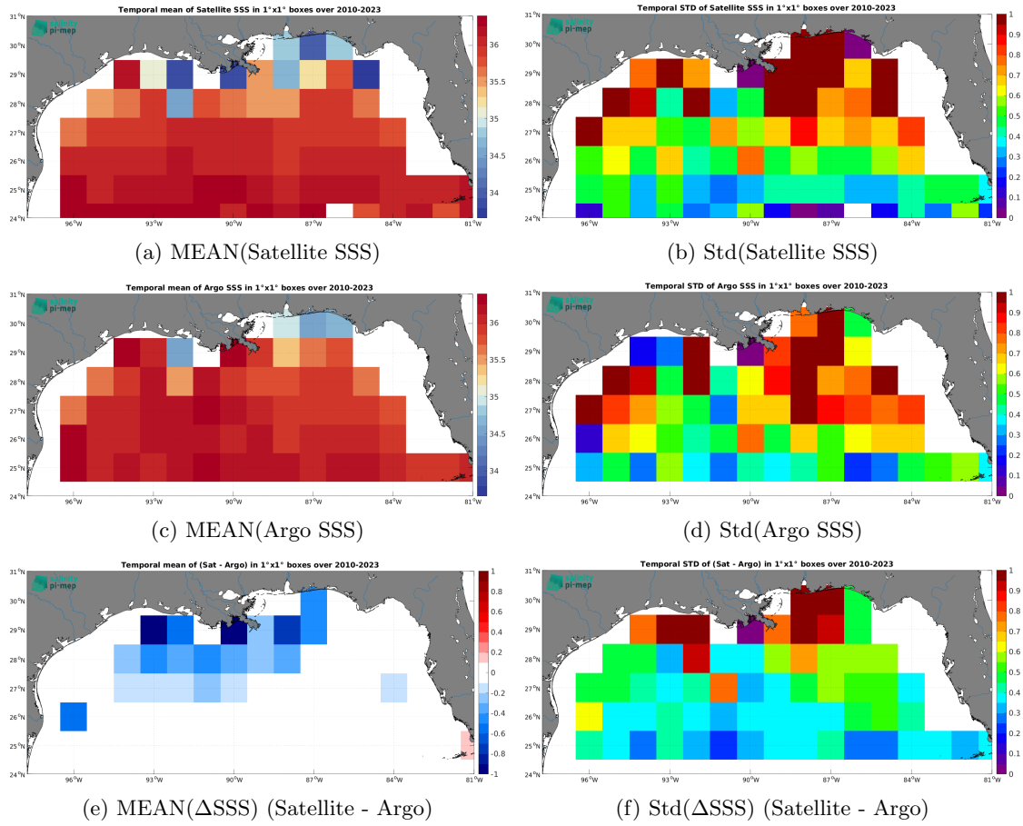
Figure 6: Temporal mean (left) and Std (right) of SSS from SMOS SSS L3 v9 - 9 Days (CATDS-CEC-LOCEAN) (top), Argo (middle), and of \Delta SSS (Satellite - Argo). Only match-up pairs are used to generate these maps.
