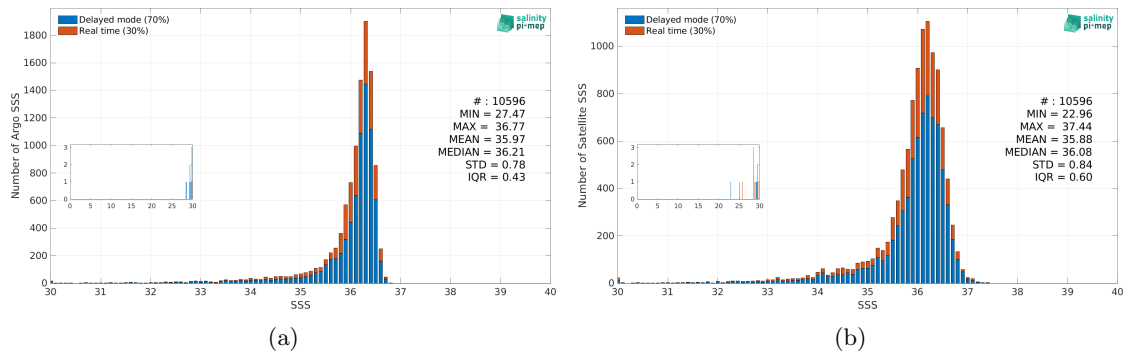
Figure 2: Histograms of SSS from Argo (a) and SMOS SSS L3 v9 - 9 Days (CATDS-CEC-LOCEAN) (b) considering all match-up pairs per bins of 0.1 over the Mississippi river plume Pi-MEP region and for the full satellite product period.
