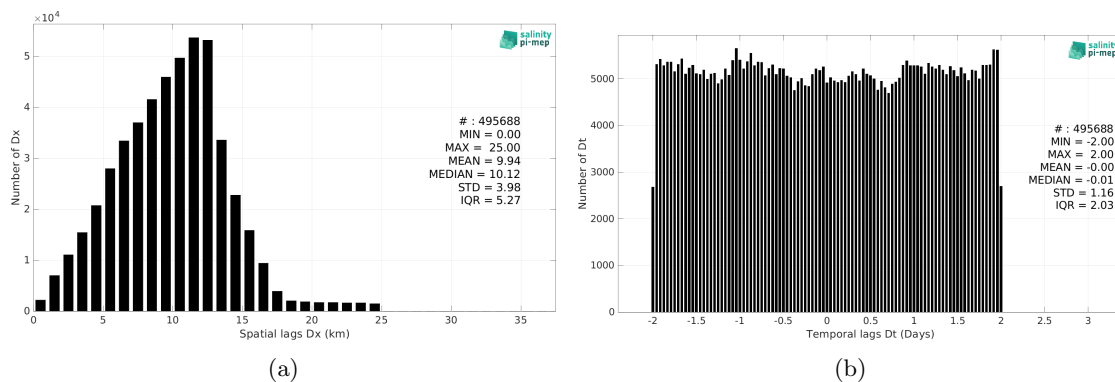
Figure 5: Histograms of the spatial (a) and temporal (b) lags between the location/time of the TSG (SAMOS) measurement and the date of the corresponding SMOS SSS L3 v9 - 18 Days (CATDS-CEC-LOCEAN) SSS pixel.
