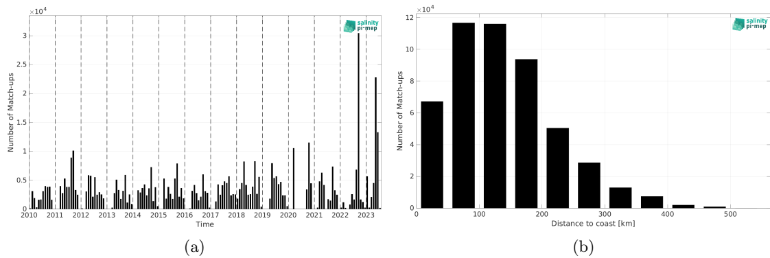
Figure 1: Number of match-ups between TSG (SAMOS) and SMOS SSS L3 v9 - 18 Days (CATDS-CEC-LOCEAN) SSS as a function of time (a) and as function of the distance to coast (b) over the Mississippi river plume Pi-MEP region and for the full satellite product period.
