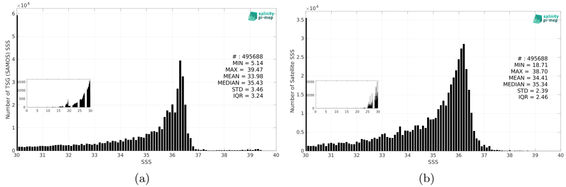
Figure 2: Histograms of SSS from TSG (SAMOS) (a) and SMOS SSS L3 v9 - 18 Days (CATDS-CEC-LOCEAN) (b) considering all match-up pairs per bins of 0.1 over the Mississippi river plume Pi-MEP region and for the full satellite product period.
