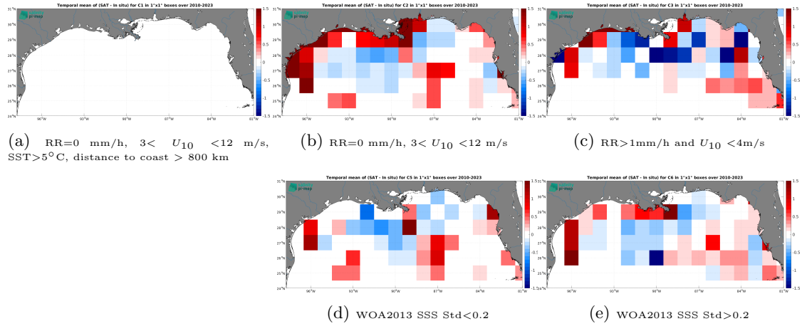
Figure 12: Temporal mean gridded over spatial boxes of size 1^{\circ}\times 1^{\circ} of \Delta\text{SSS} (SMOS SSS L3 v9 - 18 Days (CATDS-CEC-LOCEAN) - TSG (SAMOS)) for 5 different subdatasets corresponding to:RR=0 mm/h, 3 < U_{10} < 12 m/s, SST >5^{\circ}\text{C} , distance to coast > 800 km (a), RR=0 mm/h, 3 < U_{10} < 12 m/s (b), RR >1 mm/h and U_{10} < 4 m/s (c), WOA2013 SSS Std <0.2 (d), WOA2013 SSS Std >0.2 (e).
