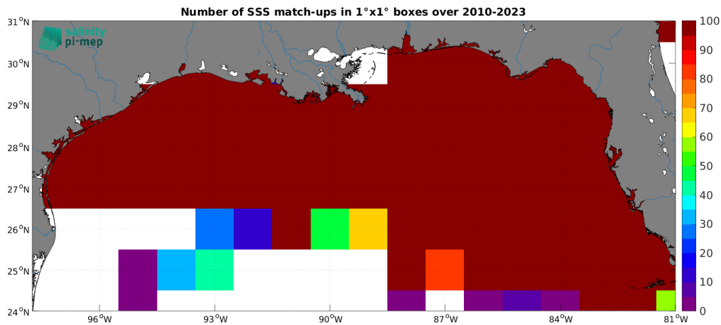
Figure 4: Number of SSS match-ups between TSG (SAMOS) SSS and the SMOS SSS L3 v9 - 18 Days (CATDS-CEC-LOCEAN) SSS product for the Mississippi river plume Pi-MEP region over 1^\circ \times 1^\circ boxes and for the full satellite product period.
