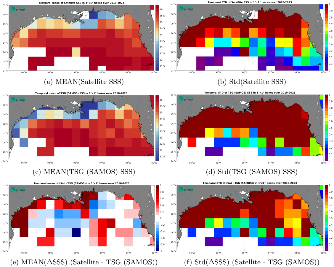
Figure 6: Temporal mean (left) and Std (right) of SSS from SMOS SSS L3 v9 - 18 Days (CATDS-CEC-LOCEAN) (top), TSG (SAMOS) (middle), and of \Delta\text{SSS} (Satellite - TSG (SAMOS)). Only match-up pairs are used to generate these maps.
