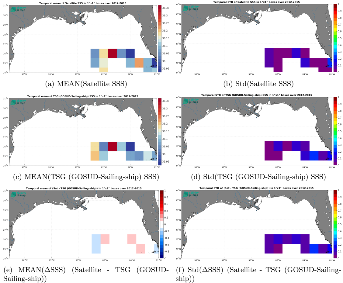
Figure 7: Temporal mean (left) and Std (right) of SSS from SMOS SSS L3 v9 - 18 Days (CATDS-CEC-LOCEAN) (top), TSG (GOSUD-Sailing-ship) (middle), and of \Delta\text{SSS} (Satellite - TSG (GOSUD-Sailing-ship)). Only match-up pairs are used to generate these maps.
