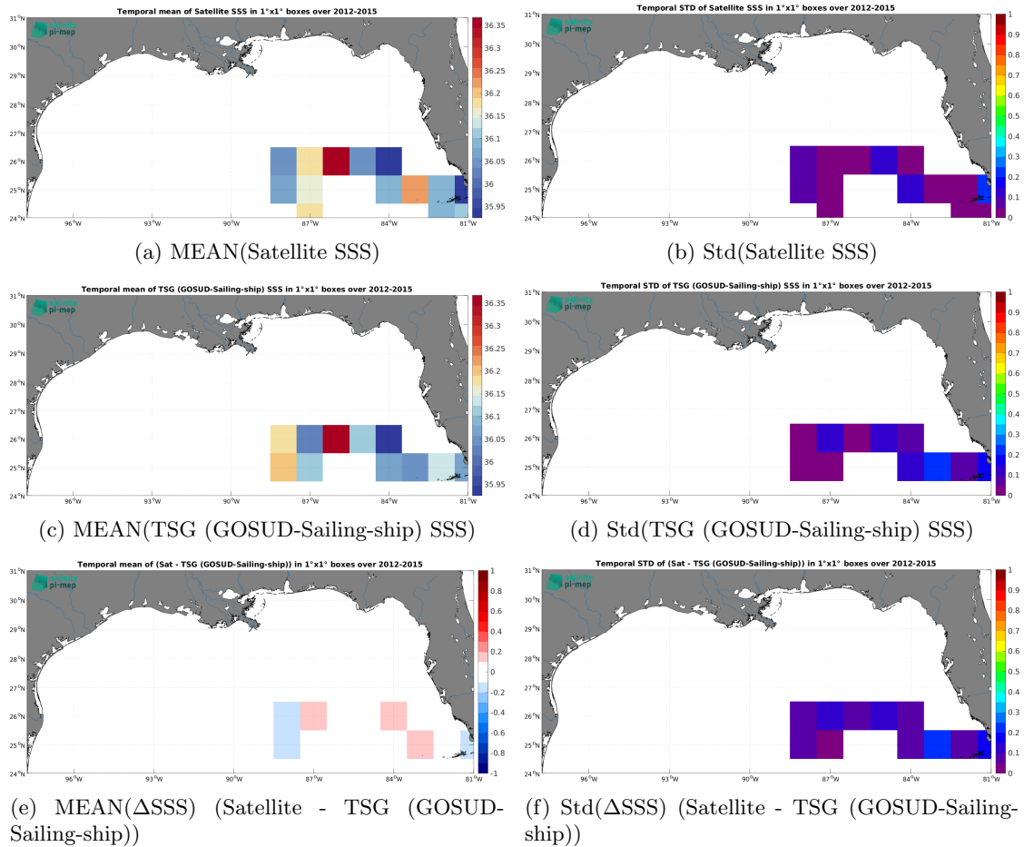
Figure 6: Temporal mean (left) and Std (right) of SSS from SMOS SSS L3 v9 - 18 Days (CATDS-CEC-LOCEAN) (top), TSG (GOSUD-Sailing-ship) (middle), and of \Delta\text{SSS} (Satellite - TSG (GOSUD-Sailing-ship)). Only match-up pairs are used to generate these maps.
