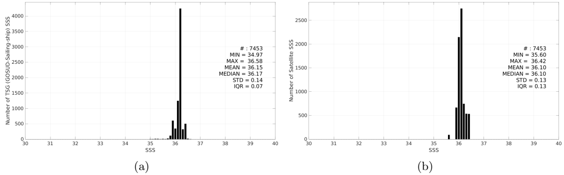
Figure 2: Histograms of SSS from TSG (GOSUD-Sailing-ship) (a) and SMOS SSS L3 v9 - 18 Days (CATDS-CEC-LOCEAN) (b) considering all match-up pairs per bins of 0.1 over the Mississippi river plume Pi-MEP region and for the full satellite product period.
