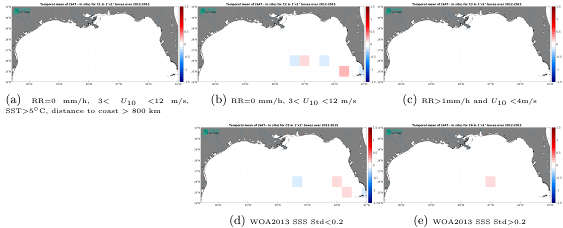
Figure 12: Temporal mean gridded over spatial boxes of size 1^{\circ}\times 1^{\circ} of \Delta SSS (SMOS SSS L3 v9 - 18 Days (CATDS-CEC-LOCEAN) - TSG (GOSUD-Sailing-ship)) for 5 different subdatasets corresponding to:RR=0 mm/h, 3 < U_{10} < 12 m/s, SST >5^{\circ}\text{C} , distance to coast > 800 km (a), RR=0 mm/h, 3 < U_{10} < 12 m/s (b), RR >1 mm/h and U_{10} < 4 m/s (c), WOA2013 SSS Std <0.2 (d), WOA2013 SSS Std >0.2 (e).
