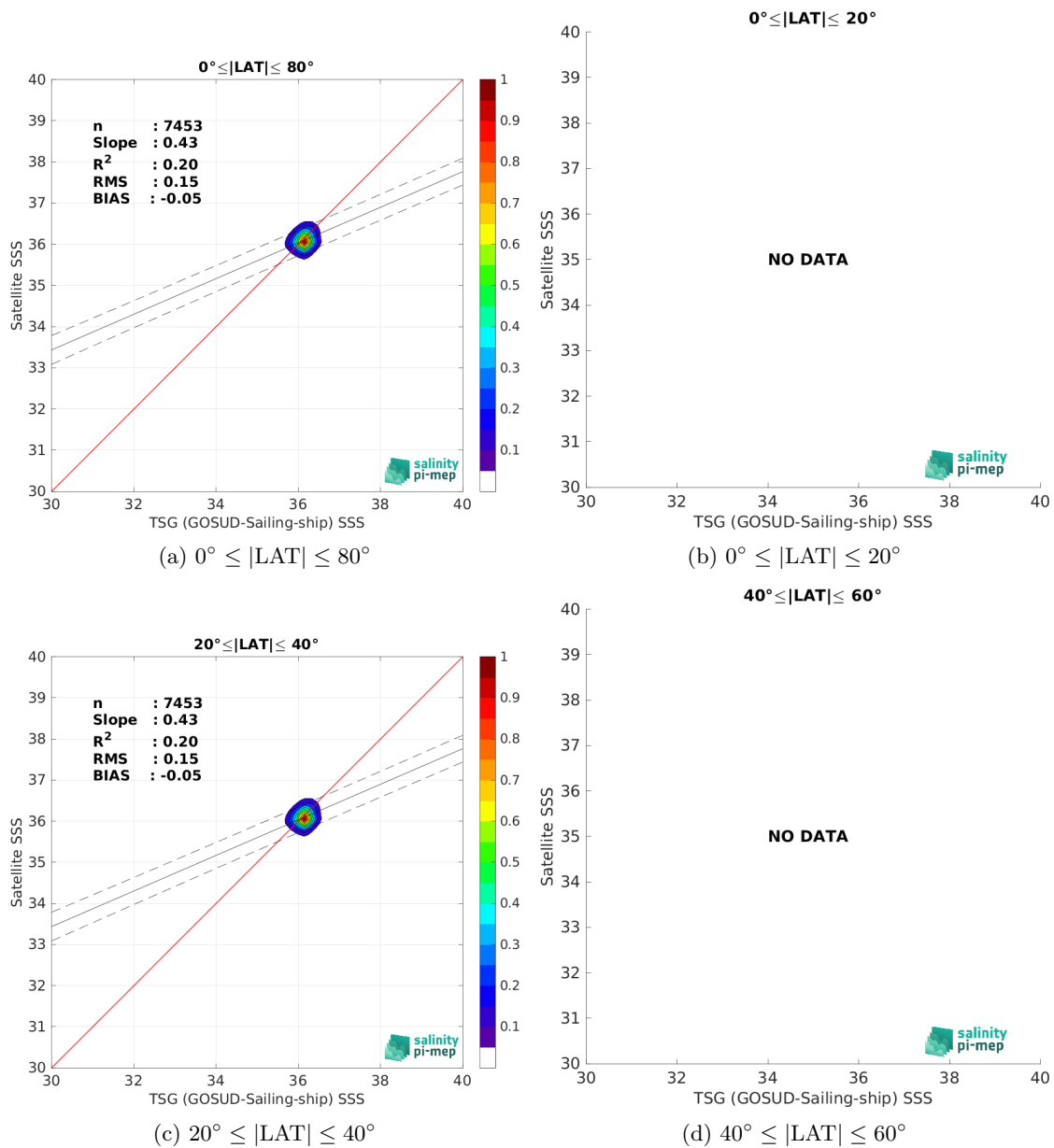
Figure 9: Contour maps of the concentration of SMOS SSS L3 v9 - 18 Days (CATDS-CEC-LOCEAN) SSS (y-axis) versus TSG (GOSUD-Sailing-ship) SSS (x-axis) at match-up pairs for different latitude bands. For each plot, the red line shows x=y . The black thin and dashed lines indicate a linear fit through the data cloud and the \pm 95\% confidence levels, respectively. The number match-up pairs n , the slope and R^2 coefficient of the linear fit, the root mean square (RMS) and the mean bias between satellite and in situ data are indicated for each latitude band in each plots.
