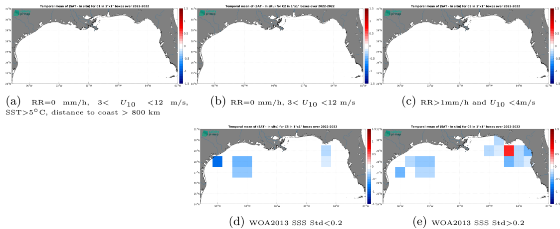
Figure 14: Temporal mean gridded over spatial boxes of size 1^\circ \times 1^\circ of \Delta SSS (SMOS SSS L3 v9 - 18 Days (CATDS-CEC-LOCEAN) - Sailability) for 5 different subdatasets corresponding to: RR=0 mm/h, 3 < U_{10} < 12 m/s, SST > 5°C, distance to coast > 800 km (a), RR=0 mm/h, 3 < U_{10} < 12 m/s (b), RR > 1mm/h and U_{10} < 4 m/s (c), WOA2013 SSS Std < 0.2 (d), WOA2013 SSS Std > 0.2 (e).
