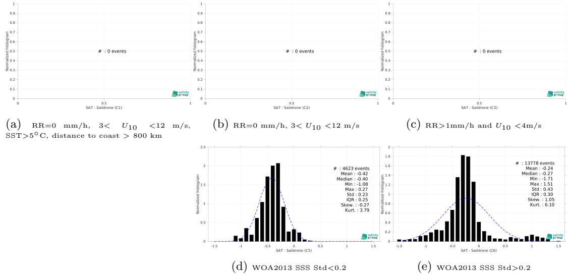
Figure 15: Normalized histogram of \Delta SSS (SMOS SSS L3 v9 - 18 Days (CATDS-CEC-LOCEAN) - Saildrone) for 5 different subdatasets corresponding to: RR=0 mm/h, 3 < U_{10} < 12 m/s, SST >5^{\circ} C, distance to coast > 800 km (a), RR=0 mm/h, 3 < U_{10} < 12 m/s (b), RR >1 mm/h and U_{10} < 4 m/s (c), WOA2013 SSS Std <0.2 (d), WOA2013 SSS Std >0.2 (e).
