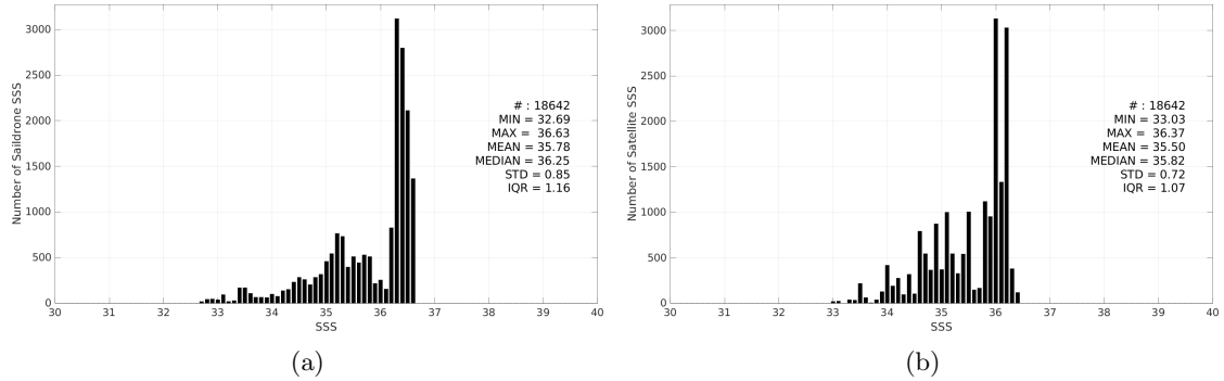
Figure 2: Histograms of SSS from Saildrone (a) and SMOS SSS L3 v9 - 18 Days (CATDS-CEC-LOCEAN) (b) considering all match-up pairs per bins of 0.1 over the Mississippi river plume Pi-MEP region and for the full satellite product period.
