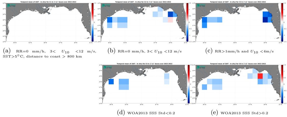
Figure 12: Temporal mean gridded over spatial boxes of size 1^{\circ}\times 1^{\circ} of \Delta\text{SSS} (SMOS SSS L3 v9 - 18 Days (CATDS-CEC-LOCEAN) - Saildrone) for 5 different subdatasets corresponding to:RR=0 mm/h, 3 < U_{10} < 12 m/s, SST >5^{\circ}\text{C} , distance to coast > 800 km (a), RR=0 mm/h, 3 < U_{10} < 12 m/s (b), RR >1 mm/h and U_{10} < 4 m/s (c), WOA2013 SSS Std <0.2 (d), WOA2013 SSS Std >0.2 (e).
