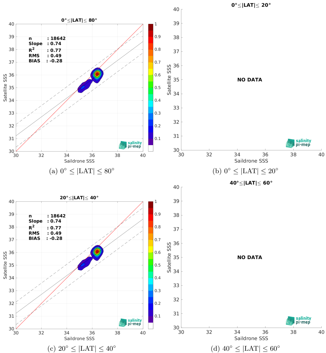
Figure 9: Contour maps of the concentration of SMOS SSS L3 v9 - 18 Days (CATDS-CEC-LOCEAN) SSS (y-axis) versus Saïldrone SSS (x-axis) at match-up pairs for different latitude bands. For each plot, the red line shows x=y . The black thin and dashed lines indicate a linear fit through the data cloud and the \pm 95\% confidence levels, respectively. The number match-up pairs n , the slope and R^2 coefficient of the linear fit, the root mean square (RMS) and the mean bias between satellite and in situ data are indicated for each latitude band in each plots.
