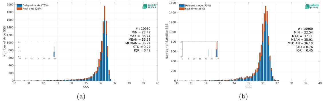
Figure 3: Histograms of SSS from Argo (a) and SMOS SSS L3 v9 - 18 Days (CATDS-CEC-LOCEAN) (b) considering all match-up pairs per bins of 0.1 over the Mississippi river plume Pi-MEP region and for the full satellite product period.
