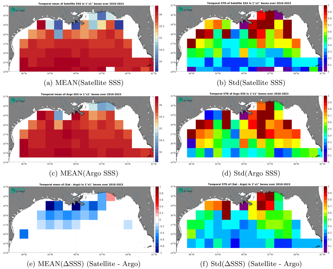
Figure 7: Temporal mean (left) and Std (right) of SSS from SMOS SSS L3 v9 - 18 Days (CATDS-CEC-LOCEAN) (top), Argo (middle), and of \Delta SSS (Satellite - Argo). Only match-up pairs are used to generate these maps.
