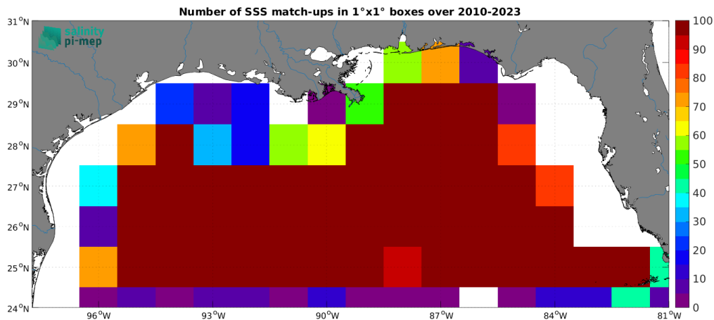
Figure 5: Number of SSS match-ups between Argo SSS and the SMOS SSS L3 v9 - 18 Days (CATDS-CEC-LOCEAN) SSS product for the Mississippi river plume Pi-MEP region over 1^\circ \times 1^\circ boxes and for the full satellite product period.
