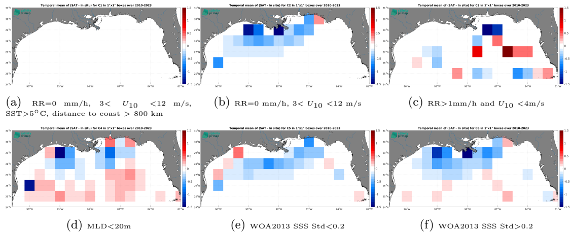
Figure 14: Temporal mean gridded over spatial boxes of size 1^\circ \times 1^\circ of \Delta SSS (SMOS SSS L3 v9 - 18 Days (CATDS-CEC-LOCEAN) - Argo) for 6 different subdatasets corresponding to: RR=0 mm/h, 3 < U_{10} < 12 m/s, SST > 5^\circ\text{C} , distance to coast > 800 km (a), RR=0 mm/h, 3 < U_{10} < 12 m/s (b), RR > 1 mm/h and U_{10} < 4 m/s (c), MLD < 20 m (d), WOA2013 SSS Std < 0.2 (e), WOA2013 SSS Std > 0.2 (f).
