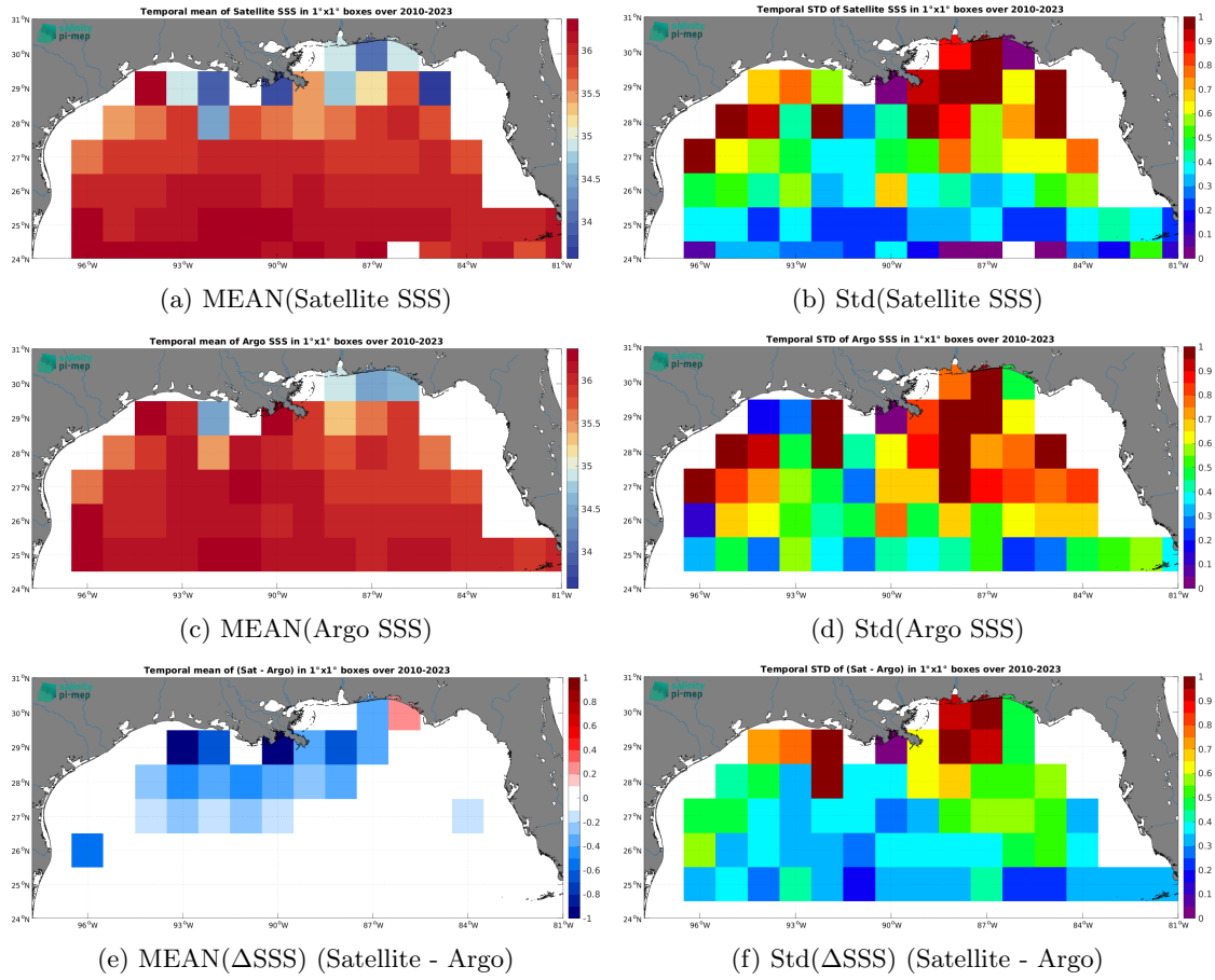
Figure 6: Temporal mean (left) and Std (right) of SSS from SMOS SSS L3 v9 - 18 Days (CATDS-CEC-LOCEAN) (top), Argo (middle), and of \Delta SSS (Satellite - Argo). Only match-up pairs are used to generate these maps.
