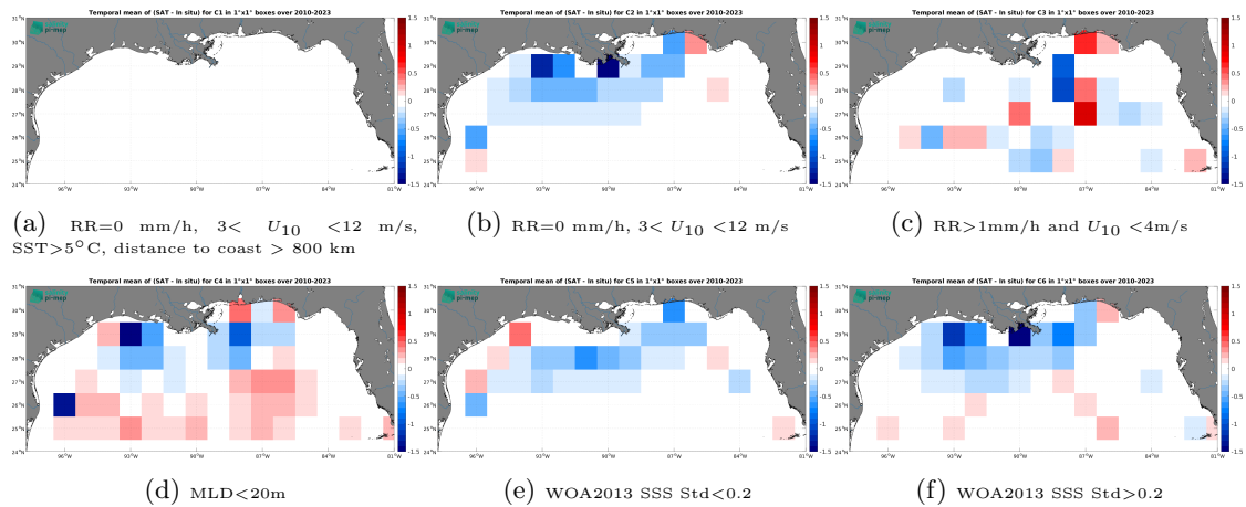
Figure 12: Temporal mean gridded over spatial boxes of size 1^{\circ}\times 1^{\circ} of \Delta\text{SSS} (SMOS SSS L3 v9 - 18 Days (CATDS-CEC-LOCEAN) - Argo) for 6 different subdatasets corresponding to:RR=0 mm/h, 3 < U_{10} < 12 m/s, SST > 5^{\circ}\text{C} , distance to coast > 800 km (a), RR=0 mm/h, 3 < U_{10} < 12 m/s (b), RR > 1\text{mm/h} and U_{10} < 4\text{m/s} (c),MLD < 20\text{m} (d),WOA2013 SSS Std < 0.2 (e),WOA2013 SSS Std > 0.2 (f).
