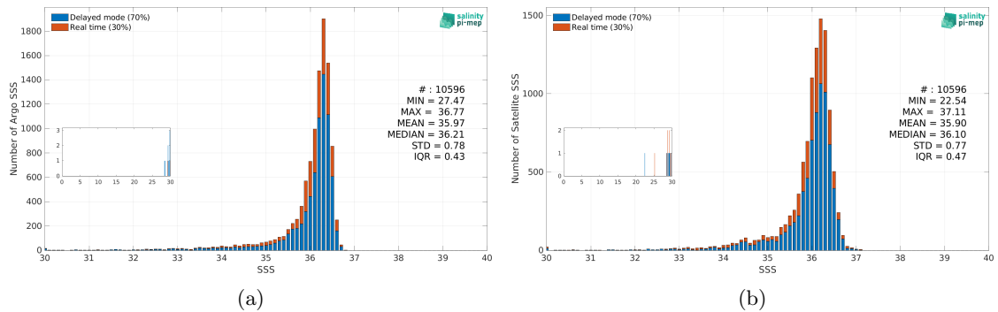
Figure 2: Histograms of SSS from Argo (a) and SMOS SSS L3 v9 - 18 Days (CATDS-CEC-LOCEAN) (b) considering all match-up pairs per bins of 0.1 over the Mississippi river plume Pi-MEP region and for the full satellite product period.
