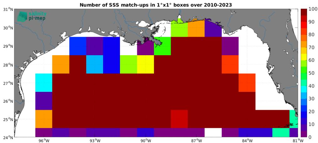
Figure 4: Number of SSS match-ups between Argo SSS and the SMOS SSS L3 v9 - 18 Days (CATDS-CEC-LOCEAN) SSS product for the Mississippi river plume Pi-MEP region over 1^\circ \times 1^\circ boxes and for the full satellite product period.
