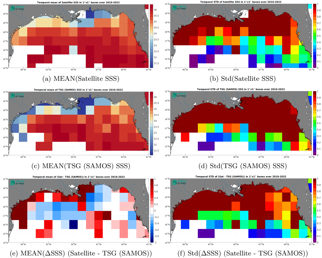
Figure 6: Temporal mean (left) and Std (right) of SSS from SMOS SSS L3 v8 - 9 Days (CATDS-CEC-LOCEAN) (top), TSG (SAMOS) (middle), and of \Delta\text{SSS} (Satellite - TSG (SAMOS)). Only match-up pairs are used to generate these maps.
