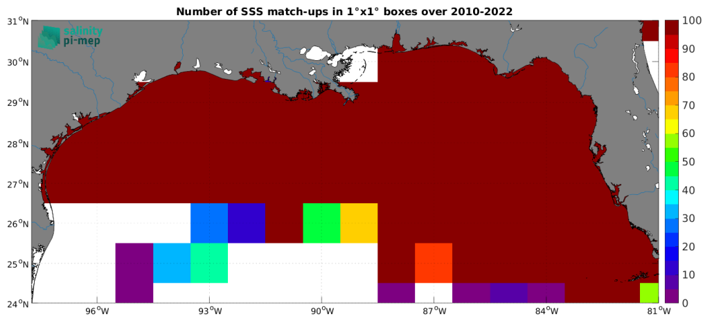
Figure 4: Number of SSS match-ups between TSG (SAMOS) SSS and the SMOS SSS L3 v8 - 9 Days (CATDS-CEC-LOCEAN) SSS product for the Mississippi river plume Pi-MEP region over 1^\circ \times 1^\circ boxes and for the full satellite product period.
