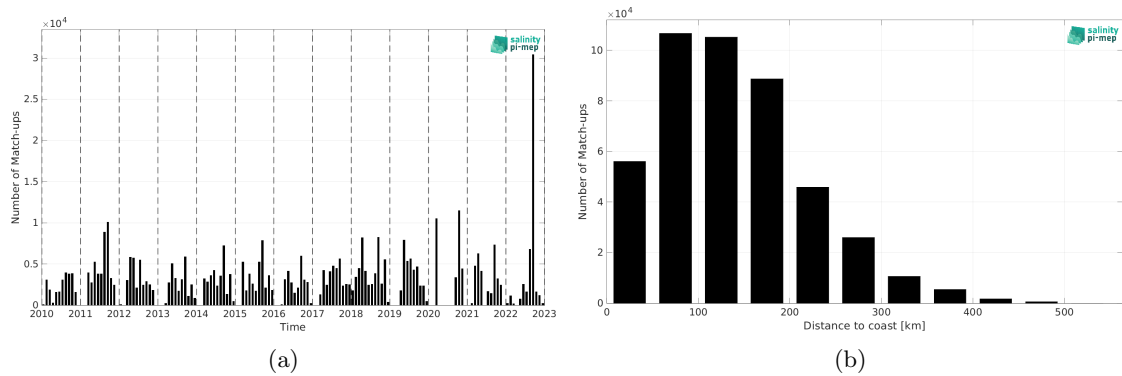
Figure 1: Number of match-ups between TSG (SAMOS) and SMOS SSS L3 v8 - 9 Days (CATDS-CEC-LOCEAN) SSS as a function of time (a) and as function of the distance to coast (b) over the Mississippi river plume Pi-MEP region and for the full satellite product period.
