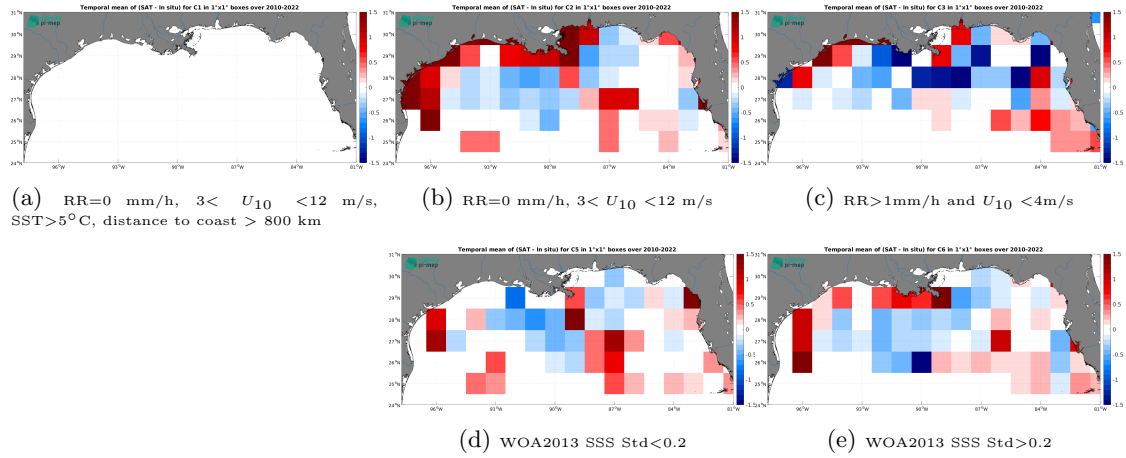
Figure 12: Temporal mean gridded over spatial boxes of size 1^{\circ}\times 1^{\circ} of \Delta\text{SSS} (SMOS SSS L3 v8 - 9 Days (CATDS-CEC-LOCEAN) - TSG (SAMOS)) for 5 different subdatasets corresponding to:RR=0 mm/h, 3 < U_{10} < 12 m/s, SST >5^{\circ}\text{C} , distance to coast > 800 km (a), RR=0 mm/h, 3 < U_{10} < 12 m/s (b), RR >1 mm/h and U_{10} < 4 m/s (c), WOA2013 SSS Std <0.2 (d), WOA2013 SSS Std >0.2 (e).
