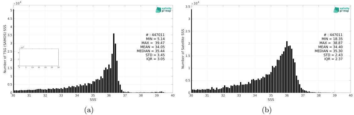
Figure 2: Histograms of SSS from TSG (SAMOS) (a) and SMOS SSS L3 v8 - 9 Days (CATDS-CEC-LOCEAN) (b) considering all match-up pairs per bins of 0.1 over the Mississippi river plume Pi-MEP region and for the full satellite product period.
