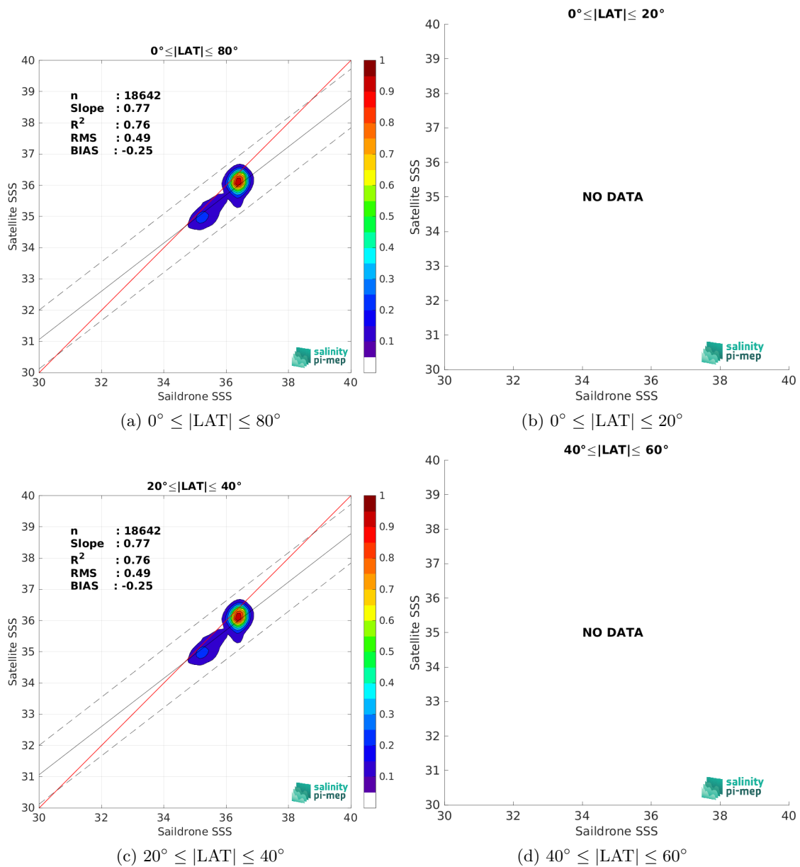
Figure 9: Contour maps of the concentration of SMOS SSS L3 v8 - 9 Days (CATDS-CEC-LOCEAN) SSS (y-axis) versus Saïdrone SSS (x-axis) at match-up pairs for different latitude bands. For each plot, the red line shows x=y . The black thin and dashed lines indicate a linear fit through the data cloud and the \pm 95\% confidence levels, respectively. The number match-up pairs n , the slope and R^2 coefficient of the linear fit, the root mean square (RMS) and the mean bias between satellite and in situ data are indicated for each latitude band in each plots.
