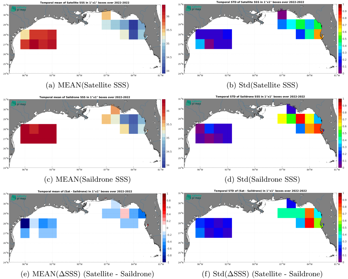
Figure 6: Temporal mean (left) and Std (right) of SSS from SMOS SSS L3 v8 - 9 Days (CATDS-CEC-LOCEAN) (top), Sairdrone (middle), and of \Delta SSS (Satellite - Sairdrone). Only match-up pairs are used to generate these maps.
