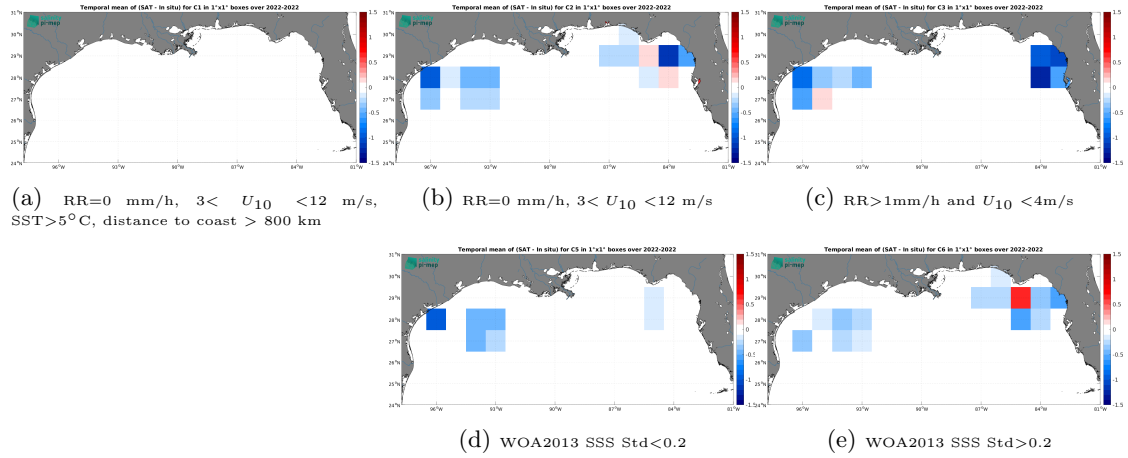
Figure 12: Temporal mean gridded over spatial boxes of size 1^{\circ}\times 1^{\circ} of \Delta\text{SSS} (SMOS SSS L3 v8 - 9 Days (CATDS-CEC-LOCEAN) - Saildrone) for 5 different subdatasets corresponding to:RR=0 mm/h, 3 < U_{10} < 12 m/s, SST >5^{\circ}\text{C} , distance to coast > 800 km (a), RR=0 mm/h, 3 < U_{10} < 12 m/s (b), RR >1 mm/h and U_{10} < 4 m/s (c), WOA2013 SSS Std <0.2 (d), WOA2013 SSS Std >0.2 (e).
