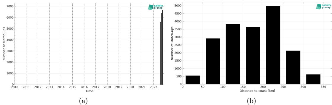
Figure 1: Number of match-ups between Saildrone and SMOS SSS L3 v8 - 9 Days (CATDS-CEC-LOCEAN) SSS as a function of time (a) and as function of the distance to coast (b) over the Mississippi river plume Pi-MEP region and for the full satellite product period.
