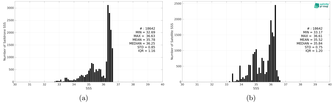
Figure 2: Histograms of SSS from Saildrone (a) and SMOS SSS L3 v8 - 9 Days (CATDS-CEC-LOCEAN) (b) considering all match-up pairs per bins of 0.1 over the Mississippi river plume Pi-MEP region and for the full satellite product period.
