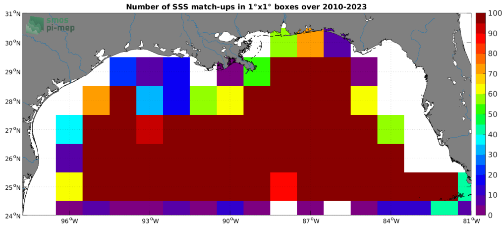
Figure 4: Number of SSS match-ups between Argo SSS and the SMOS SSS L3 v8 - 9 Days (CATDS-CECOS-LOCEAN) SSS product for the Mississippi river plume Pi-MEP region over 1^{\circ} \times 1^{\circ} boxes and for the full satellite product period.
