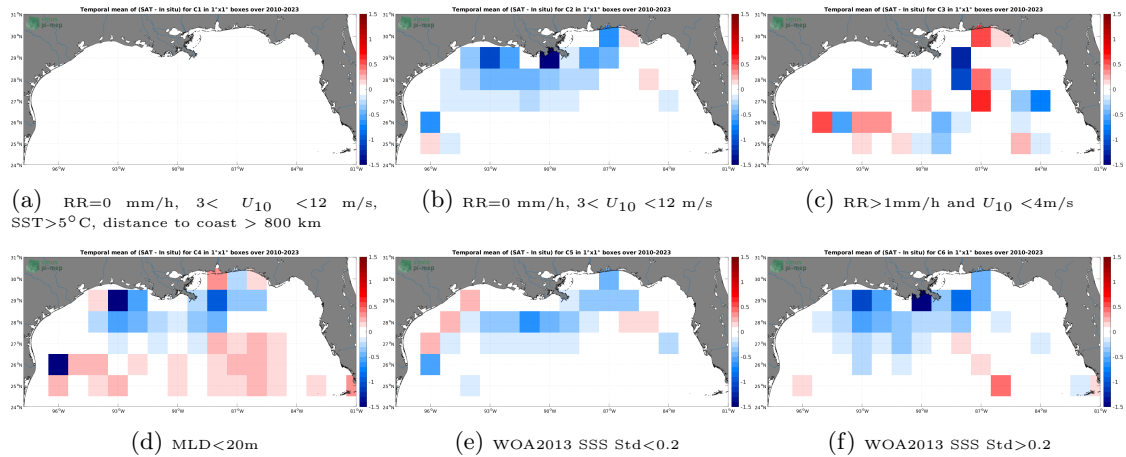
Figure 12: Temporal mean gridded over spatial boxes of size 1^{\circ}\times 1^{\circ} of \Delta\text{SSS} (SMOS SSS L3 v8 - 9 Days (CATDS-CECOS-LOCEAN) - Argo) for 6 different subdatasets corresponding to:RR=0 mm/h, 3 < U_{10} < 12 m/s, SST > 5^{\circ}\text{C} , distance to coast > 800 km (a), RR=0 mm/h, 3 < U_{10} < 12 m/s (b), RR > 1 mm/h and U_{10} < 4 m/s (c),MLD < 20\text{m} (d),WOA2013 SSS Std < 0.2 (e),WOA2013 SSS Std > 0.2 (f).
