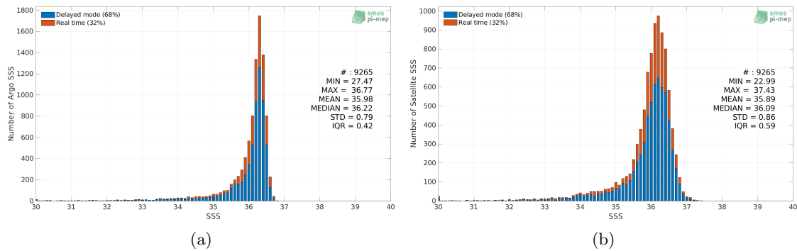
Figure 2: Histograms of SSS from Argo (a) and SMOS SSS L3 v8 - 9 Days (CATDS-CECOS-LOCEAN) (b) considering all match-up pairs per bins of 0.1 over the Mississippi river plume Pi-MEP region and for the full satellite product period.
