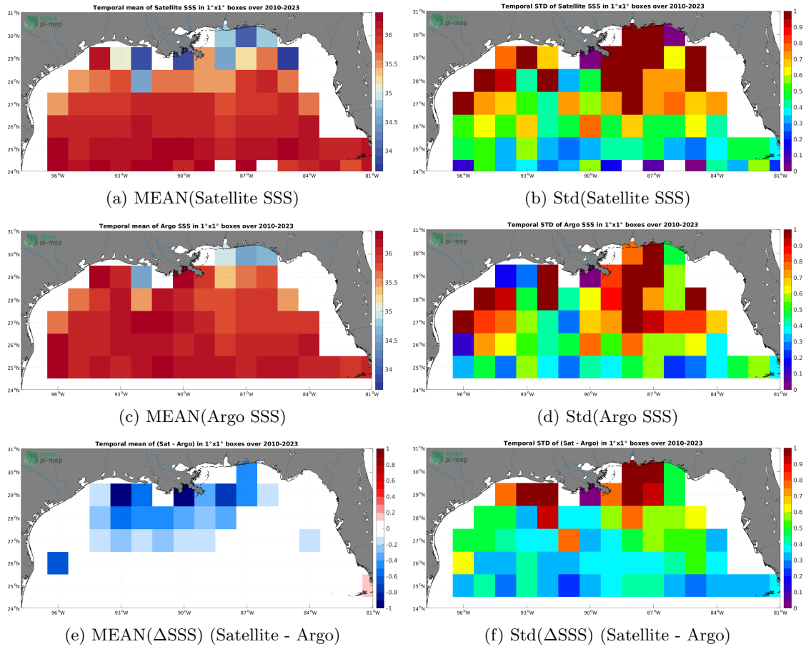
Figure 6: Temporal mean (left) and Std (right) of SSS from SMOS SSS L3 v8 - 9 Days (CATDS-CECOS-LOCEAN) (top), Argo (middle), and of \Delta SSS (Satellite - Argo). Only match-up pairs are used to generate these maps.
