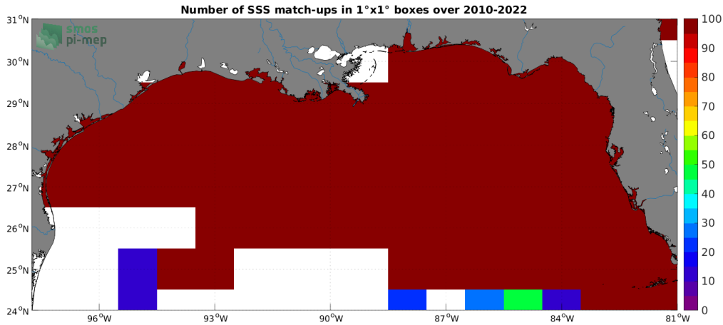
Figure 4: Number of SSS match-ups between TSG (SAMOS) SSS and the SMOS SSS L3 v8 - 18 Days (CATDS-CECOS-LOCEAN) SSS product for the Mississippi river plume Pi-MEP region over 1^\circ \times 1^\circ boxes and for the full satellite product period.
