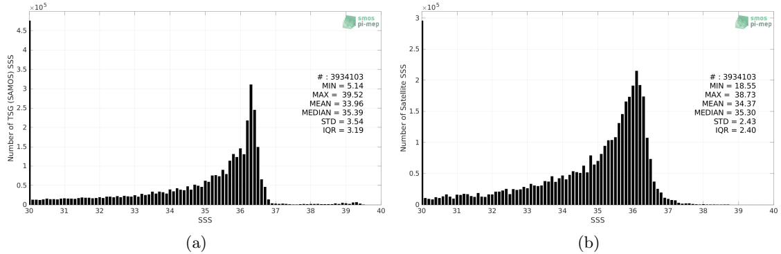
Figure 2: Histograms of SSS from TSG (SAMOS) (a) and SMOS SSS L3 v8 - 18 Days (CATDS-CECOS-LOCEAN) (b) considering all match-up pairs per bins of 0.1 over the Mississippi river plume Pi-MEP region and for the full satellite product period.
