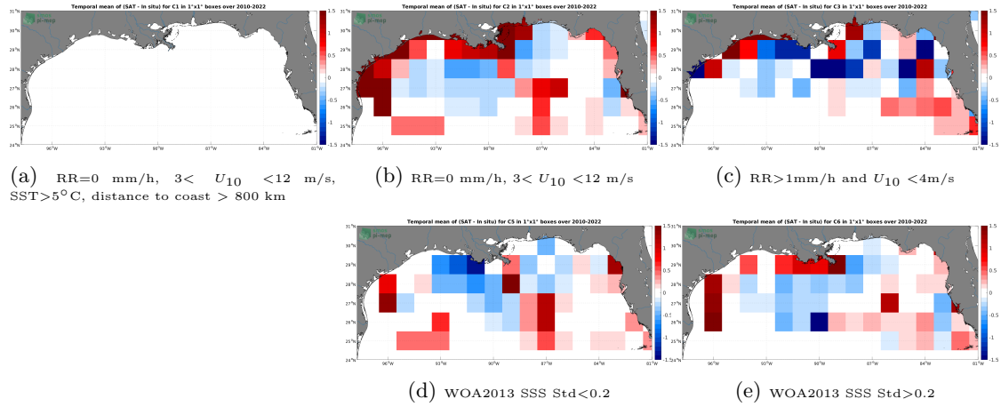
Figure 12: Temporal mean gridded over spatial boxes of size 1^{\circ}\times 1^{\circ} of \Delta\text{SSS} (SMOS SSS L3 v8 - 18 Days (CATDS-CECOS-LOCEAN) - TSG (SAMOS)) for 5 different subdatasets corresponding to:RR=0 mm/h, 3 < U_{10} < 12 m/s, SST >5^{\circ}\text{C} , distance to coast > 800 km (a), RR=0 mm/h, 3 < U_{10} < 12 m/s (b), RR >1 mm/h and U_{10} < 4 m/s (c), WOA2013 SSS Std <0.2 (d), WOA2013 SSS Std >0.2 (e).
