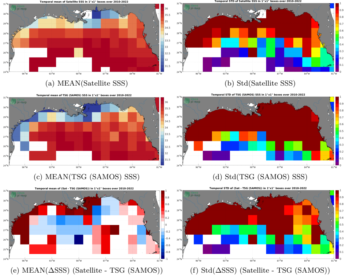
Figure 6: Temporal mean (left) and Std (right) of SSS from SMOS SSS L3 v8 - 18 Days (CATDS-CECOS-LOCEAN) (top), TSG (SAMOS) (middle), and of \Delta\text{SSS} (Satellite - TSG (SAMOS)). Only match-up pairs are used to generate these maps.
