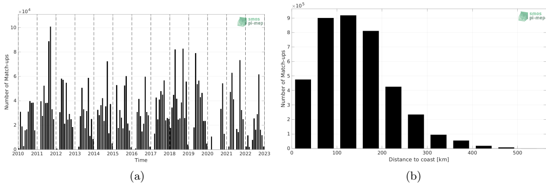
Figure 1: Number of match-ups between TSG (SAMOS) and SMOS SSS L3 v8 - 18 Days (CATDS-CECOS-LOCEAN) SSS as a function of time (a) and as function of the distance to coast (b) over the Mississippi river plume Pi-MEP region and for the full satellite product period.
