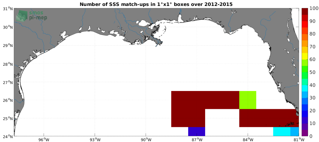
Figure 4: Number of SSS match-ups between TSG (GOSUD-Sailing-ship) SSS and the SMOS SSS L3 v8 - 18 Days (CATDS-CECOS-LOCEAN) SSS product for the Mississippi river plume Pi-MEP region over 1^\circ \times 1^\circ boxes and for the full satellite product period.
