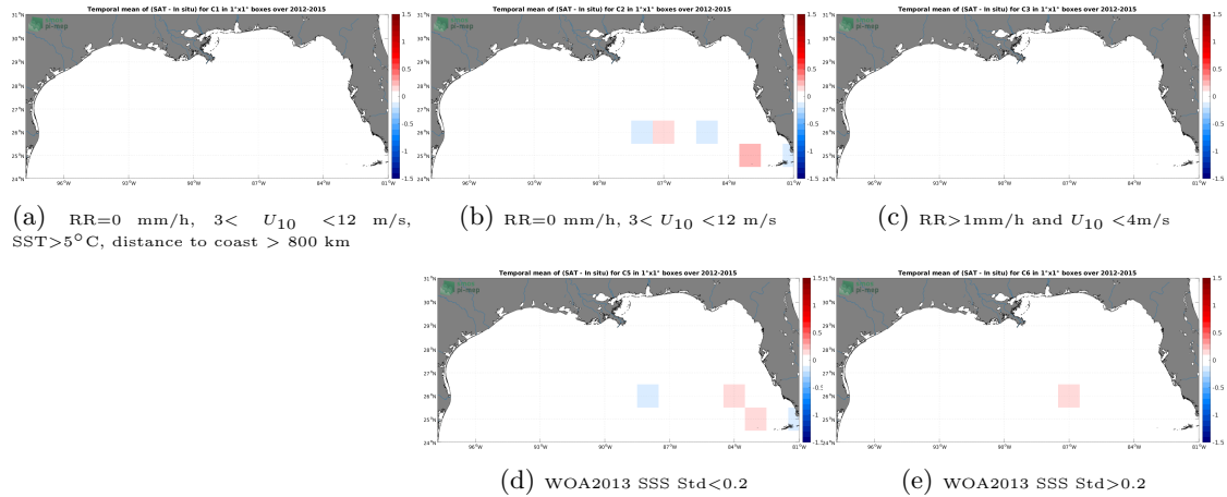
Figure 12: Temporal mean gridded over spatial boxes of size 1^{\circ}\times 1^{\circ} of \Delta SSS (SMOS SSS L3 v8 - 18 Days (CATDS-CECOS-LOCEAN) - TSG (GOSUD-Sailing-ship)) for 5 different subdatasets corresponding to:RR=0 mm/h, 3 < U_{10} < 12 m/s, SST >5^{\circ}\text{C} , distance to coast > 800 km (a), RR=0 mm/h, 3 < U_{10} < 12 m/s (b), RR >1 mm/h and U_{10} < 4 m/s (c), WOA2013 SSS Std <0.2 (d), WOA2013 SSS Std >0.2 (e).
