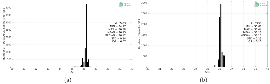
Figure 2: Histograms of SSS from TSG (GOSUD-Sailing-ship) (a) and SMOS SSS L3 v8 - 18 Days (CATDS-CECOS-LOCEAN) (b) considering all match-up pairs per bins of 0.1 over the Mississippi river plume Pi-MEP region and for the full satellite product period.
