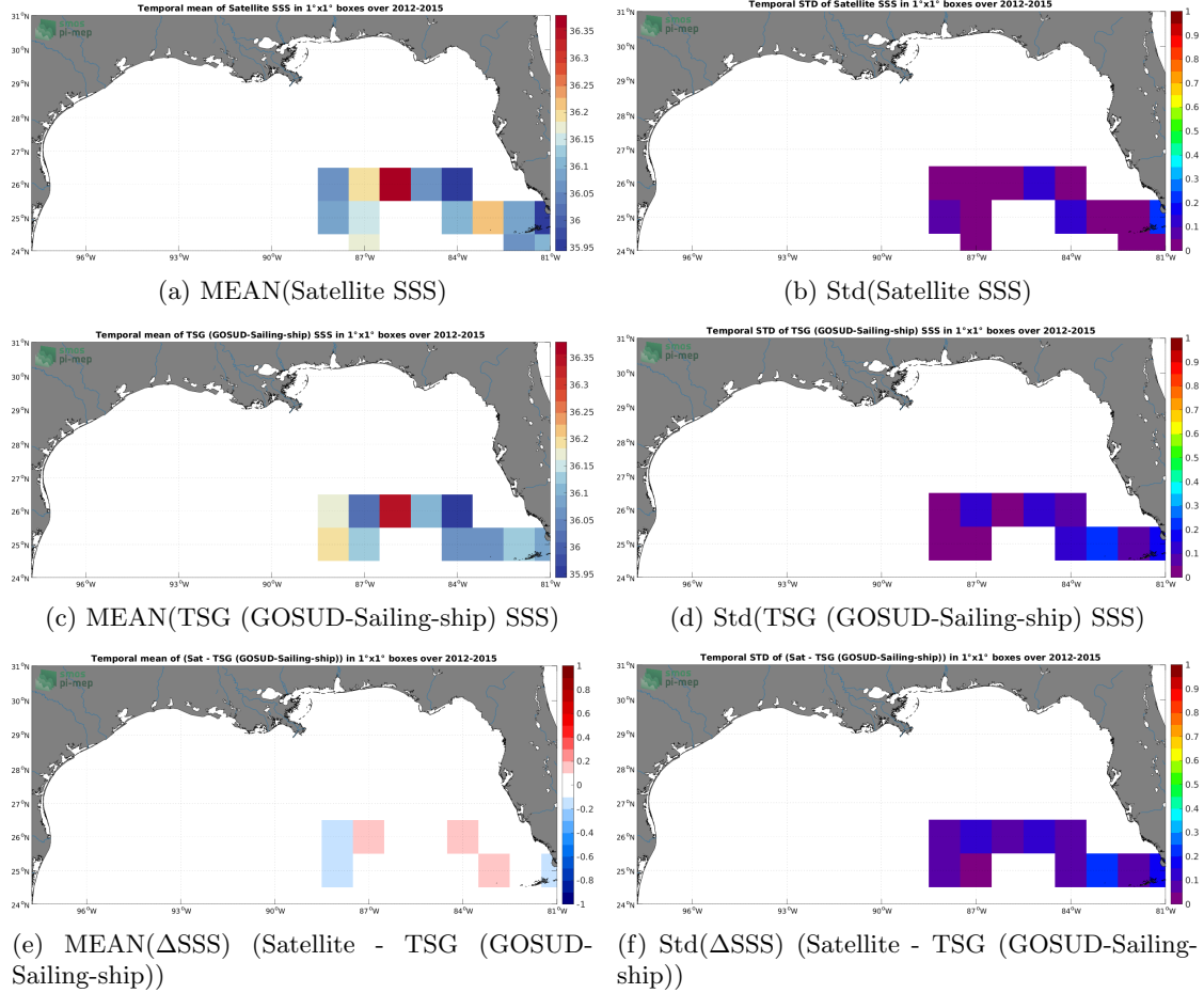
Figure 6: Temporal mean (left) and Std (right) of SSS from SMOS SSS L3 v8 - 18 Days (CATDS-CECOS-LOCEAN) (top), TSG (GOSUD-Sailing-ship) (middle), and of \Delta\text{SSS} (Satellite - TSG (GOSUD-Sailing-ship)). Only match-up pairs are used to generate these maps.
