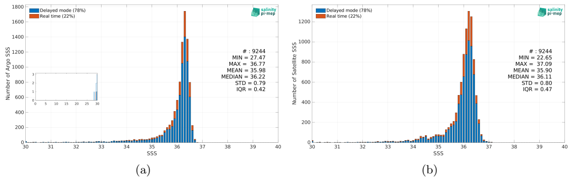
Figure 2: Histograms of SSS from Argo (a) and SMOS SSS L3 v8 - 18 Days (CATDS-CEC-LOCEAN) (b) considering all match-up pairs per bins of 0.1 over the Mississippi river plume Pi-MEP region and for the full satellite product period.
