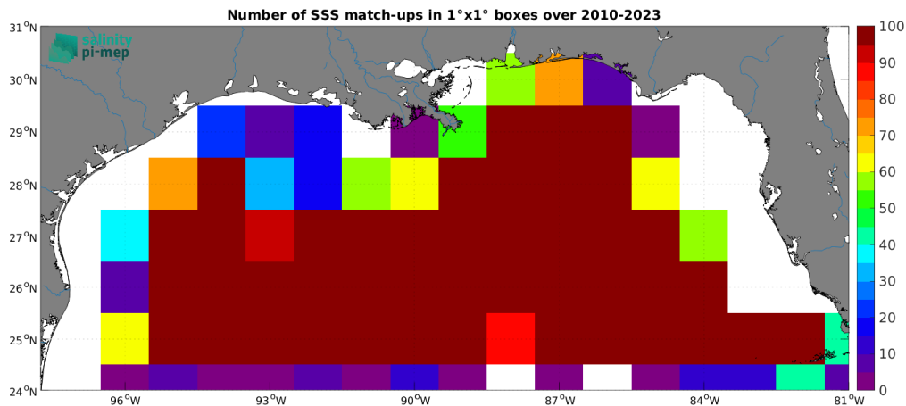
Figure 4: Number of SSS match-ups between Argo SSS and the SMOS SSS L3 v8 - 18 Days (CATDS-CEC-LOCEAN) SSS product for the Mississippi river plume Pi-MEP region over 1^\circ \times 1^\circ boxes and for the full satellite product period.
