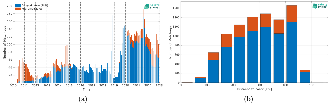
Figure 1: Number of match-ups between Argo and SMOS SSS L3 v8 - 18 Days (CATDS-CEC-LOCEAN) SSS as a function of time (a) and as function of the distance to coast (b) over the Mississippi river plume Pi-MEP region and for the full satellite product period.
