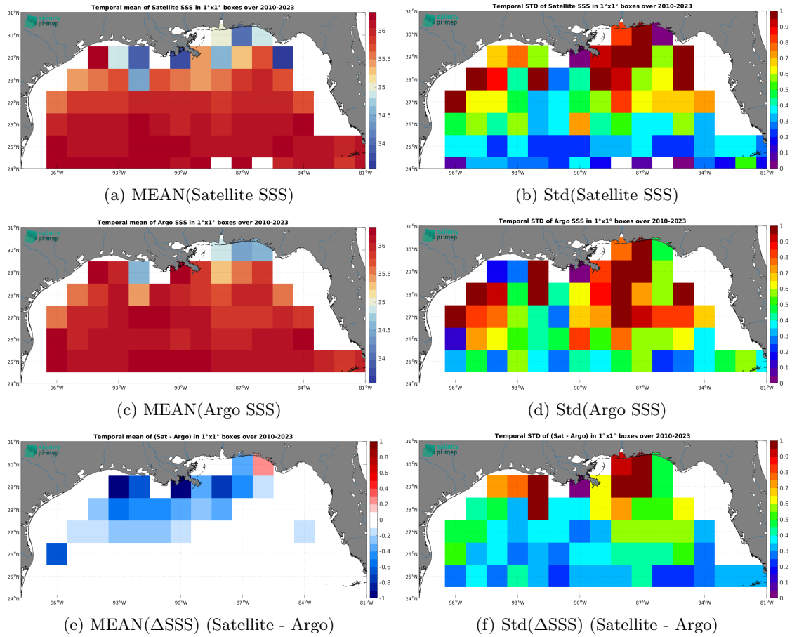
Figure 6: Temporal mean (left) and Std (right) of SSS from SMOS SSS L3 v8 - 18 Days (CATDS-CEC-LOCEAN) (top), Argo (middle), and of \Delta SSS (Satellite - Argo). Only match-up pairs are used to generate these maps.
