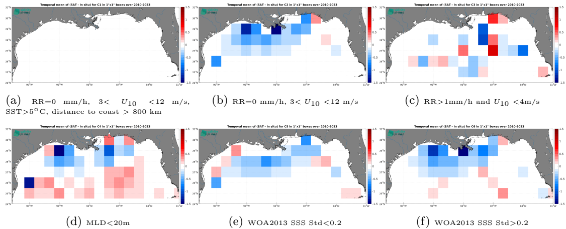
Figure 12: Temporal mean gridded over spatial boxes of size 1^{\circ}\times 1^{\circ} of \Delta\text{SSS} (SMOS SSS L3 v8 - 18 Days (CATDS-CEC-LOCEAN) - Argo) for 6 different subdatasets corresponding to:RR=0 mm/h, 3 < U_{10} < 12 m/s, SST > 5^{\circ}\text{C} , distance to coast > 800 km (a), RR=0 mm/h, 3 < U_{10} < 12 m/s (b), RR > 1\text{mm/h} and U_{10} < 4\text{m/s} (c),MLD < 20\text{m} (d),WOA2013 SSS Std < 0.2 (e),WOA2013 SSS Std > 0.2 (f).
