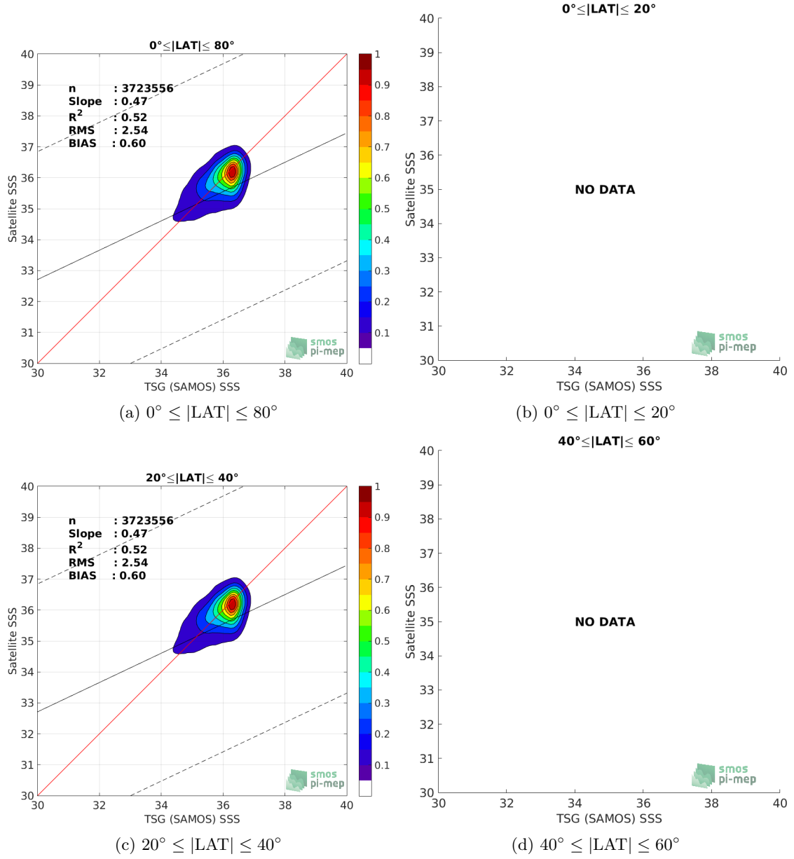
Figure 9: Contour maps of the concentration of SMOS SSS L3 v7 - 9 Days (CATDS-CECOS-LOCEAN) SSS (y-axis) versus TSG (SAMOS) SSS (x-axis) at match-up pairs for different latitude bands. For each plot, the red line shows x=y . The black thin and dashed lines indicate a linear fit through the data cloud and the \pm 95\% confidence levels, respectively. The number match-up pairs n , the slope and R^2 coefficient of the linear fit, the root mean square (RMS) and the mean bias between satellite and in situ data are indicated for each latitude band in each plots.
