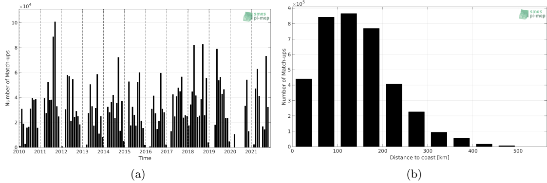
Figure 1: Number of match-ups between TSG (SAMOS) and SMOS SSS L3 v7 - 9 Days (CATDS-CECOS-LOCEAN) SSS as a function of time (a) and as function of the distance to coast (b) over the Mississippi river plume Pi-MEP region and for the full satellite product period.
