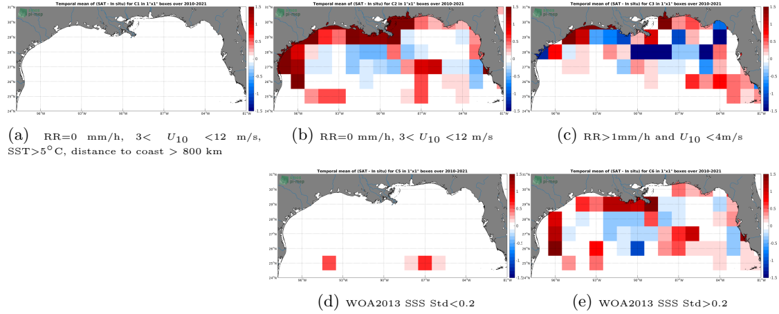
Figure 12: Temporal mean gridded over spatial boxes of size 1^{\circ}\times 1^{\circ} of \Delta\text{SSS} (SMOS SSS L3 v7 - 9 Days (CATDS-CECOS-LOCEAN) - TSG (SAMOS)) for 5 different subdatasets corresponding to: RR=0 mm/h, 3 < U_{10} < 12 m/s, SST >5^{\circ}\text{C} , distance to coast > 800 km (a), RR=0 mm/h, 3 < U_{10} < 12 m/s (b), RR >1 mm/h and U_{10} < 4 m/s (c), WOA2013 SSS Std <0.2 (d), WOA2013 SSS Std >0.2 (e).
