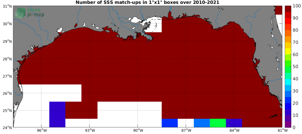
Figure 4: Number of SSS match-ups between TSG (SAMOS) SSS and the SMOS SSS L3 v7 - 9 Days (CATDS-CECOS-LOCEAN) SSS product for the Mississippi river plume Pi-MEP region over 1^\circ \times 1^\circ boxes and for the full satellite product period.
