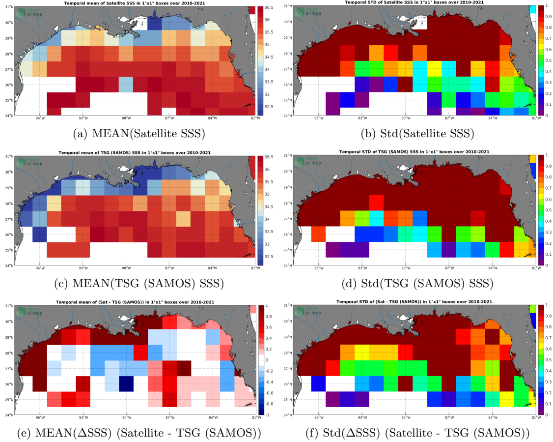
Figure 6: Temporal mean (left) and Std (right) of SSS from SMOS SSS L3 v7 - 9 Days (CATDS-CECOS-LOCEAN) (top), TSG (SAMOS) (middle), and of \Delta\text{SSS} (Satellite - TSG (SAMOS)). Only match-up pairs are used to generate these maps.
