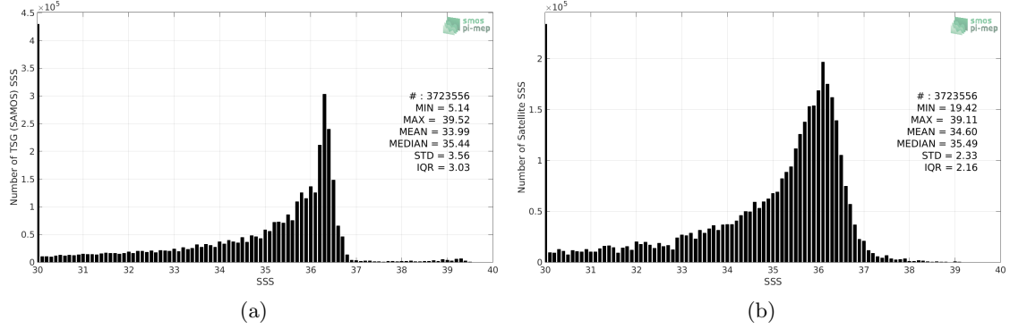
Figure 2: Histograms of SSS from TSG (SAMOS) (a) and SMOS SSS L3 v7 - 9 Days (CATDS-CECOS-LOCEAN) (b) considering all match-up pairs per bins of 0.1 over the Mississippi river plume Pi-MEP region and for the full satellite product period.
