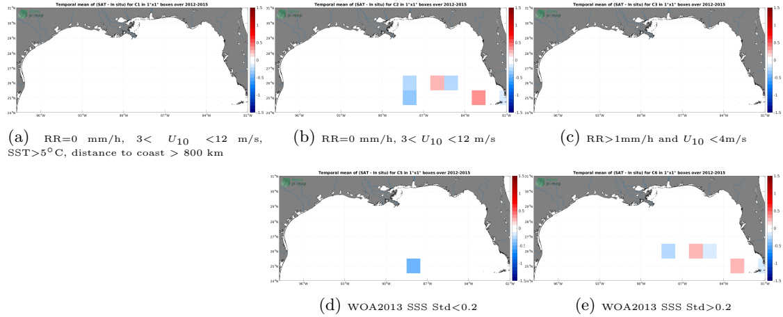
Figure 12: Temporal mean gridded over spatial boxes of size 1^{\circ}\times 1^{\circ} of \Delta SSS (SMOS SSS L3 v7 - 9 Days (CATDS-CECOS-LOCEAN) - TSG (GOSUD-Sailing-ship)) for 5 different subdatasets corresponding to:RR=0 mm/h, 3 < U_{10} < 12 m/s, SST >5^{\circ}\text{C} , distance to coast > 800 km (a), RR=0 mm/h, 3 < U_{10} < 12 m/s (b), RR >1 mm/h and U_{10} < 4 m/s (c), WOA2013 SSS Std <0.2 (d), WOA2013 SSS Std >0.2 (e).
