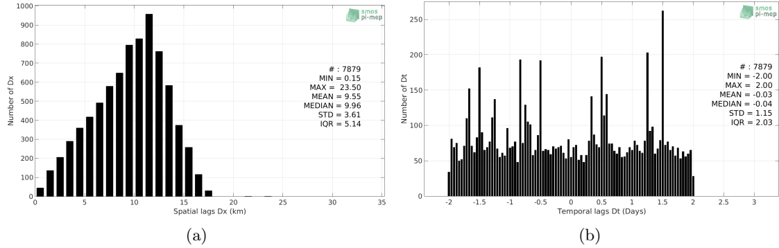
Figure 5: Histograms of the spatial (a) and temporal (b) lags between the location/time of the Argo measurement and the date of the corresponding SMOS SSS L3 v7 - 9 Days (CATDS-CECOS-LOCEAN) SSS pixel.
