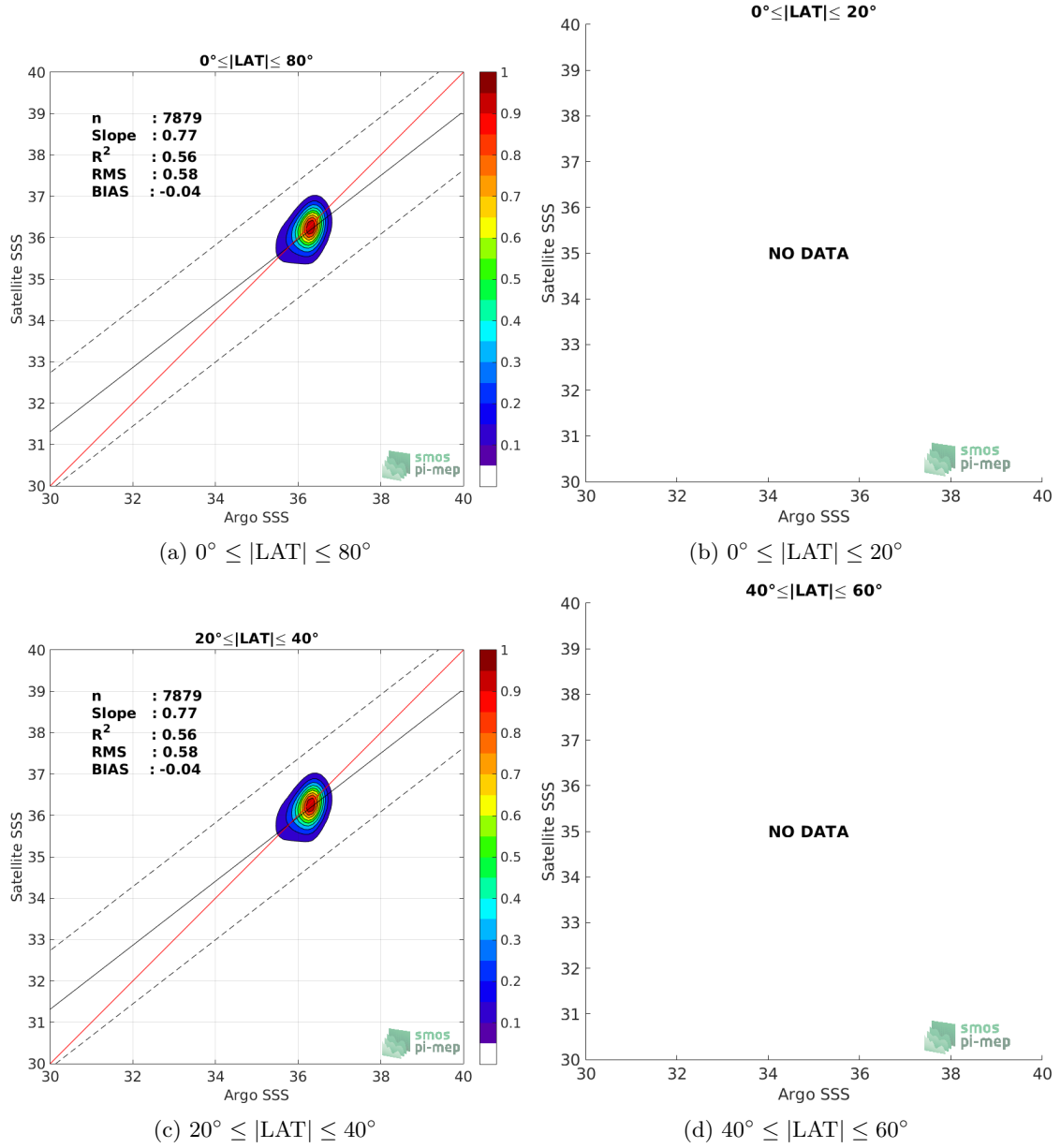
Figure 9: Contour maps of the concentration of SMOS SSS L3 v7 - 9 Days (CATDS-CECOS-LOCEAN) SSS (y-axis) versus Argo SSS (x-axis) at match-up pairs for different latitude bands. For each plot, the red line shows x=y . The black thin and dashed lines indicate a linear fit through the data cloud and the \pm 95\% confidence levels, respectively. The number match-up pairs n , the slope and R^2 coefficient of the linear fit, the root mean square (RMS) and the mean bias between satellite and in situ data are indicated for each latitude band in each plots.
