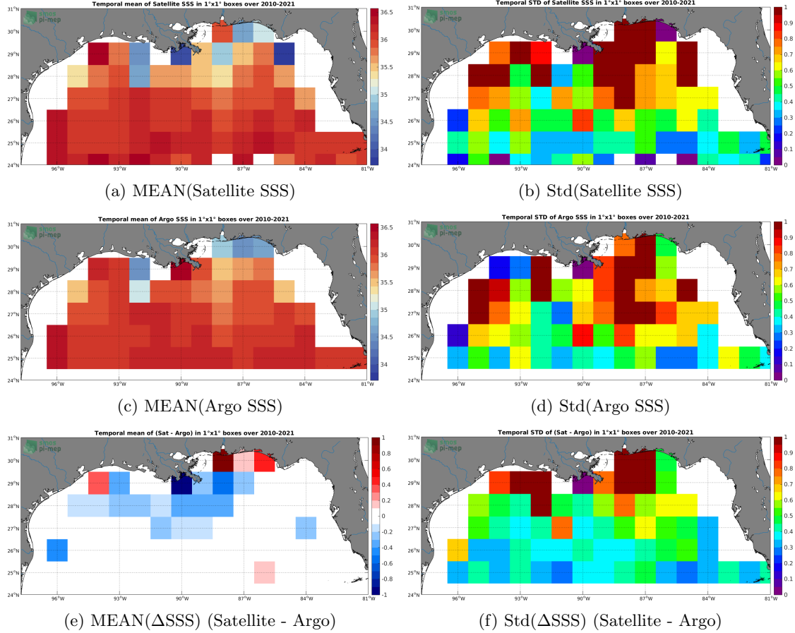
Figure 6: Temporal mean (left) and Std (right) of SSS from SMOS SSS L3 v7 - 9 Days (CATDS-CECOS-LOCEAN) (top), Argo (middle), and of \Delta\text{SSS} (Satellite - Argo). Only match-up pairs are used to generate these maps.
