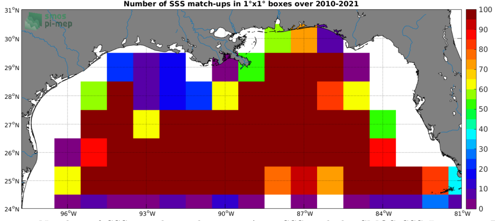
Figure 4: Number of SSS match-ups between Argo SSS and the SMOS SSS L3 v7 - 9 Days (CATDS-CECOS-LOCEAN) SSS product for the Mississippi river plume Pi-MEP region over 1^\circ \times 1^\circ boxes and for the full satellite product period.
