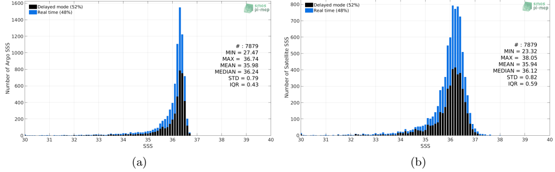
Figure 2: Histograms of SSS from Argo (a) and SMOS SSS L3 v7 - 9 Days (CATDS-CECOS-LOCEAN) (b) considering all match-up pairs per bins of 0.1 over the Mississippi river plume Pi-MEP region and for the full satellite product period.
