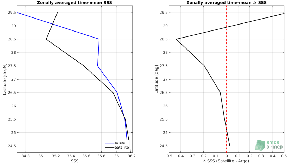
Figure 8: Left panel: Zonal mean SSS from SMOS SSS L3 v7 - 9 Days (CATDS-CECOS-LOCEAN) satellite product (black) and from Argo (blue). Right panel: Zonal mean of \Delta SSS (Satellite - Argo) for all the collected Pi-MEP match-up pairs estimated over the full satellite product period.
