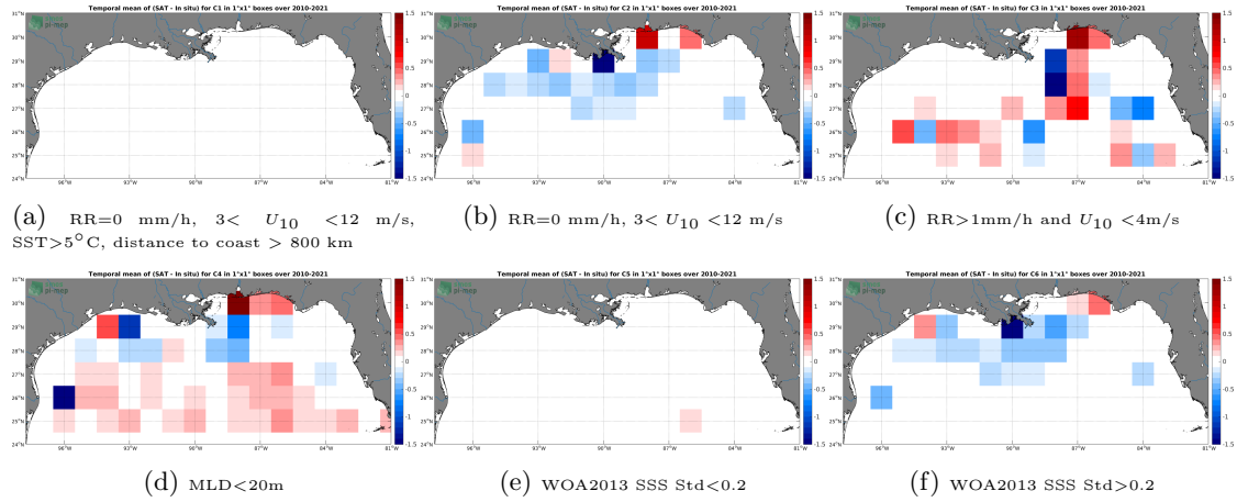
Figure 12: Temporal mean gridded over spatial boxes of size 1^{\circ} \times 1^{\circ} of \Delta\text{SSS} (SMOS SSS L3 v7 - 9 Days (CATDS-CECOS-LOCEAN) - Argo) for 6 different subdatasets corresponding to: \text{RR}=0 mm/h, 3 < U_{10} < 12 m/s, \text{SST} > 5^{\circ}\text{C} , distance to coast > 800 km (a), \text{RR}=0 mm/h, 3 < U_{10} < 12 m/s (b), \text{RR} > 1 mm/h and U_{10} < 4 m/s (c), \text{MLD} < 20\text{m} (d), WOA2013 SSS Std < 0.2 (e), WOA2013 SSS Std > 0.2 (f).
