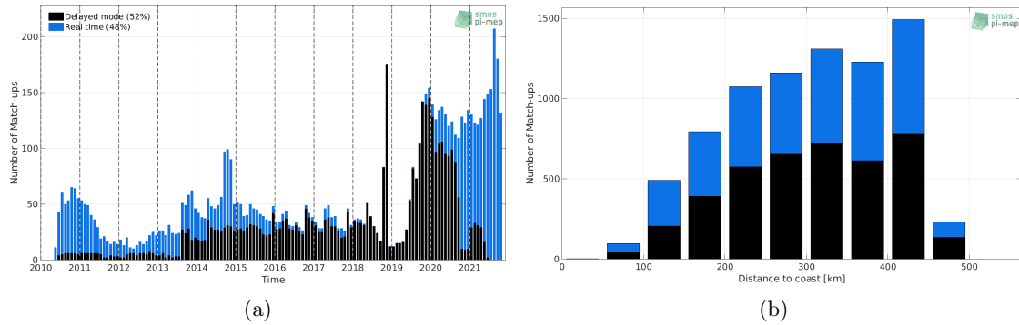
Figure 1: Number of match-ups between Argo and SMOS SSS L3 v7 - 9 Days (CATDS-CECOS-LOCEAN) SSS as a function of time (a) and as function of the distance to coast (b) over the Mississippi river plume Pi-MEP region and for the full satellite product period.
