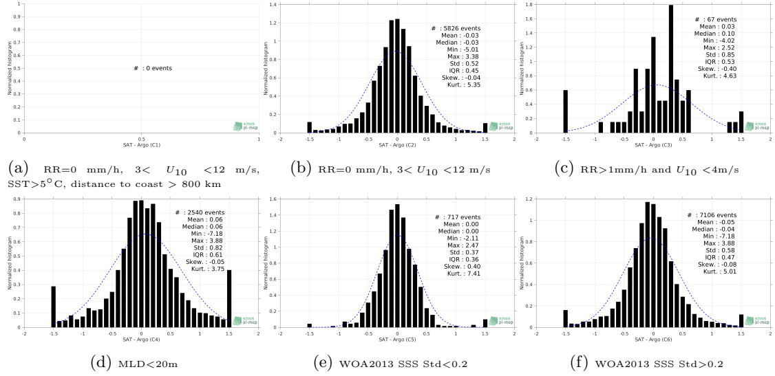
Figure 13: Normalized histogram of \Delta SSS (SMOS SSS L3 v7 - 9 Days (CATDS-CECOS-LOCEAN) - Argo) for 6 different subdatasets corresponding to: RR=0 mm/h, 3 < U_{10} < 12 m/s, SST>5°C, distance to coast > 800 km (a), RR=0 mm/h, 3 < U_{10} < 12 m/s (b), RR>1mm/h and U_{10} < 4 m/s (c), MLD<20m (d), WOA2013 SSS Std<0.2 (e), WOA2013 SSS Std>0.2 (f).
