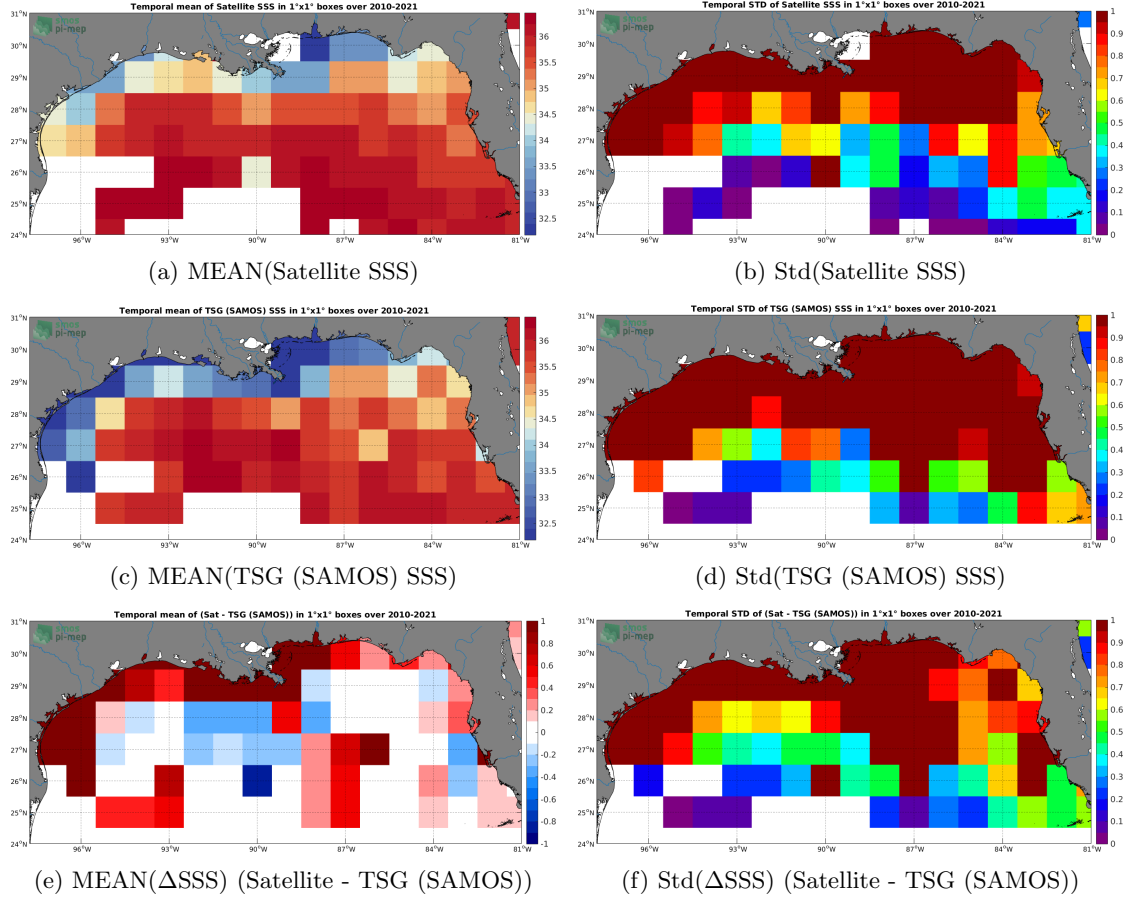
Figure 6: Temporal mean (left) and Std (right) of SSS from SMOS SSS L3 v7 - 18 Days (CATDS-CECOS-LOCEAN) (top), TSG (SAMOS) (middle), and of \Delta\text{SSS} (Satellite - TSG (SAMOS)). Only match-up pairs are used to generate these maps.
