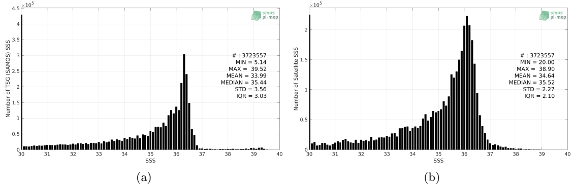
Figure 2: Histograms of SSS from TSG (SAMOS) (a) and SMOS SSS L3 v7 - 18 Days (CATDS-CECOS-LOCEAN) (b) considering all match-up pairs per bins of 0.1 over the Mississippi river plume Pi-MEP region and for the full satellite product period.
