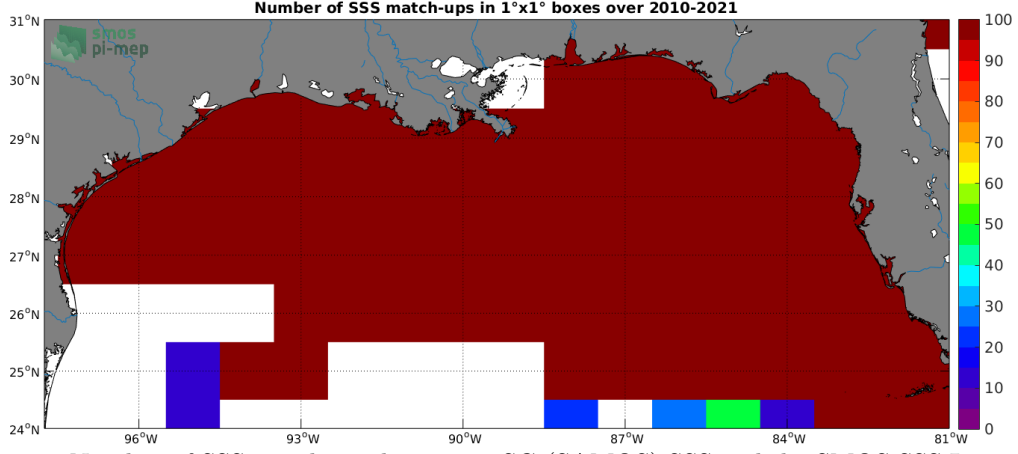
Figure 4: Number of SSS match-ups between TSG (SAMOS) SSS and the SMOS SSS L3 v7 - 18 Days (CATDS-CECOS-LOCEAN) SSS product for the Mississippi river plume Pi-MEP region over 1^\circ \times 1^\circ boxes and for the full satellite product period.
