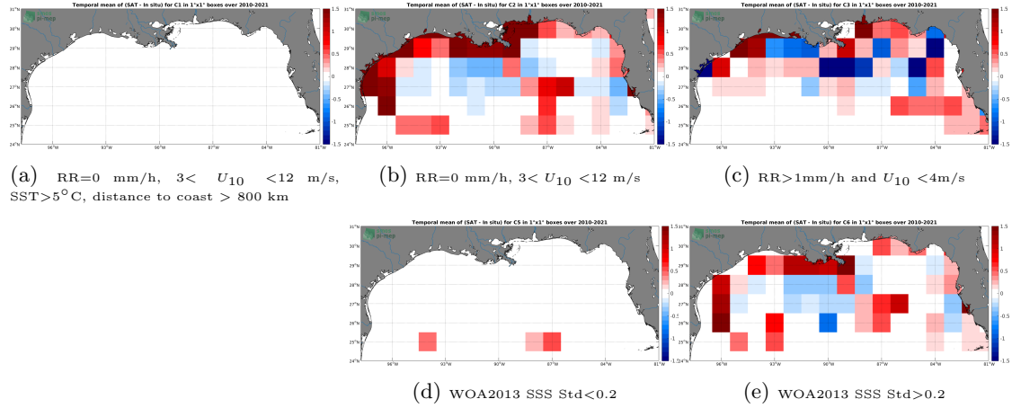
Figure 12: Temporal mean gridded over spatial boxes of size 1^{\circ}\times 1^{\circ} of \Delta\text{SSS} (SMOS SSS L3 v7 - 18 Days (CATDS-CECOS-LOCEAN) - TSG (SAMOS)) for 5 different subdatasets corresponding to: \text{RR}=0 mm/h, 3 < U_{10} < 12 m/s, \text{SST} > 5^{\circ}\text{C} , distance to coast > 800 km (a), \text{RR}=0 mm/h, 3 < U_{10} < 12 m/s (b), \text{RR} > 1 mm/h and U_{10} < 4 m/s (c), WOA2013 SSS Std < 0.2 (d), WOA2013 SSS Std > 0.2 (e).
