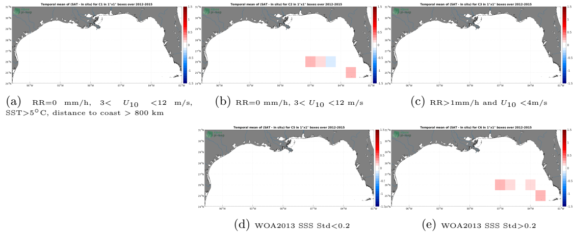
Figure 12: Temporal mean gridded over spatial boxes of size 1^{\circ}\times 1^{\circ} of \Delta SSS (SMOS SSS L3 v7 - 18 Days (CATDS-CECOS-LOCEAN) - TSG (GOSUD-Sailing-ship)) for 5 different subdatasets corresponding to:RR=0 mm/h, 3 < U_{10} < 12 m/s, SST >5^{\circ}\text{C} , distance to coast > 800 km (a), RR=0 mm/h, 3 < U_{10} < 12 m/s (b), RR >1 mm/h and U_{10} < 4 m/s (c), WOA2013 SSS Std <0.2 (d), WOA2013 SSS Std >0.2 (e).
