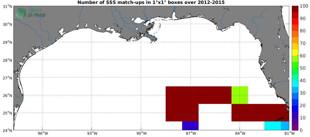
Figure 4: Number of SSS match-ups between TSG (GOSUD-Sailing-ship) SSS and the SMOS SSS L3 v7 - 18 Days (CATDS-CECOS-LOCEAN) SSS product for the Mississippi river plume Pi-MEP region over 1^\circ \times 1^\circ boxes and for the full satellite product period.
