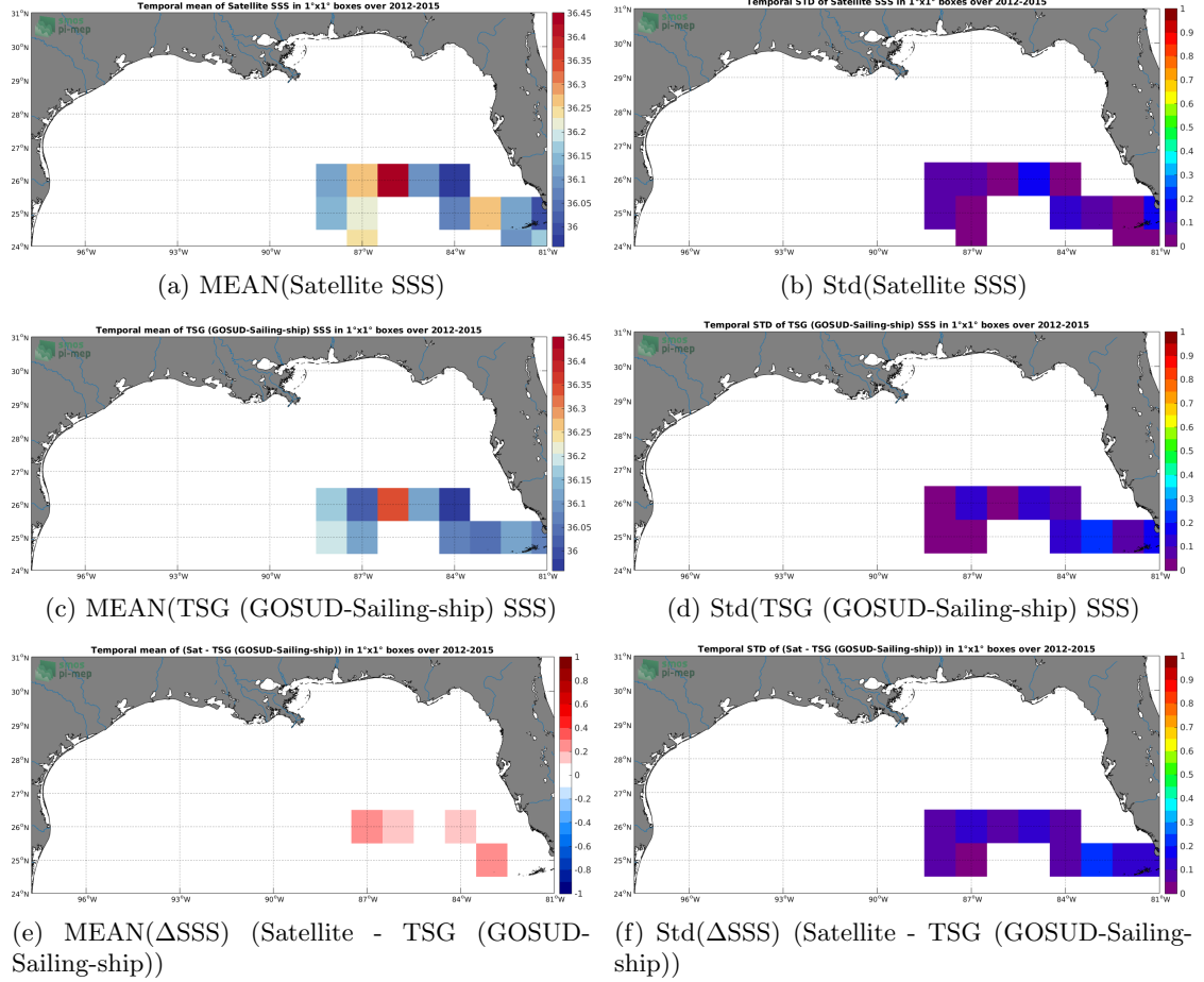
Figure 6: Temporal mean (left) and Std (right) of SSS from SMOS SSS L3 v7 - 18 Days (CATDS-CECOS-LOCEAN) (top), TSG (GOSUD-Sailing-ship) (middle), and of \Delta\text{SSS} (Satellite - TSG (GOSUD-Sailing-ship)). Only match-up pairs are used to generate these maps.
