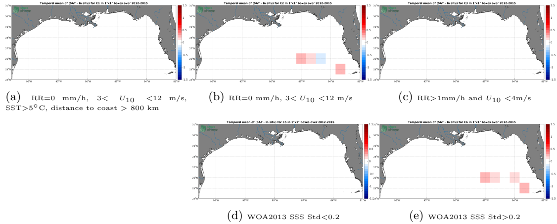
Figure 12: Temporal mean gridded over spatial boxes of size 1^\circ \times 1^\circ of \Delta SSS (SMOS SSS L3 v7 - 18 Days (CATDS-CECOS-LOCEAN) - TSG (GOSUD-Sailing-ship)) for 5 different subdatasets corresponding to:RR=0 mm/h, 3 < U_{10} < 12 m/s, SST >5^\circ\text{C} , distance to coast > 800 km (a), RR=0 mm/h, 3 < U_{10} < 12 m/s (b), RR >1 mm/h and U_{10} < 4 m/s (c), WOA2013 SSS Std <0.2 (d), WOA2013 SSS Std >0.2 (e).
