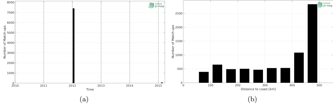
Figure 1: Number of match-ups between TSG (GOSUD-Sailing-ship) and SMOS SSS L3 v7 - 18 Days (CATDS-CECOS-LOCEAN) SSS as a function of time (a) and as function of the distance to coast (b) over the Mississippi river plume Pi-MEP region and for the full satellite product period.
