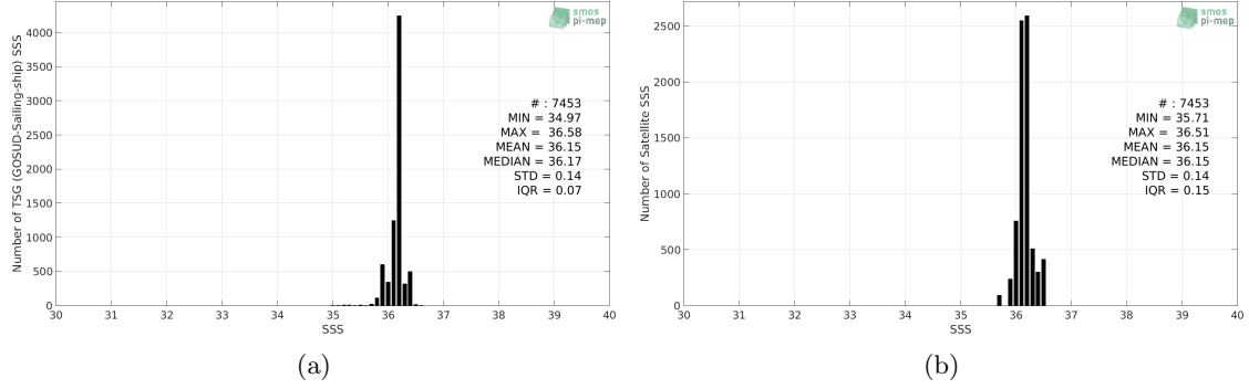
Figure 2: Histograms of SSS from TSG (GOSUD-Sailing-ship) (a) and SMOS SSS L3 v7 - 18 Days (CATDS-CECOS-LOCEAN) (b) considering all match-up pairs per bins of 0.1 over the Mississippi river plume Pi-MEP region and for the full satellite product period.
