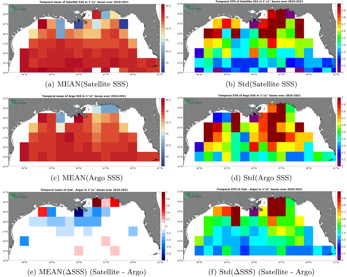
Figure 6: Temporal mean (left) and Std (right) of SSS from SMOS SSS L3 v7 - 18 Days (CATDS-CECOS-LOCEAN) (top), Argo (middle), and of \Delta\text{SSS} (Satellite - Argo). Only match-up pairs are used to generate these maps.
