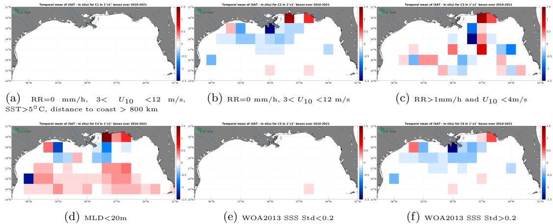
Figure 12: Temporal mean gridded over spatial boxes of size 1^{\circ}\times 1^{\circ} of \Delta\text{SSS} (SMOS SSS L3 v7 - 18 Days (CATDS-CECOS-LOCEAN) - Argo) for 6 different subdatasets corresponding to:RR=0 mm/h, 3 < U_{10} < 12 m/s, SST > 5^{\circ}\text{C} , distance to coast > 800 km (a), RR=0 mm/h, 3 < U_{10} < 12 m/s (b), RR > 1\text{mm/h} and U_{10} < 4\text{m/s} (c),MLD < 20\text{m} (d),WOA2013 SSS Std < 0.2 (e),WOA2013 SSS Std > 0.2 (f).
